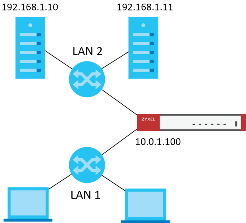
Figure 316 Virtual Server on the LAN - Example 2
