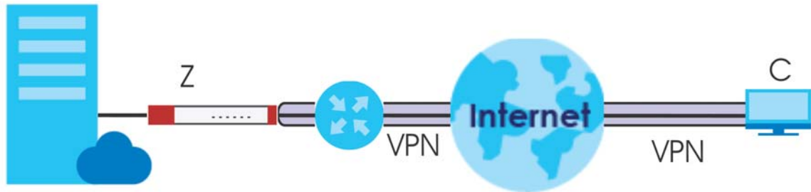
Figure 387 L2TP and Zyxel Device Behind a NAT Router
