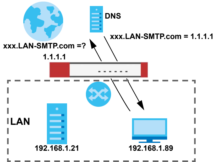
Figure 312 LAN Computer Queries a Public DNS Server
