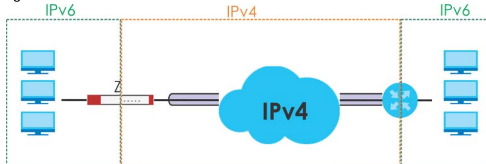
Figure 265 IPv6-in-IPv4 Tunnel
