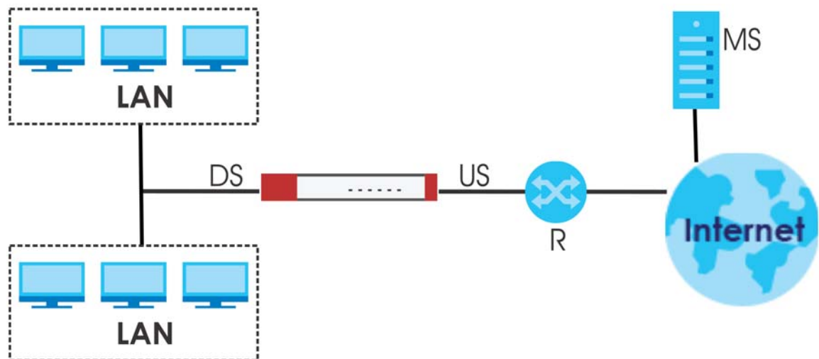
Figure 248 IGMP Proxy
