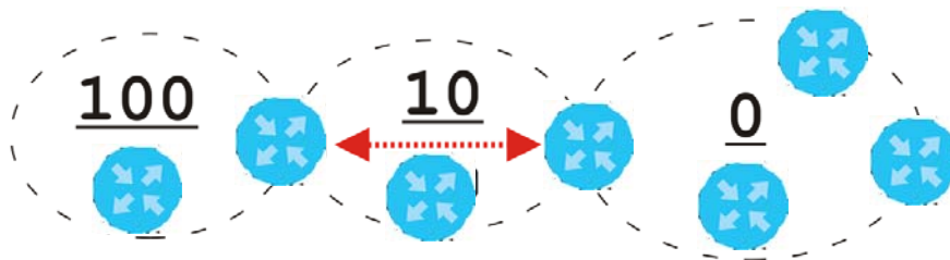
Figure 297 OSPF: Virtual Link
