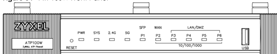
Figure 64 ATP100W Front Panel
