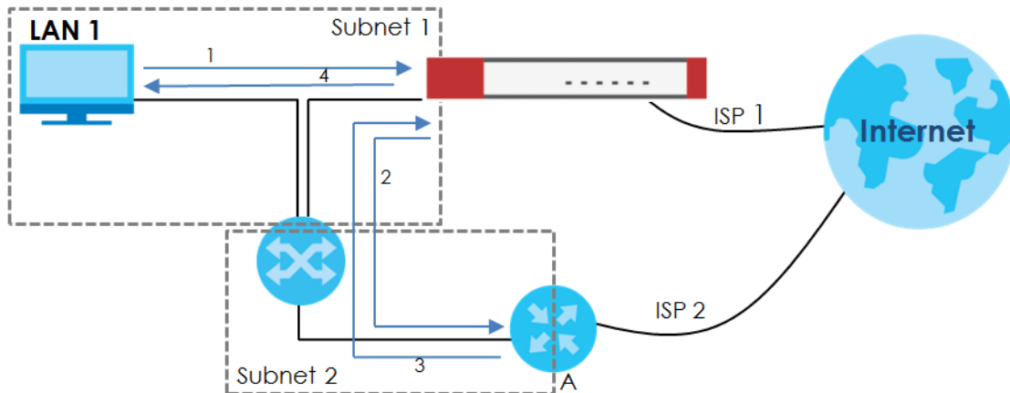
Figure 424 Using Virtual Interfaces to Avoid Asymmetrical Routes
