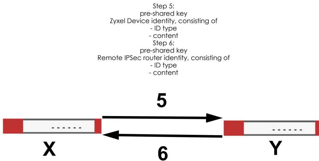
Figure 375 IKE SA: Main Negotiation Mode, Steps 5 - 6: Authentication (continued)
