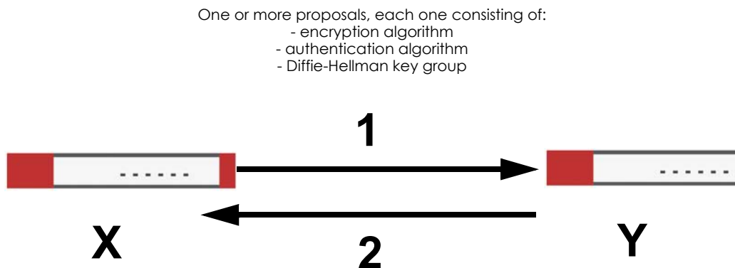
Figure 373 IKE SA: Main Negotiation Mode, Steps 1 - 2: IKE SA Proposal
