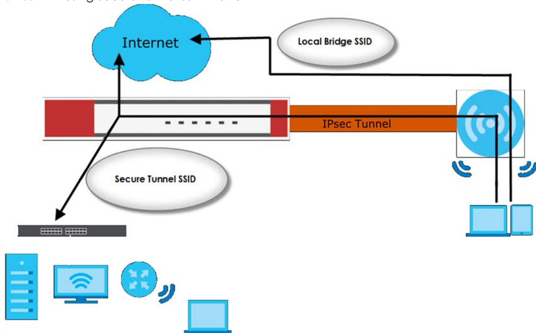
Figure 230 AP Using Secure Tunnel SSID Profile
