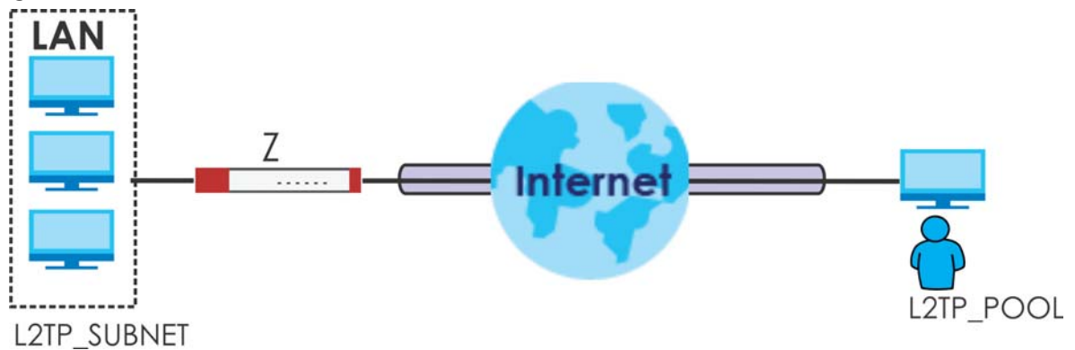
Figure 385 Policy Route for L2TP VPN
