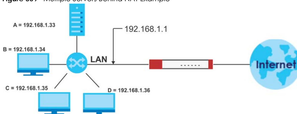
Figure 309 Multiple Servers Behind NAT Example
