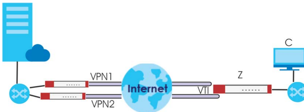
Figure 277 VTI and Trunk for VPN Load Balancing
