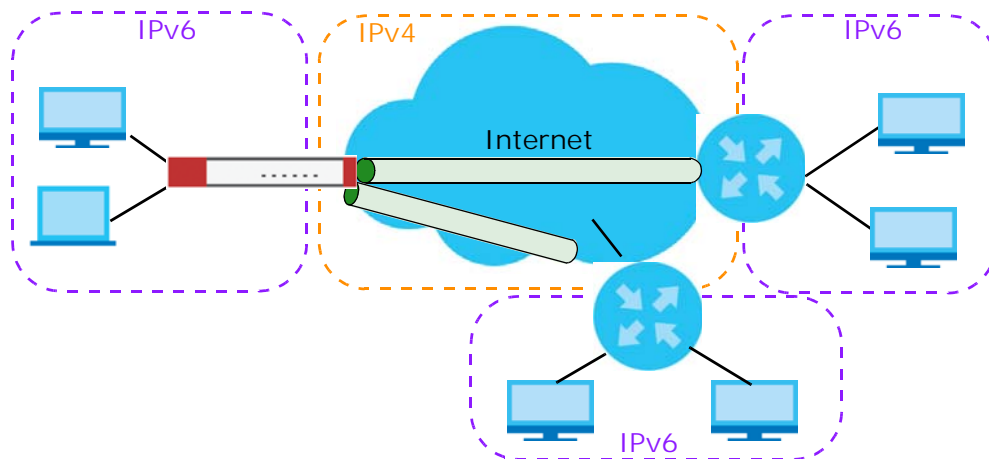
Figure 266 6to4 Tunnel
