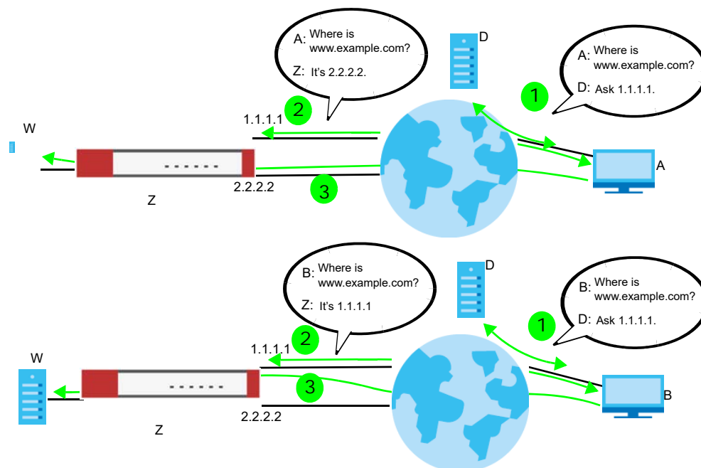
Figure 357 DNS Load Balancing Example
