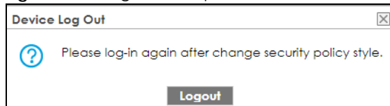
Figure 481 Logout Prompt
