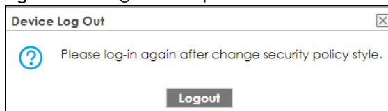
Figure 476 Logout Prompt
