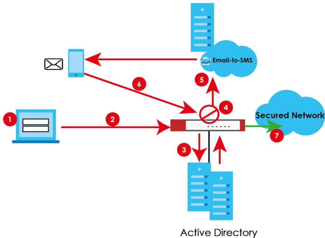
Figure 604 Two-Factor Authentication
