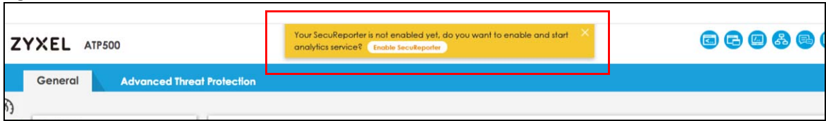
Figure 633 SecuReporter Banner
