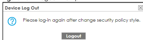
Figure 487 Logout Prompt
