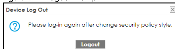
Figure 492 Logout Prompt
