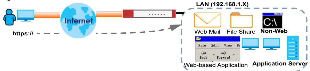
Figure 362 SSL VPN
