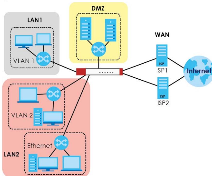
Figure 542 Example: Zones
