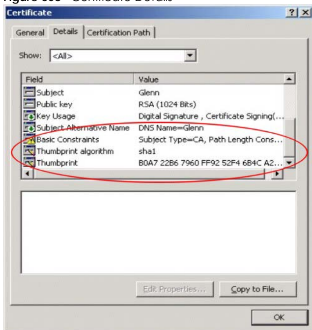
Figure 608 Certificate Details
