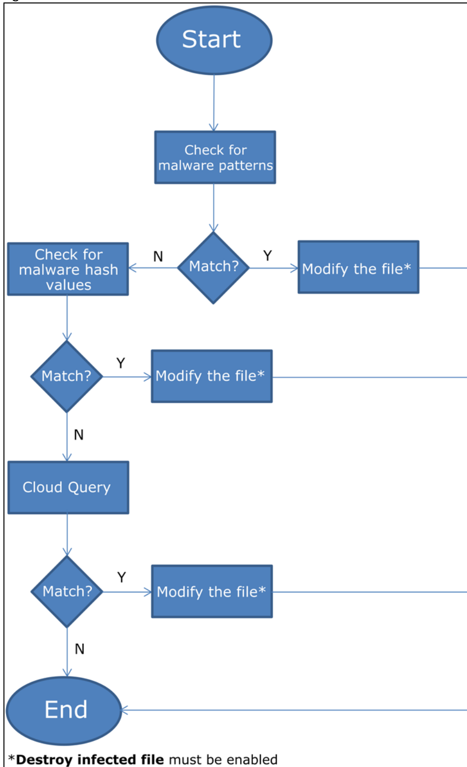
Figure 457 Anti-Malware Flowchart
