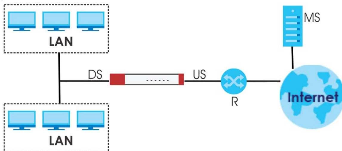
Figure 248 IGMP Proxy
