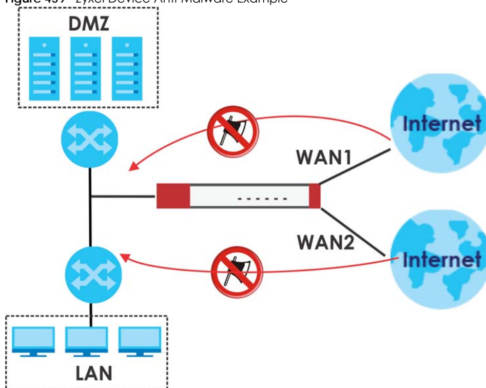
Figure 459 Zyxel Device Anti-Malware Example
