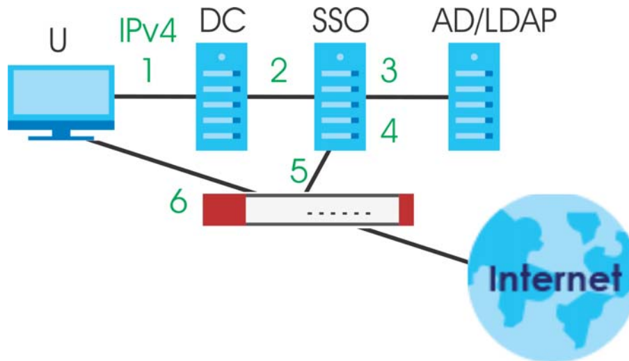
Figure 422 SSO Overview
