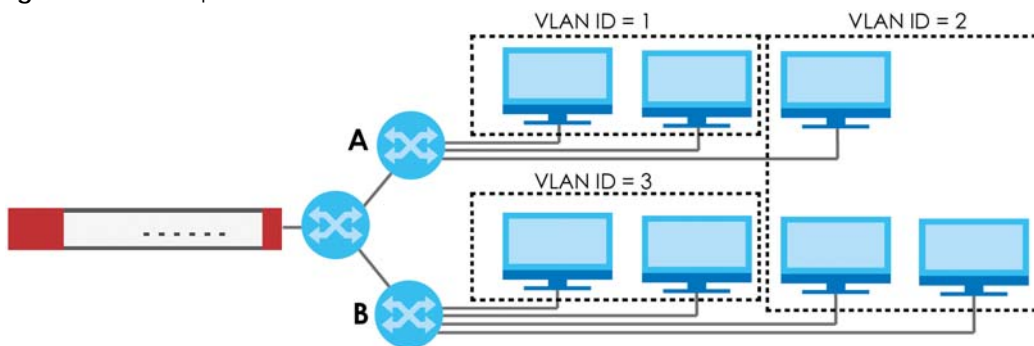
Figure 274 Example: After VLAN
