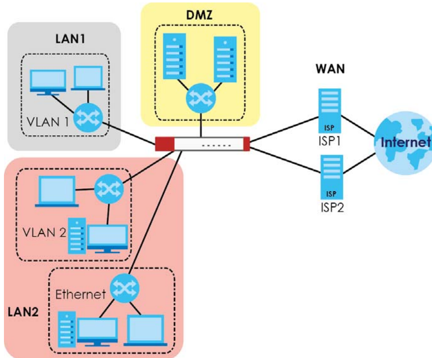
Figure 546 Example: Zones
