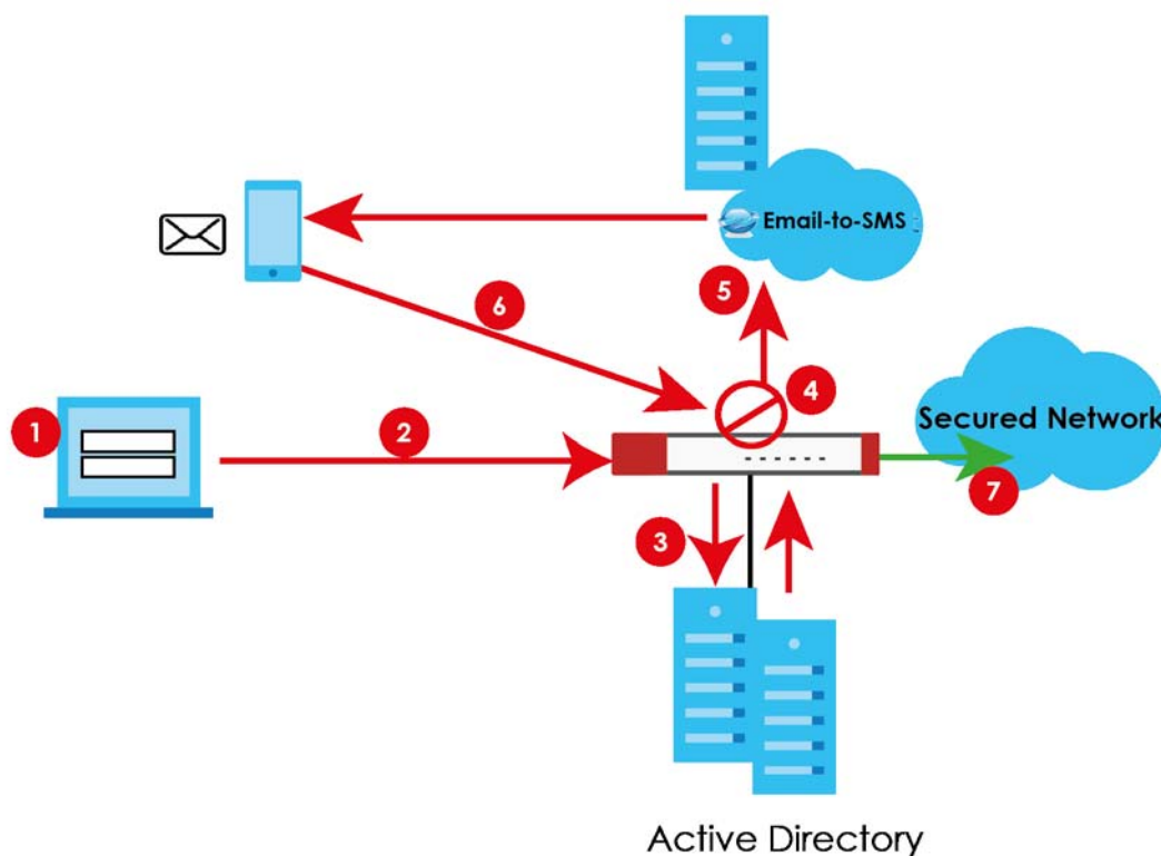
Figure 608 Two-Factor Authentication
