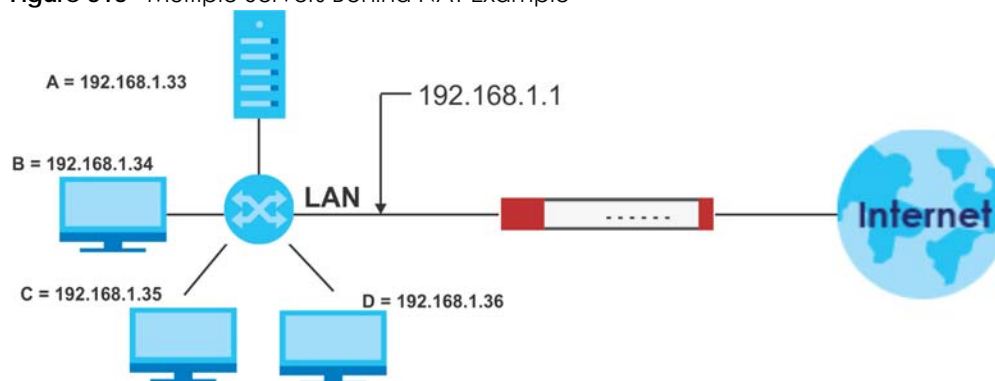
Figure 313 Multiple Servers Behind NAT Example
