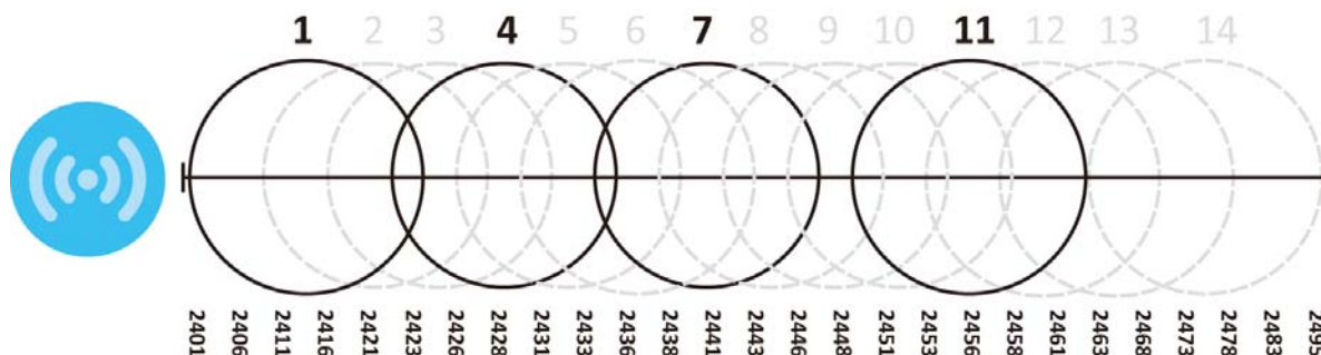
Figure 244 An Example Four-Channel Deployment
