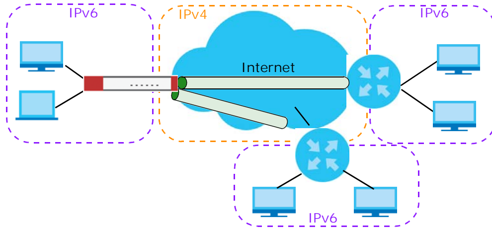
Figure 270 6to4 Tunnel
