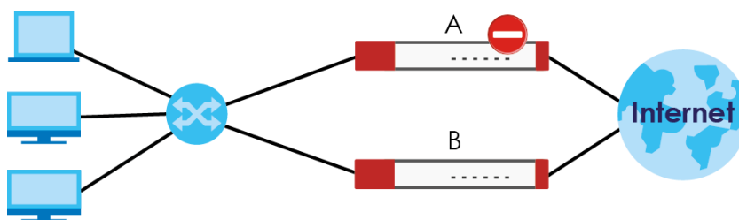
Figure 628 Device HA Backup Taking Over for the Master
