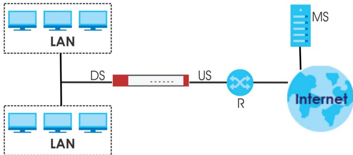
Figure 252 IGMP Proxy
