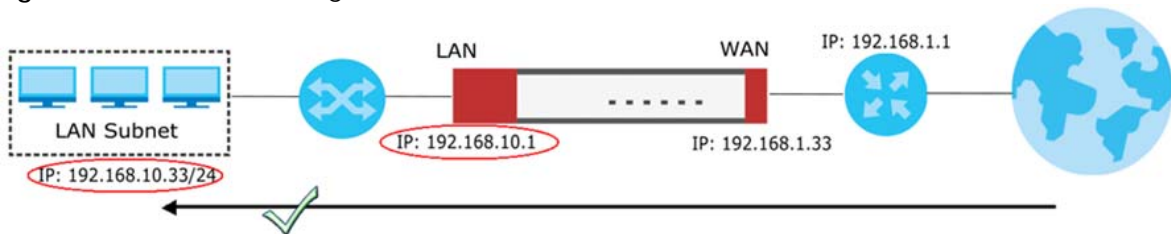
Figure 250 IP Address Change
