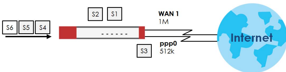
Figure 285 Weighted Round Robin Algorithm Example
