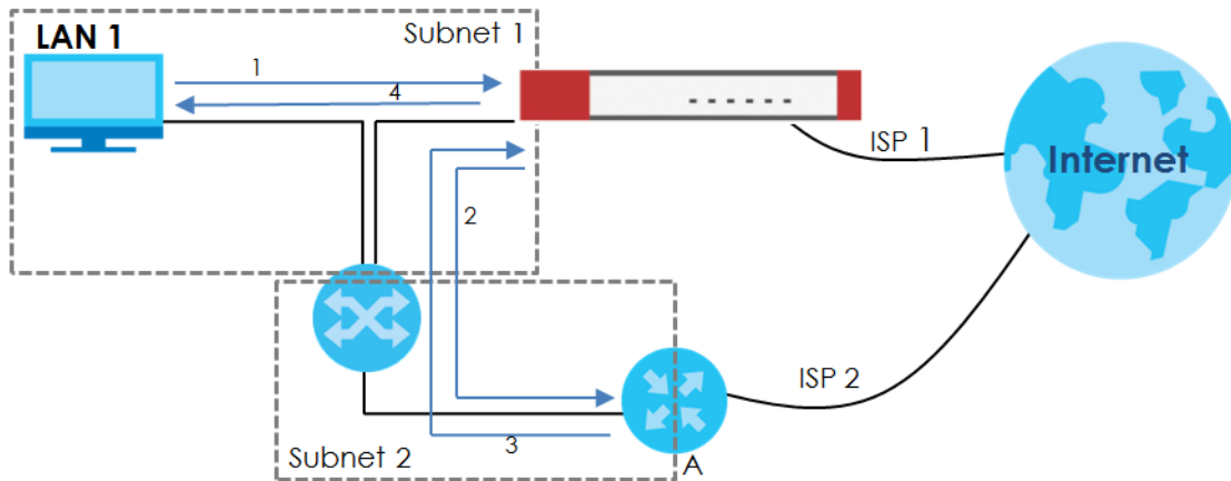
Figure 428 Using Virtual Interfaces to Avoid Asymmetrical Routes
