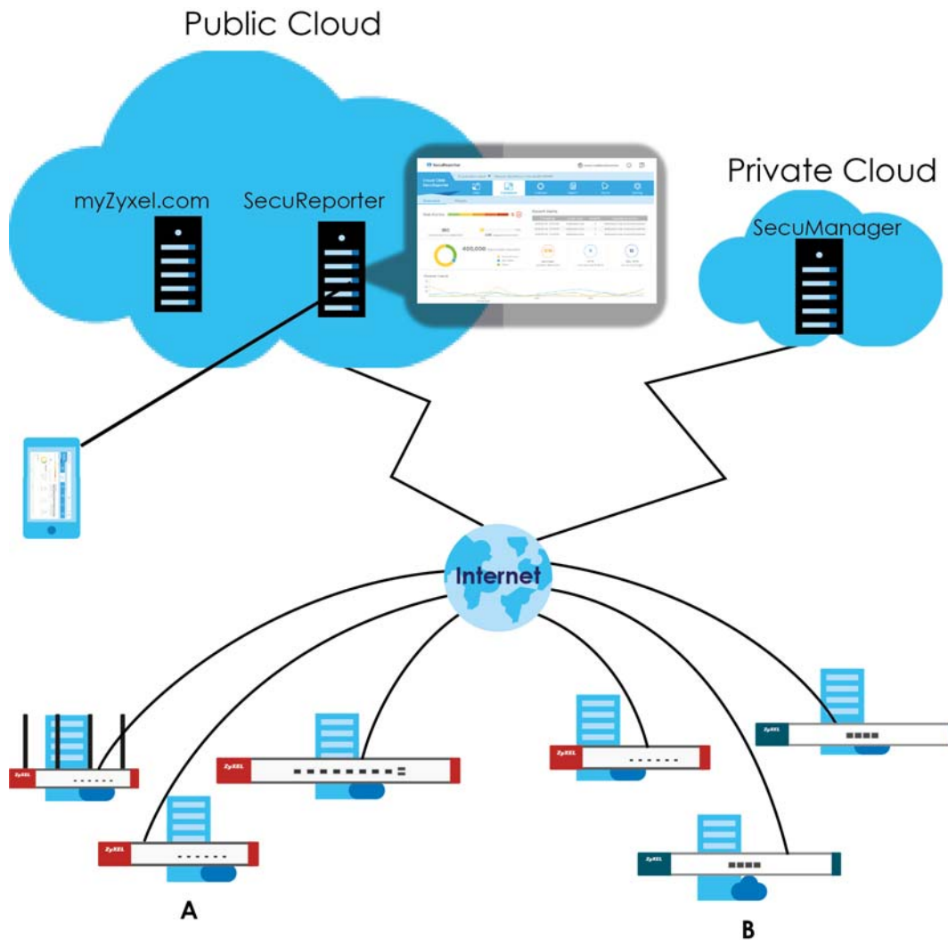
Figure 635 Cloud CNM SecuReporter Application Scenario
