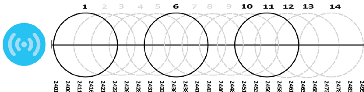
Figure 243 An Example Three-Channel Deployment
