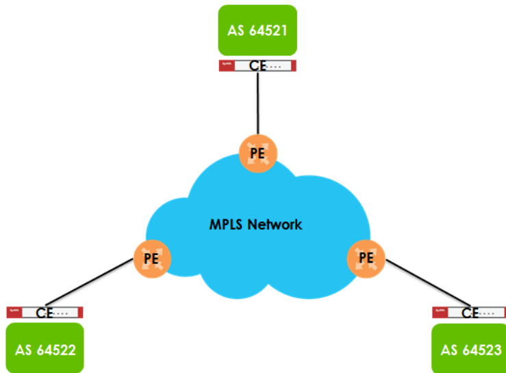
Figure 309 Scenario 1: CE Router - to - MPLS
