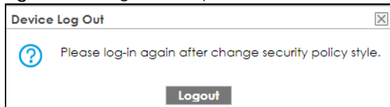
Figure 521 Logout Prompt
