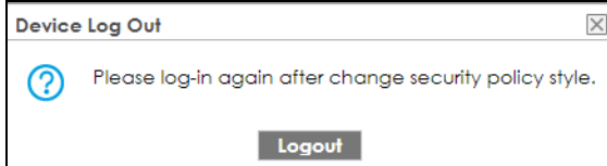
Figure 473 Logout Prompt
