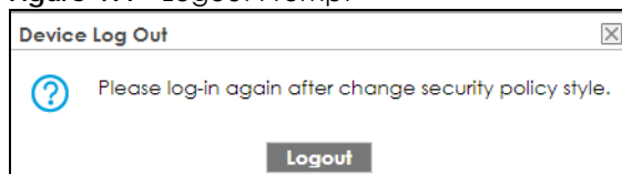
Figure 497 Logout Prompt
