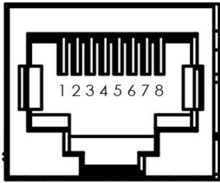
Figure 71 RJ-45 Connector Pins
