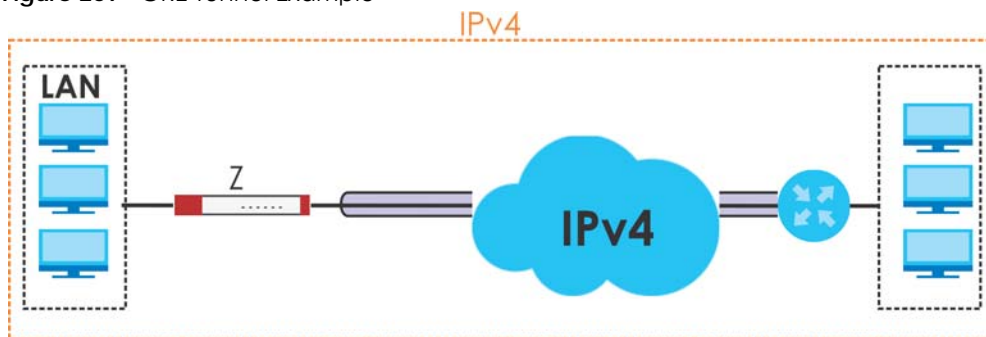
Figure 269 GRE Tunnel Example
