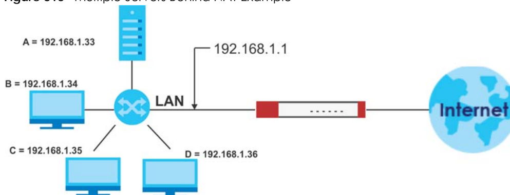
Figure 315 Multiple Servers Behind NAT Example
