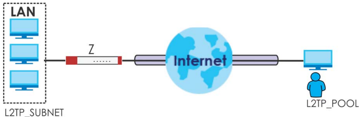
Figure 391 Policy Route for L2TP VPN
