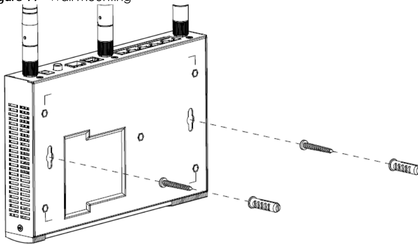
Figure 77 Wall Mounting
