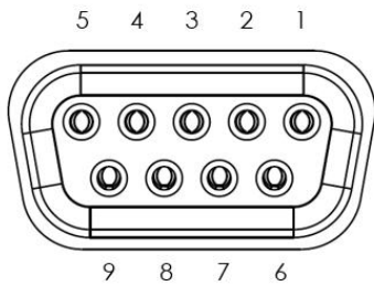
Figure 72 DB-9 Connector Pins
