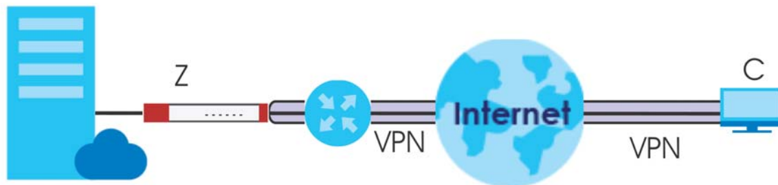
Figure 393 L2TP and Zyxel Device Behind a NAT Router
