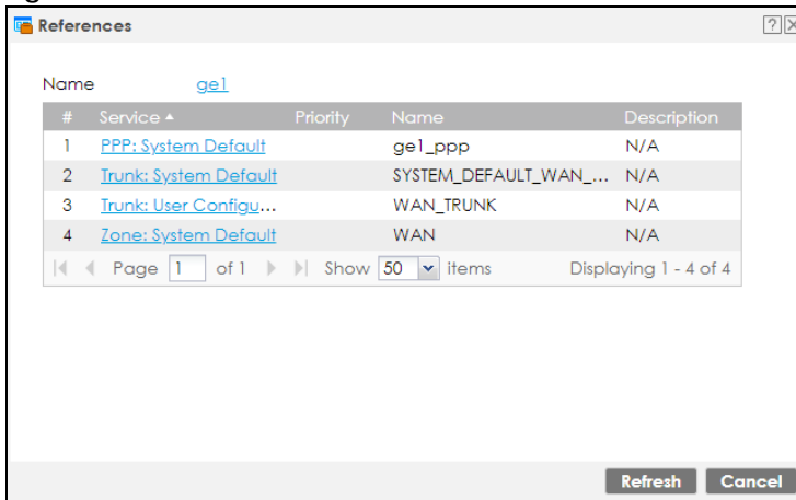
Figure 261 References
