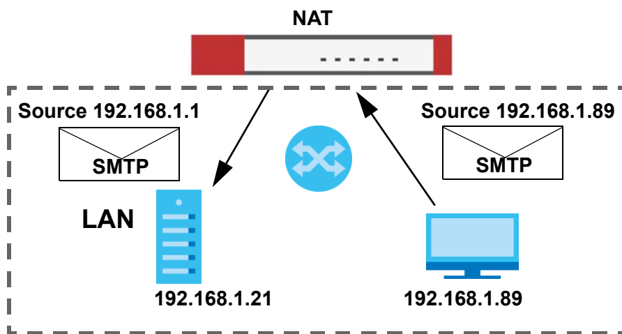
Figure 319 LAN to LAN Traffic
