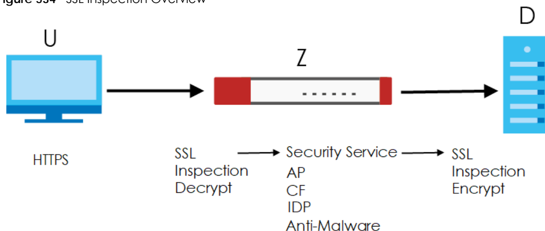
Figure 534 SSL Inspection Overview
