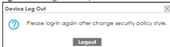
Figure 526 Logout Prompt
