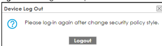
Figure 492 Logout Prompt
