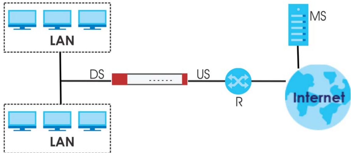
Figure 254 IGMP Proxy
