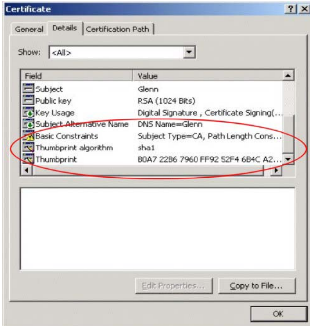
Figure 614 Certificate Details
