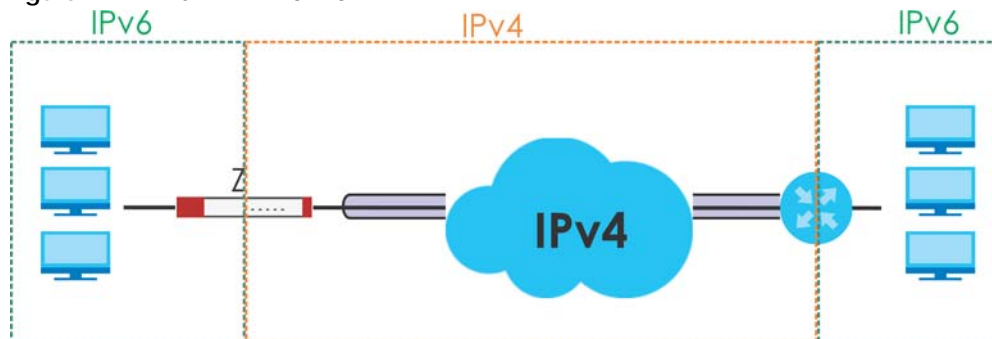
Figure 271 IPv6-in-IPv4 Tunnel
