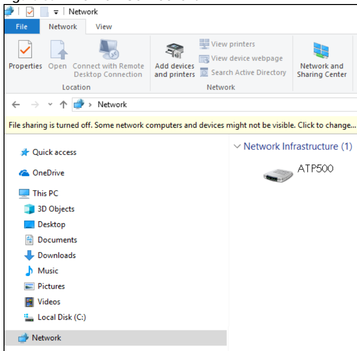
Figure 351 Network Connections
