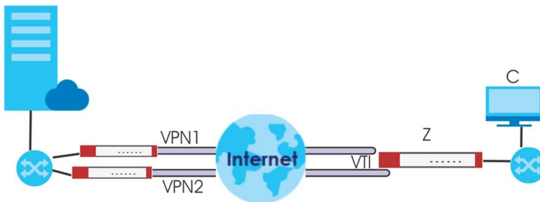
Figure 283 VTI and Trunk for VPN Load Balancing
