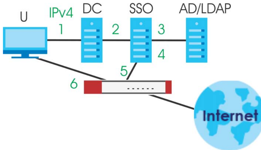
Figure 421 SSO Overview
