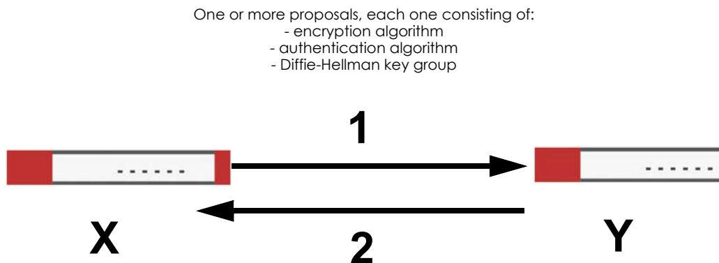
Figure 376 IKE SA: Main Negotiation Mode, Steps 1 - 2: IKE SA Proposal
