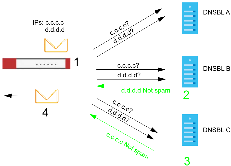
Figure 525 DNSBL Legitimate Email Detection Example
