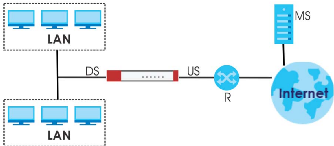
Figure 251 IGMP Proxy
