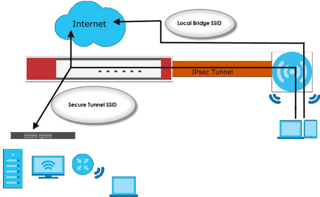
Figure 229 AP Using Secure Tunnel SSID Profile
