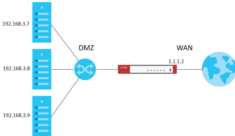
Figure 318 Virtual Server on the WAN- Example 1
