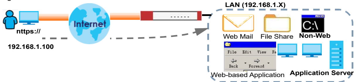
Figure 383 Network Access Mode: Full Tunnel Mode
