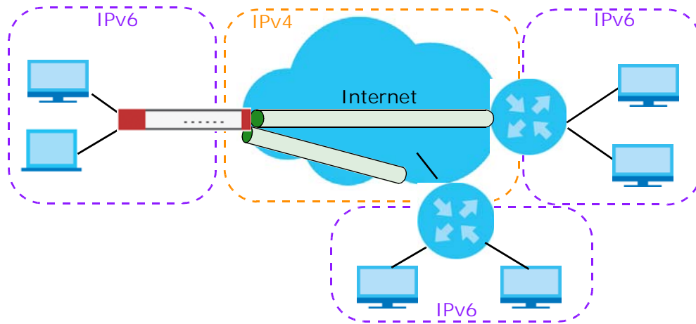
Figure 269 6to4 Tunnel
