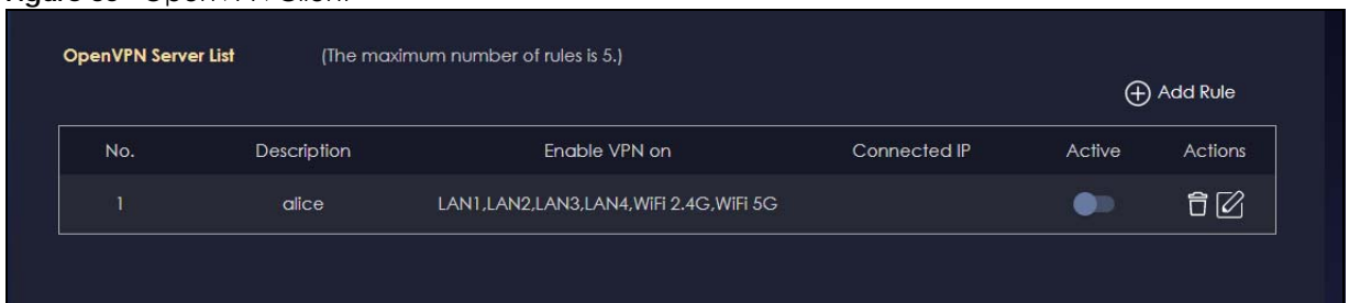
Figure 35 OpenVPN Client
