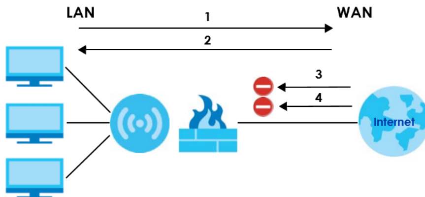
Figure 80 Default Firewall Action
