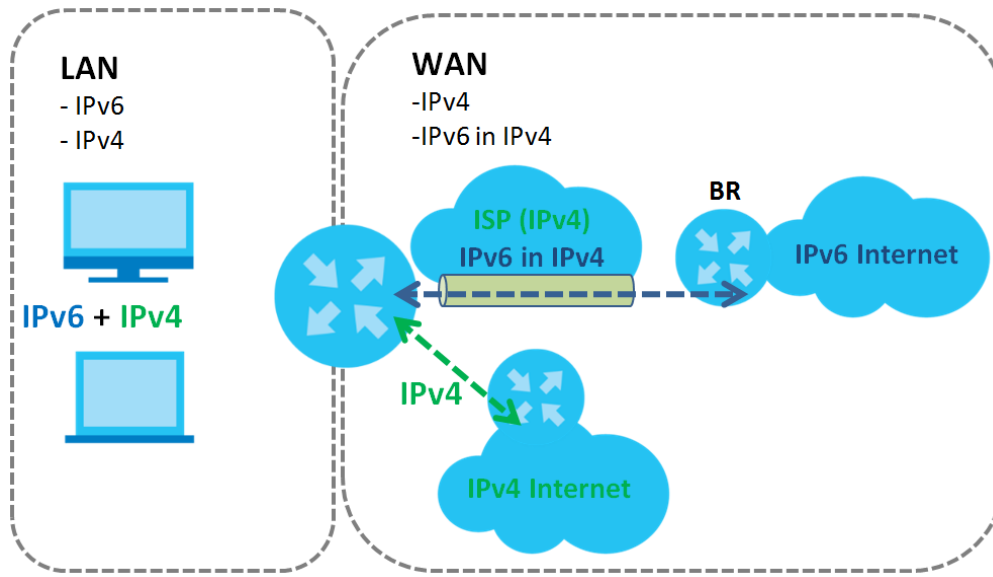
Figure 50 IPv6 Rapid Deployment
