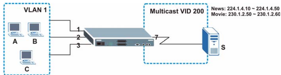
Figure 81 MVR Configuration Example
