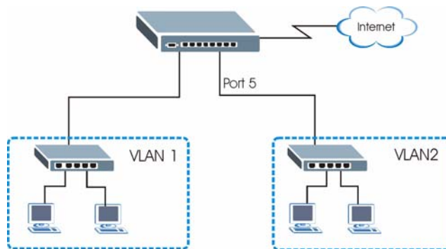
Figure 25 Initial Setup Network Example: VLAN
