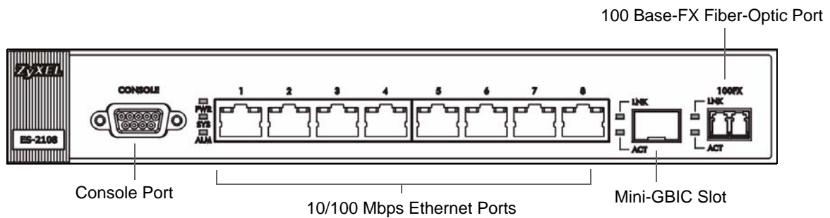
Figure 13 Front Panel: ES-2108-LC
