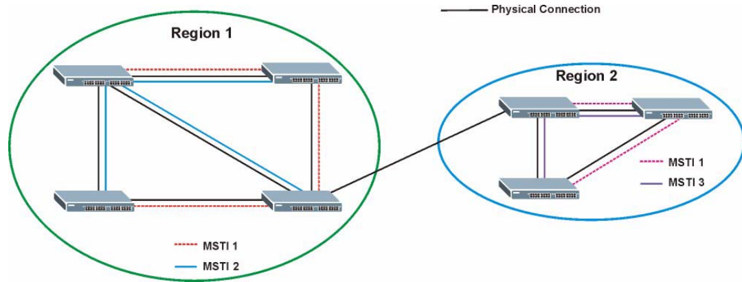
Figure 51 MSTIs in Different Regions
