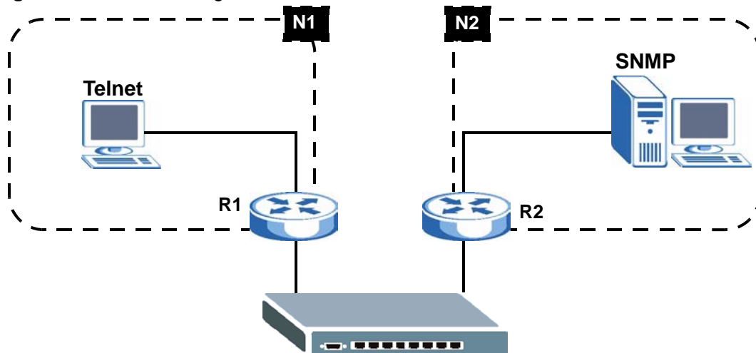
Figure 103 Static Routing Overview
