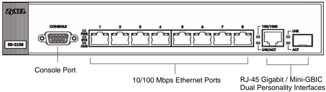
Figure 12 Front Panel: ES-2108-G/ES-2108PWR
