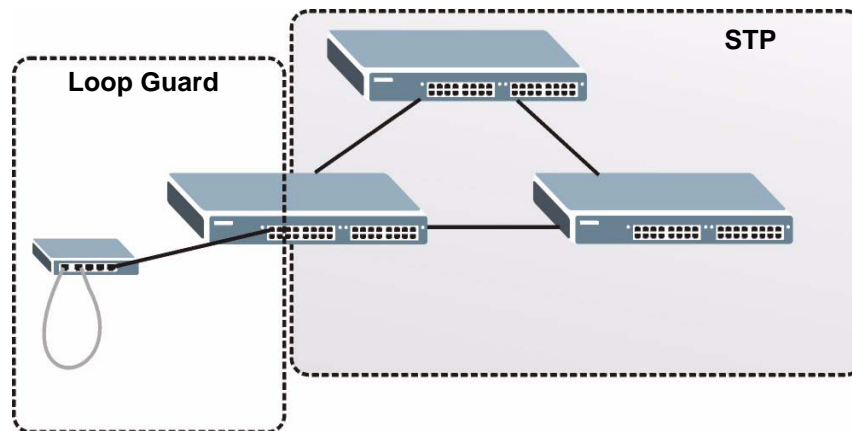
Figure 98 Loop Guard vs STP
