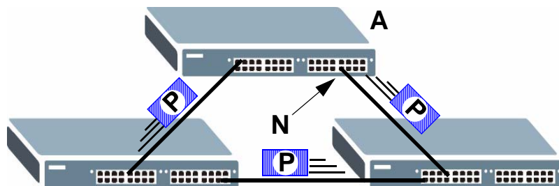
Figure 101 Loop Guard - Network Loop
