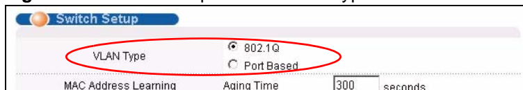
Figure 40 Switch Setup: Select VLAN Type
