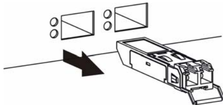
Figure 17 Transceiver Removal Example
