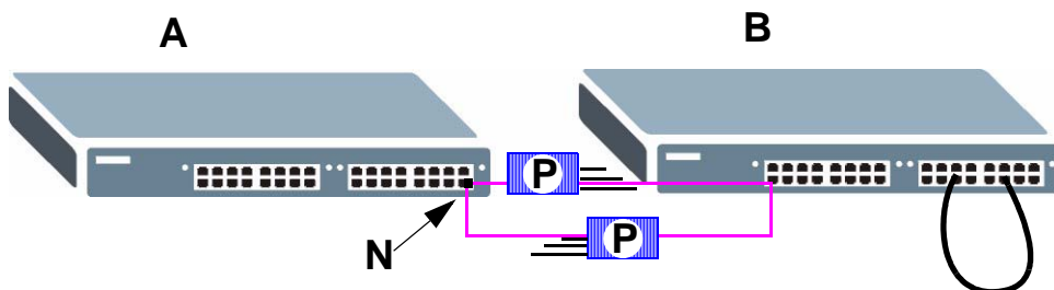
Figure 100 Loop Guard - Probe Packet
