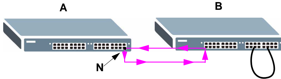
Figure 99 Switch in Loop State
