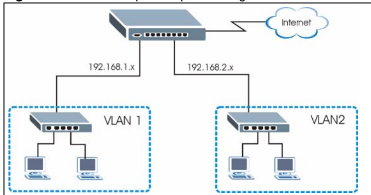
Figure 27 Initial Setup Example: Management IP Address
