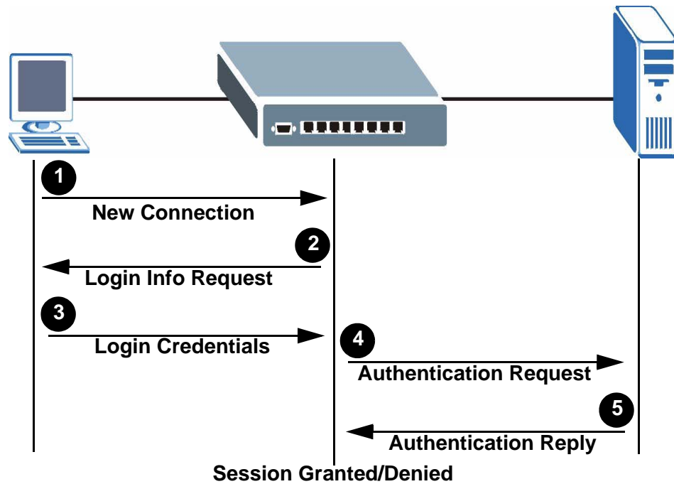
Figure 67 IEEE 802.1x Authentication Process
