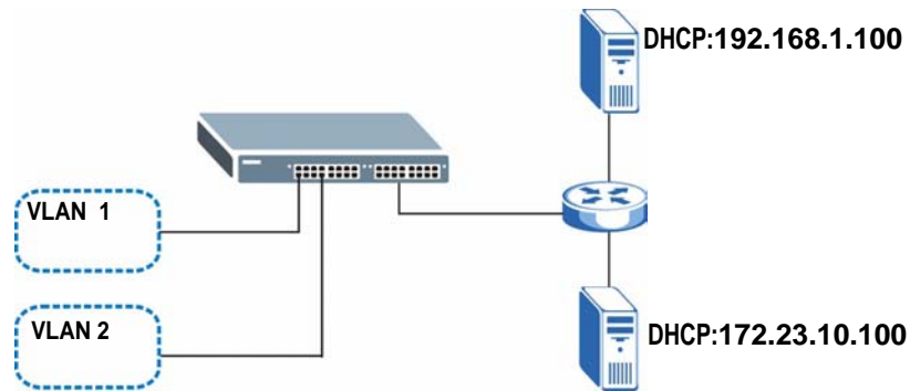
Figure 114 DHCP Relay for Two VLANs
