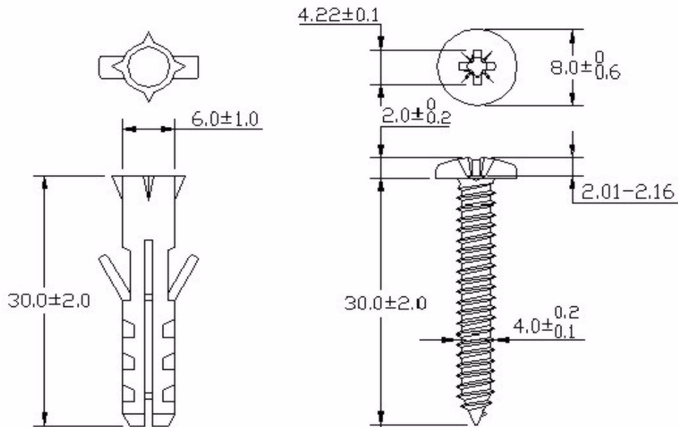
Figure 157 Masonry Plug and M4 Tap Screw
