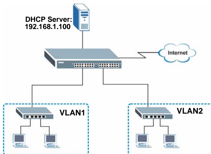
Figure 111 Global DHCP Relay Network Example
