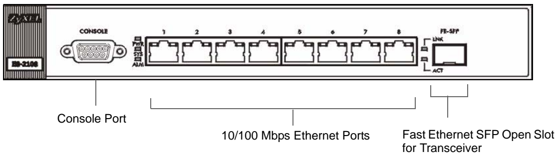
Figure 11 Front Panel: ES-2108-F
