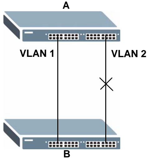
Figure 49 STP/RSTP Network Example
