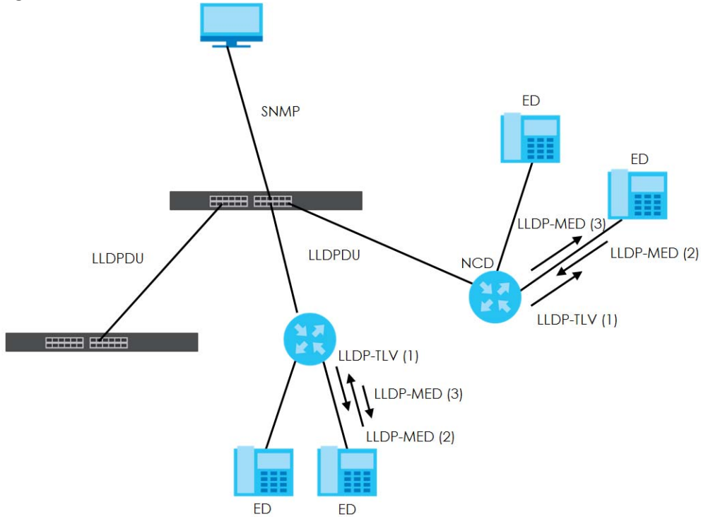
Figure 154 LLDP-MED Overview
