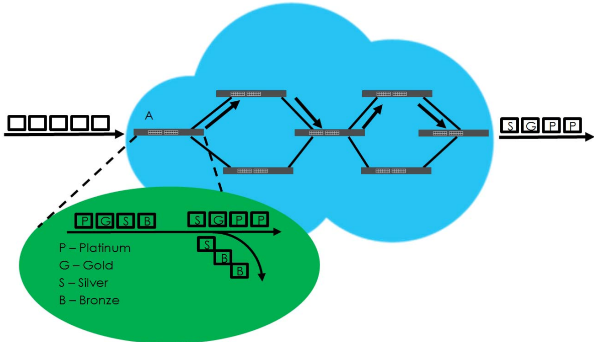
Figure 174 DiffServ Network
