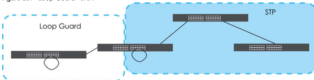
Figure 259 Loop Guard vs. STP
