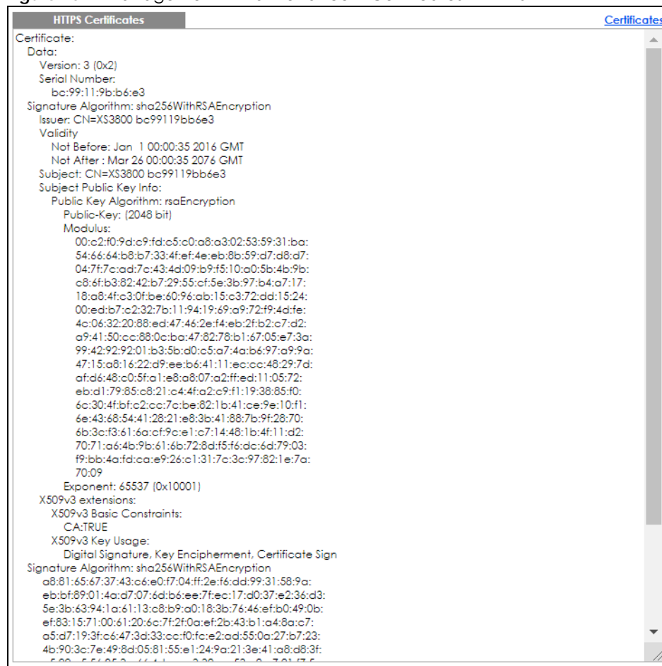
Figure 201 Management > Maintenance > Certificates > HTTPS
