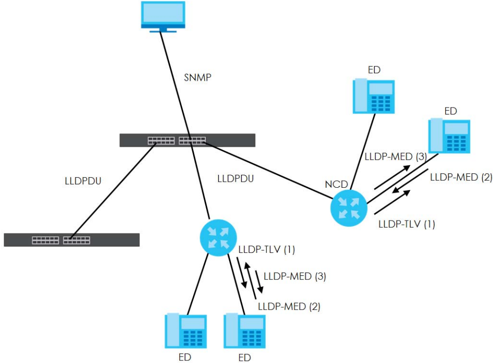
Figure 154 LLDP-MED Overview
