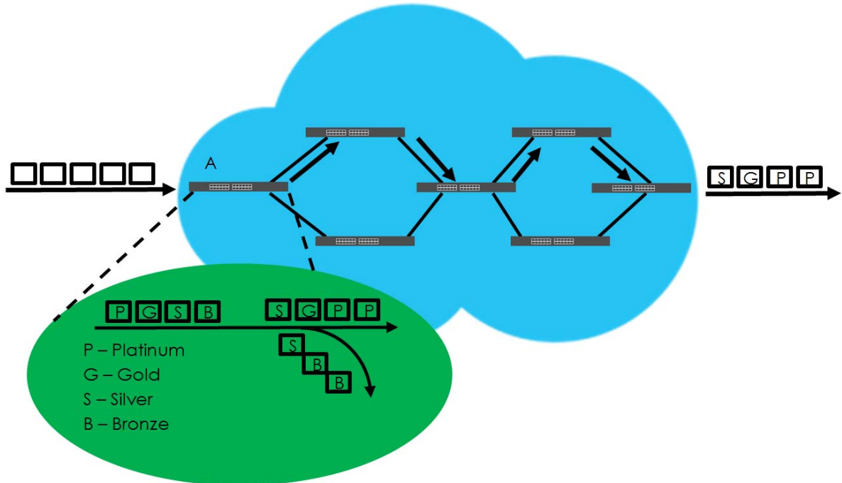
Figure 174 DiffServ Network
