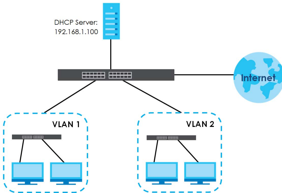
Figure 168 Global DHCP Relay Network Example
