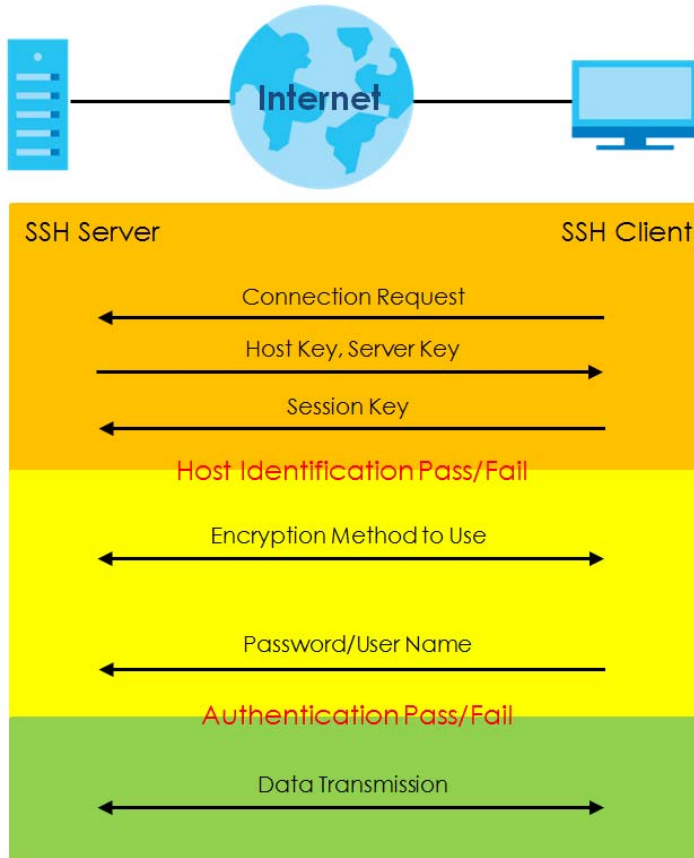
Figure 199 How SSH Works
