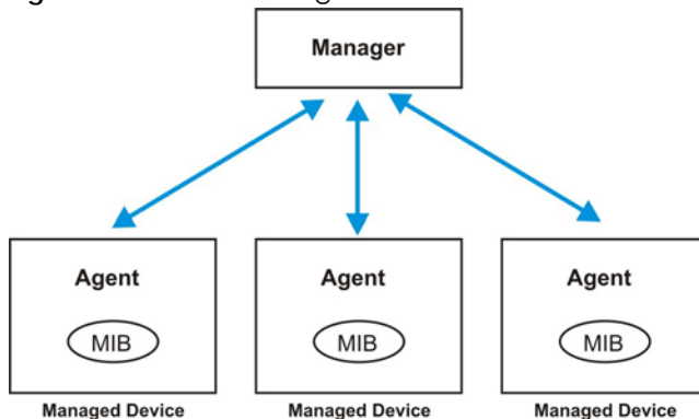
Figure 197 SNMP Management Model
