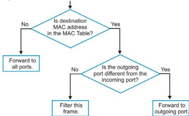
Figure 217 MAC Table Flowchart
