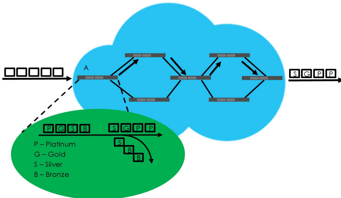
Figure 160 DiffServ Network
