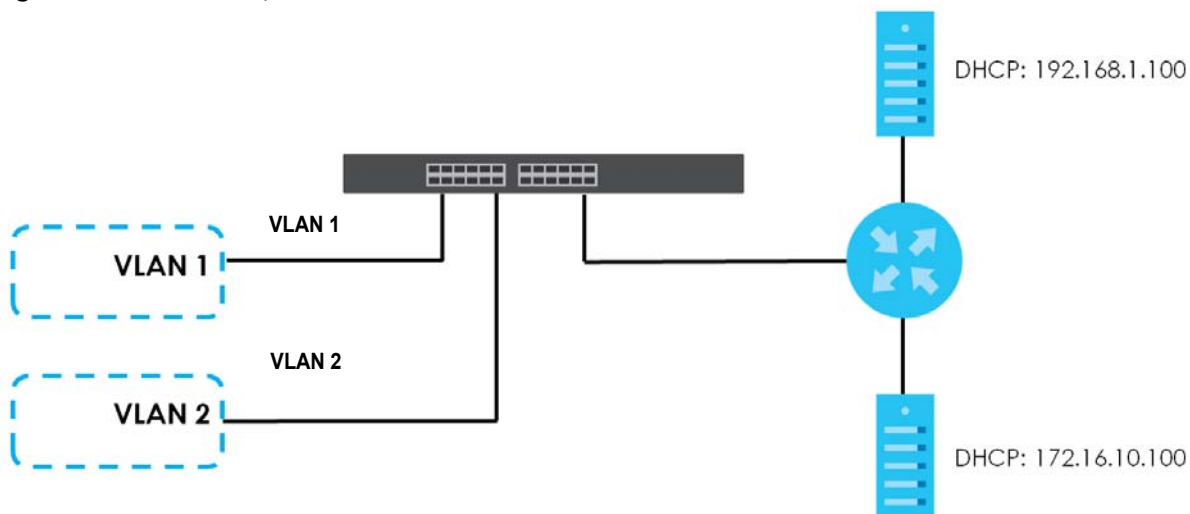
Figure 172 DHCP Relay for Two VLANs
