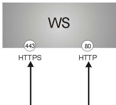
Figure 200 HTTPS Implementation
