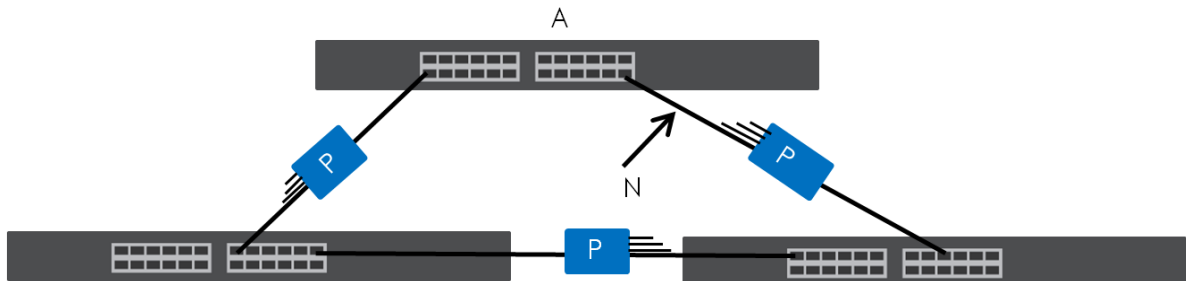
Figure 136 Loop Guard – Network Loop
