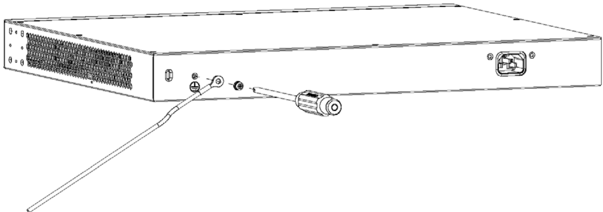
Figure 32 Grounding
