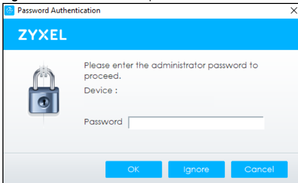
Figure 45 Password Prompt
