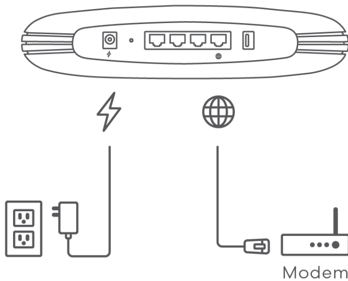
Figure 1 WSQ60/WSQ50 Rear Panel
