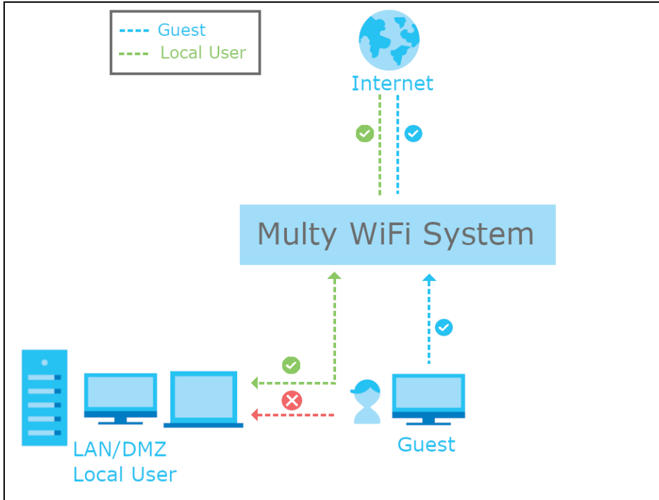
Figure 15 Guest WiFi
