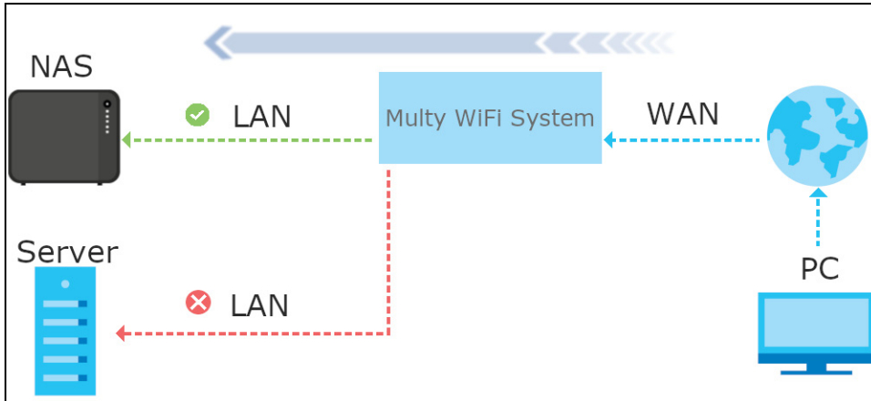
Figure 17 Port Forwarding
