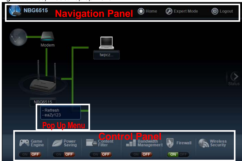
Figure 26 Easy Mode: Pop Up Menu
