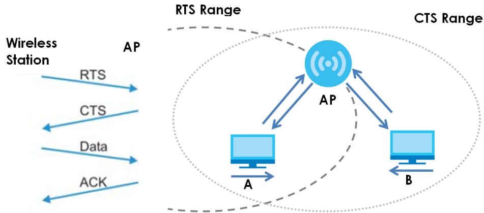
Figure 139 RTS/CTS
