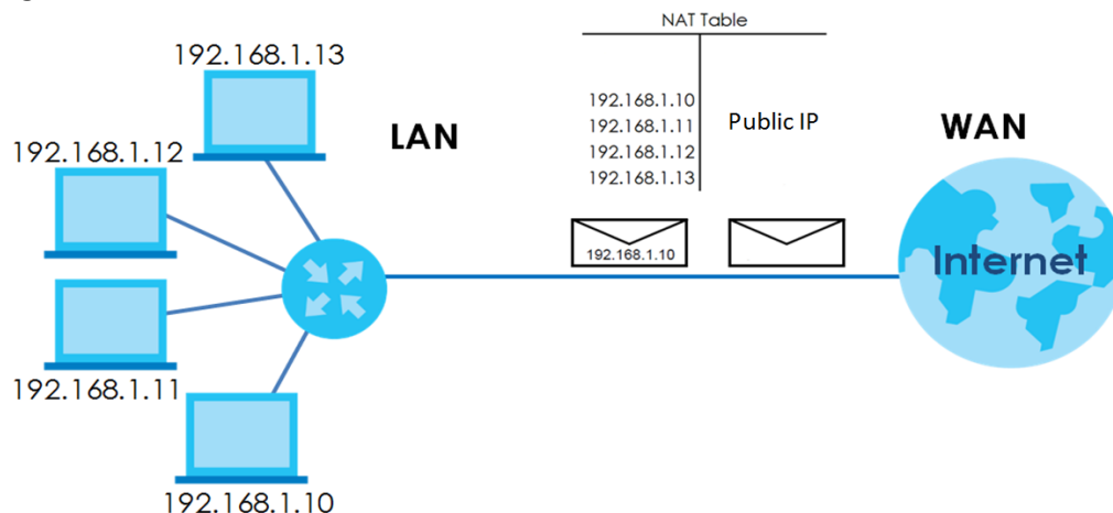
Figure 82 NAT Example
