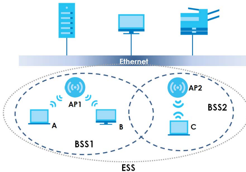
Figure 138 Infrastructure WLAN
