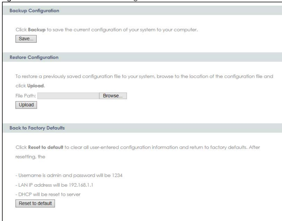
Figure 90 Maintenance &gt; Tools &gt; Configuration
