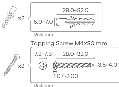
Figure 3 Screw Specifications
