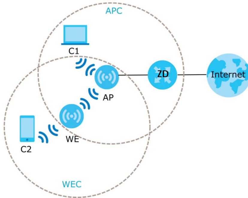
Figure 6 Mesh Application
