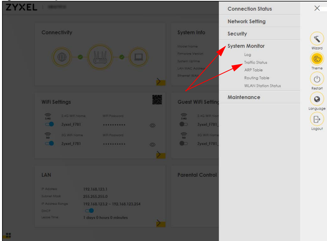
Figure 28 Navigation Panel
