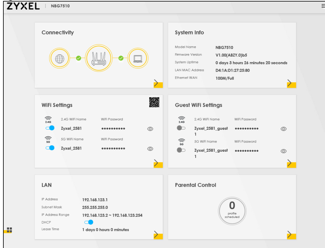
Figure 24 Connection Status
