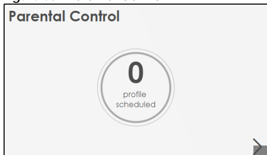
Figure 53 Parental Control
