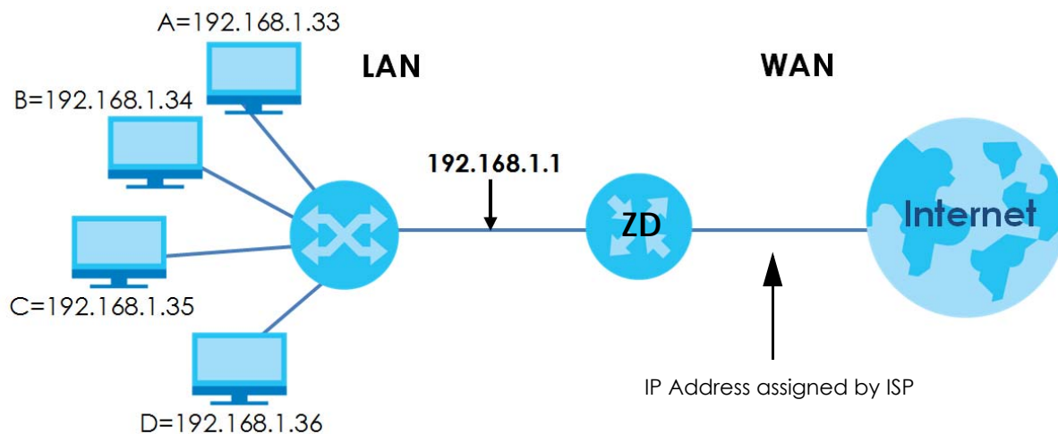
Figure 120 Multiple Servers Behind NAT Example
