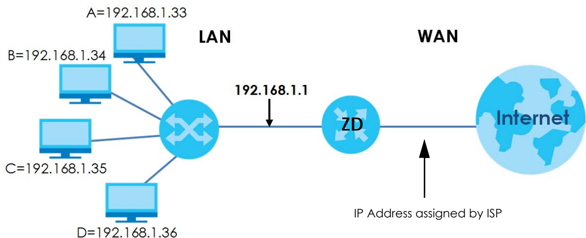
Figure 122 Multiple Servers Behind NAT Example
