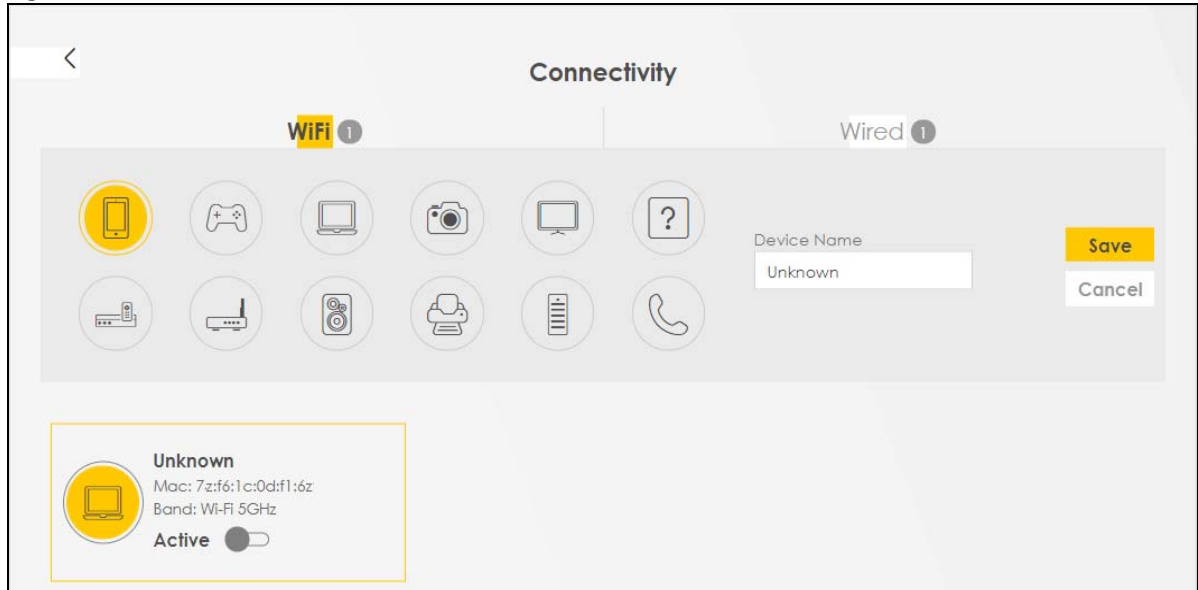
Figure 38 Connectivity: Edit
