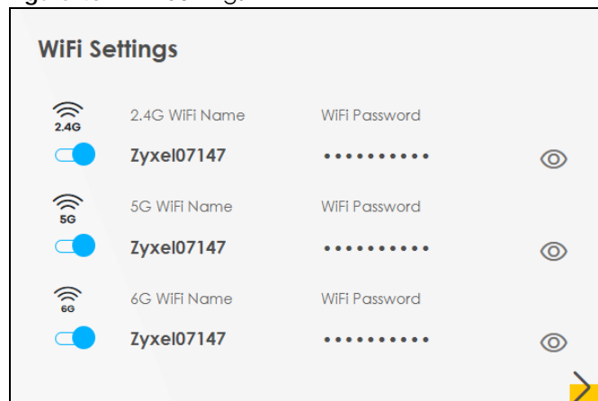
Figure 43 WiFi Settings
