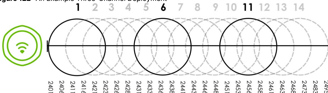
Figure 122 An Example Three-Channel Deployment
