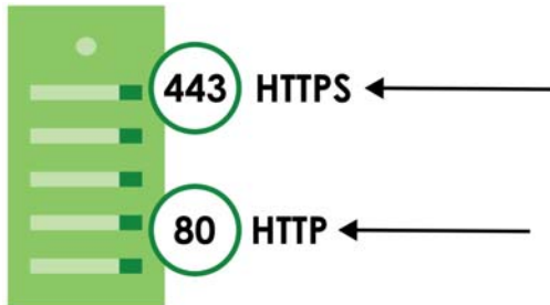
Figure 170 HTTP/HTTPS Implementation
