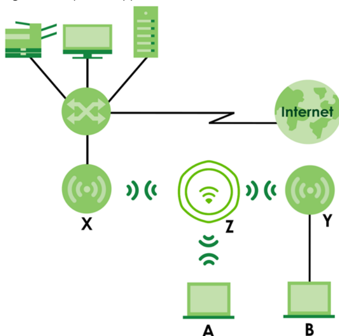
Figure 5 Repeater Application
