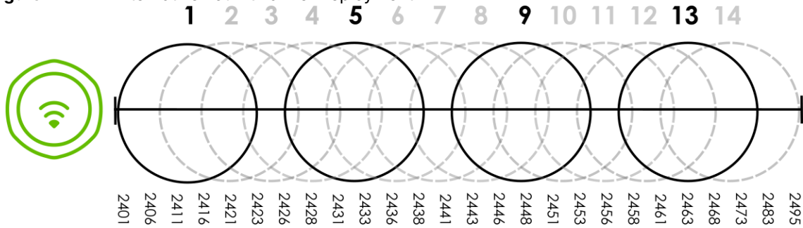
Figure 124 An Alternative Four-Channel Deployment
