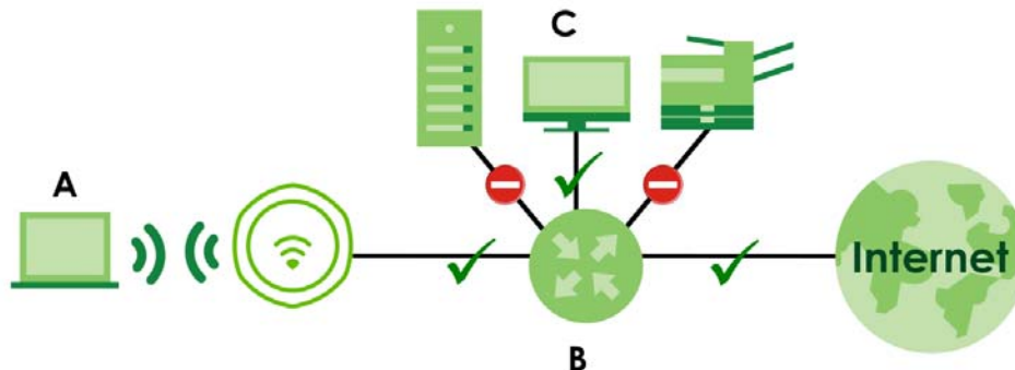
Figure 153 Layer-2 Isolation Application
