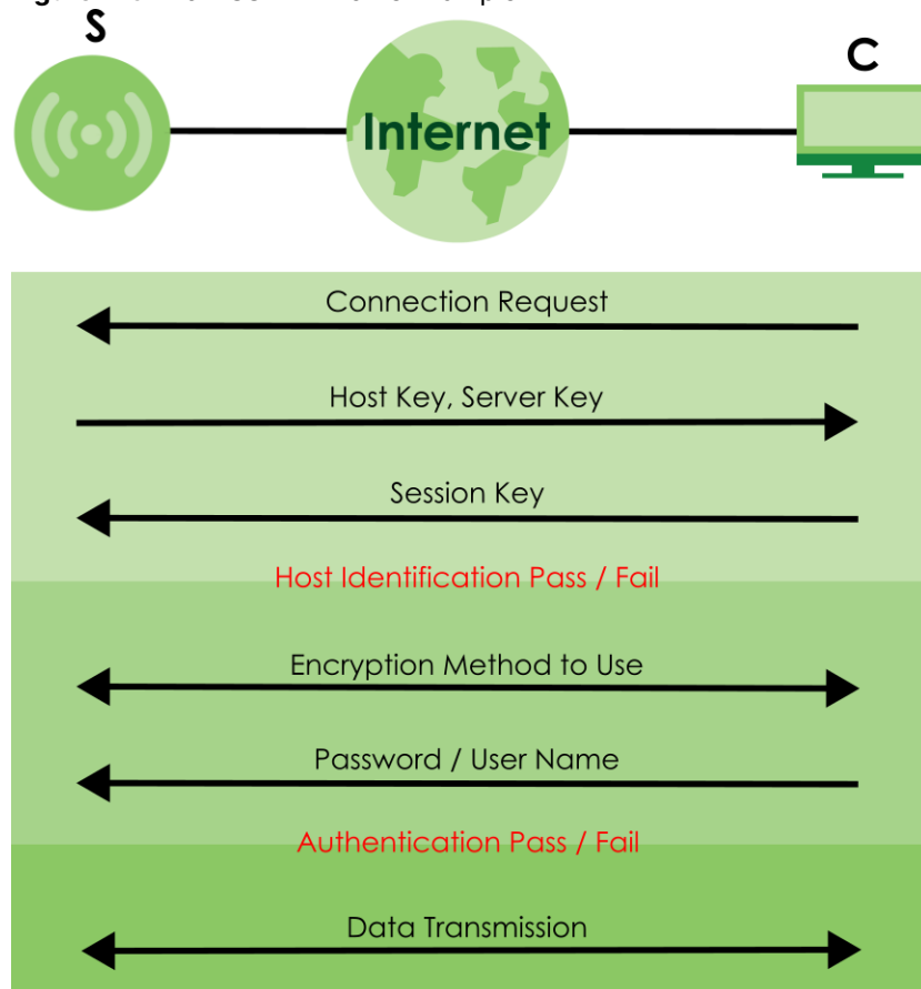
Figure 176 How SSH v1 Works Example
