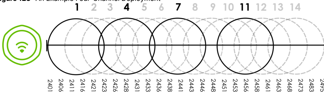
Figure 123 An Example Four-Channel Deployment
