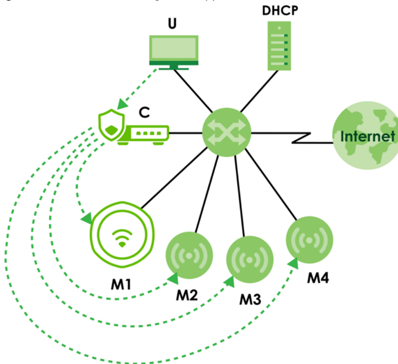
Figure 209 Controller Managed AP Application
