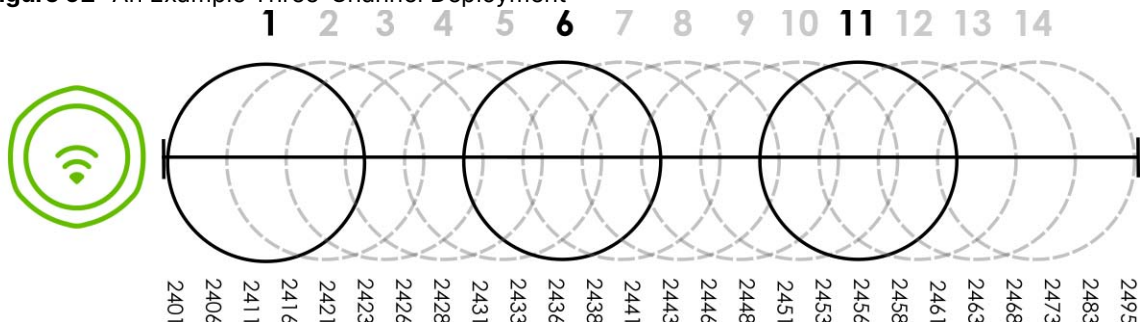
Figure 92 An Example Three-Channel Deployment
