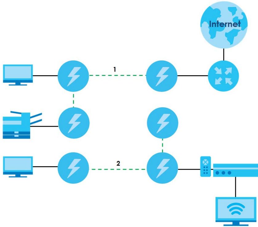
Figure 18 Add New Adapters to Make a Second Network
