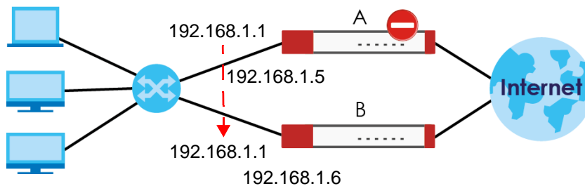
Figure 540 Management IP Addresses
