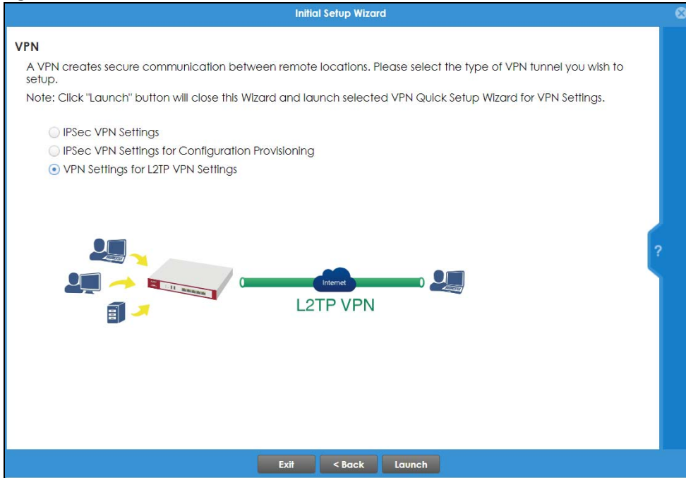
Figure 100 VPN Settings for L2TP VPN Settings Wizard: L2TP VPN Settings
