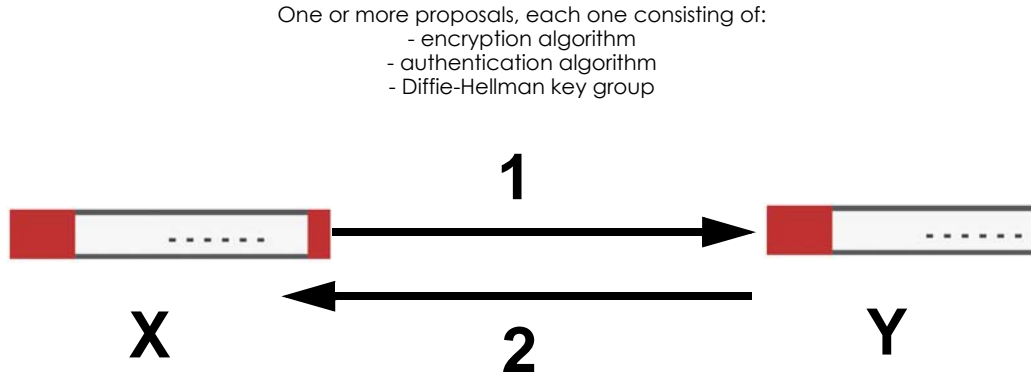
Figure 438 IKE SA: Main Negotiation Mode, Steps 1 - 2: IKE SA Proposal
