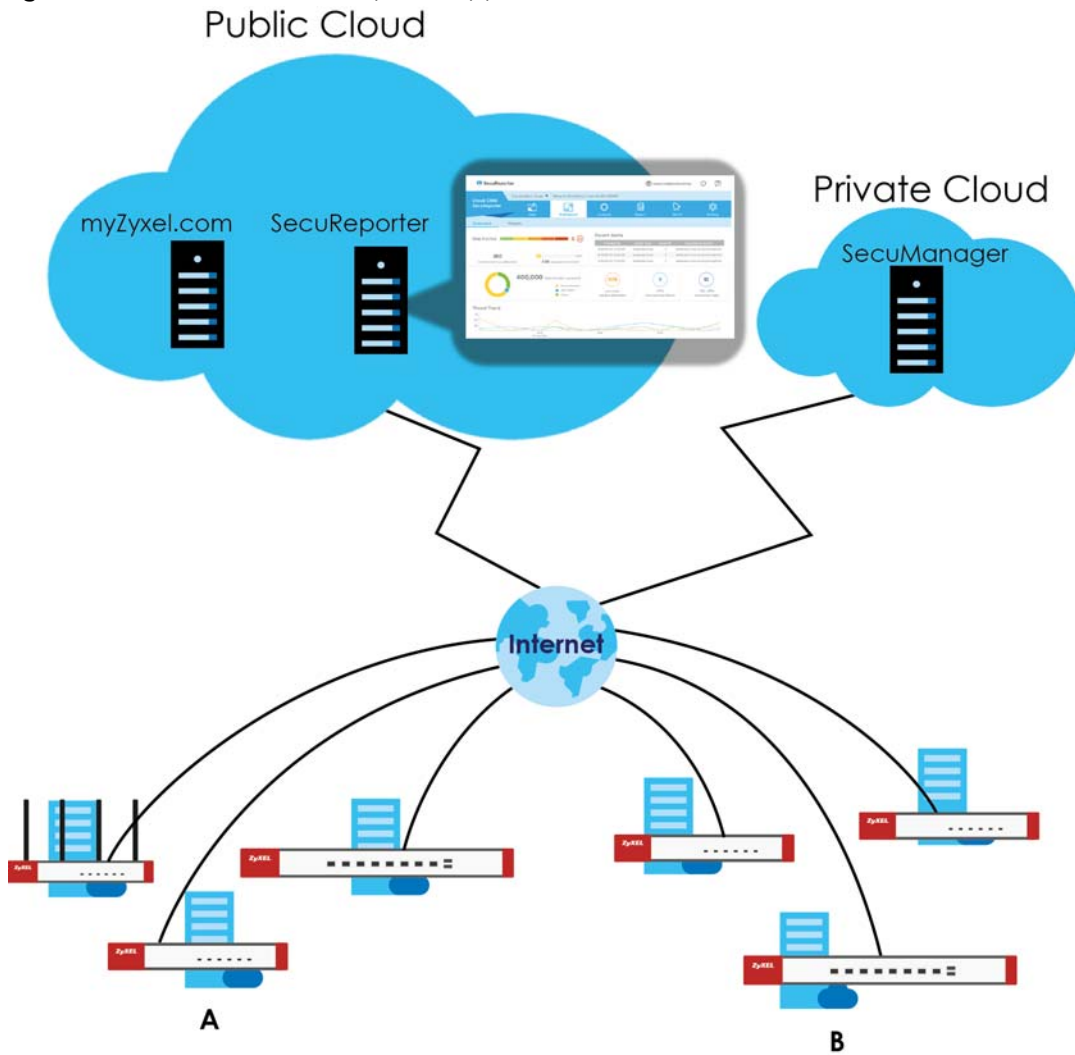
Figure 419 Cloud CNM SecuReporter Application Scenario
