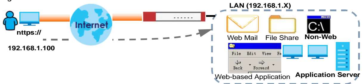
Figure 445 Network Access Mode: Full Tunnel Mode
