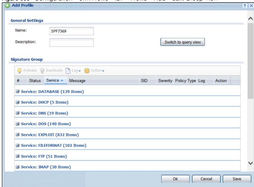
Figure 503 Configuration > UTM Profile > IDP > Profile > Add > Edit: Group View
