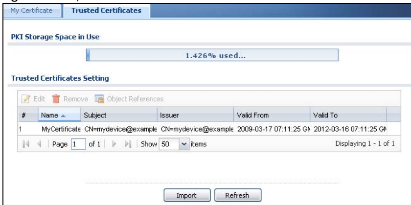
Figure 656 Zyxel Device Trusted CA Screen
