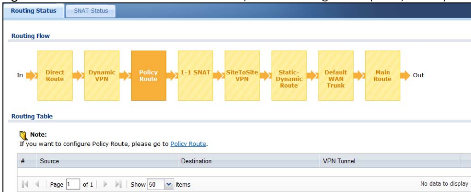
Figure 727 Maintenance > Packet Flow Explore > Routing Status (Policy Route)
