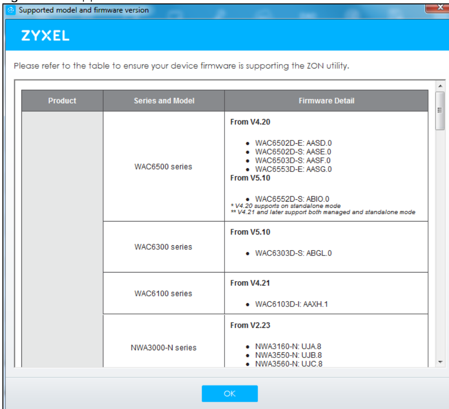
Figure 684 Supported Devices and Versions
