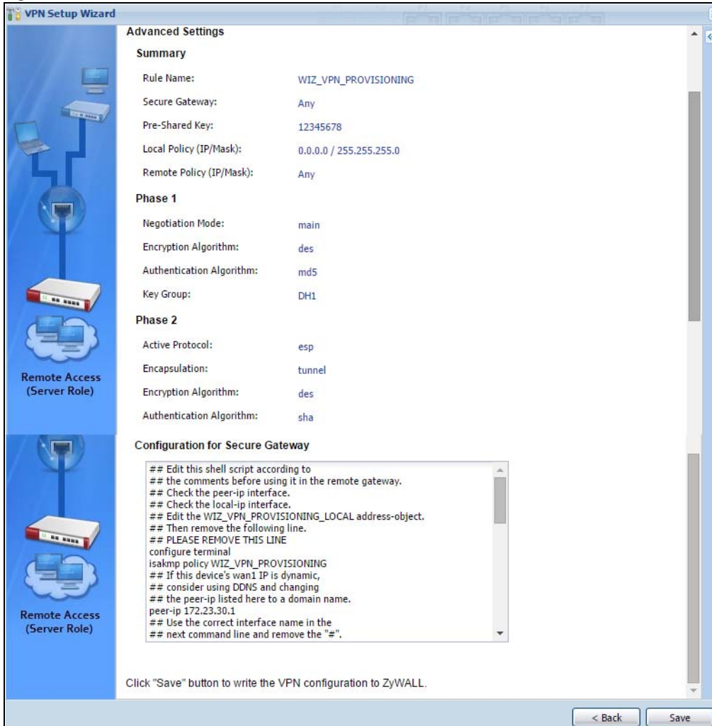
Figure 146 VPN for Configuration Provisioning Advanced Wizard: Summary
