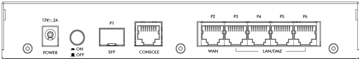
Figure 55 USG40 / USG40W Rear Panel
