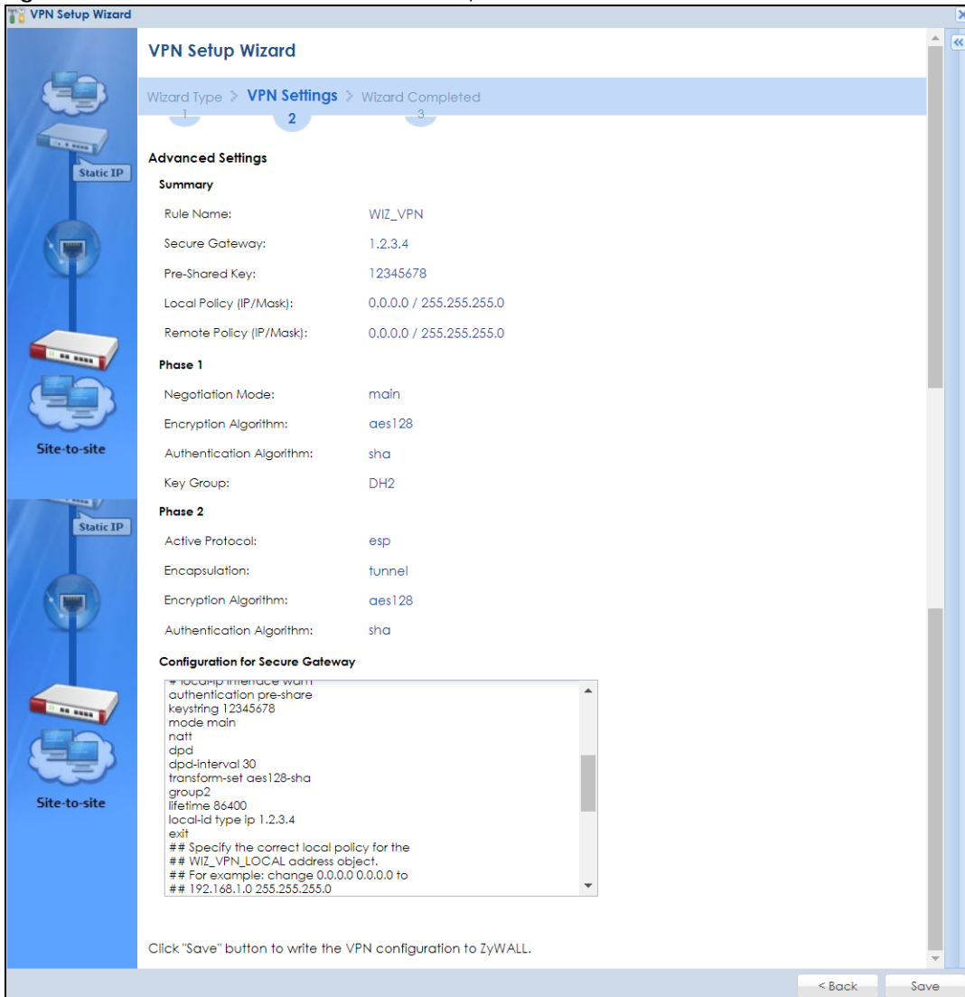
Figure 136 VPN Advanced Wizard: Summary
