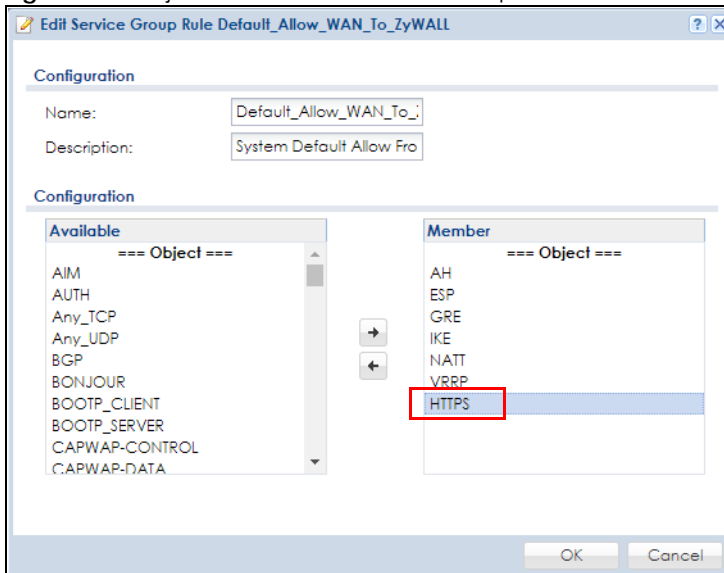
Figure 74 Object &gt; Service &gt; Service Group - HTTPS
