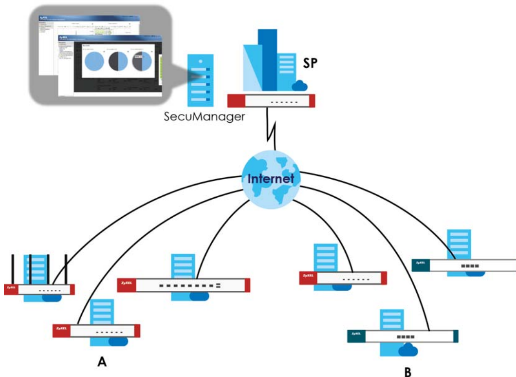
Figure 417 Cloud CNM SecuManager Example Network Topology
