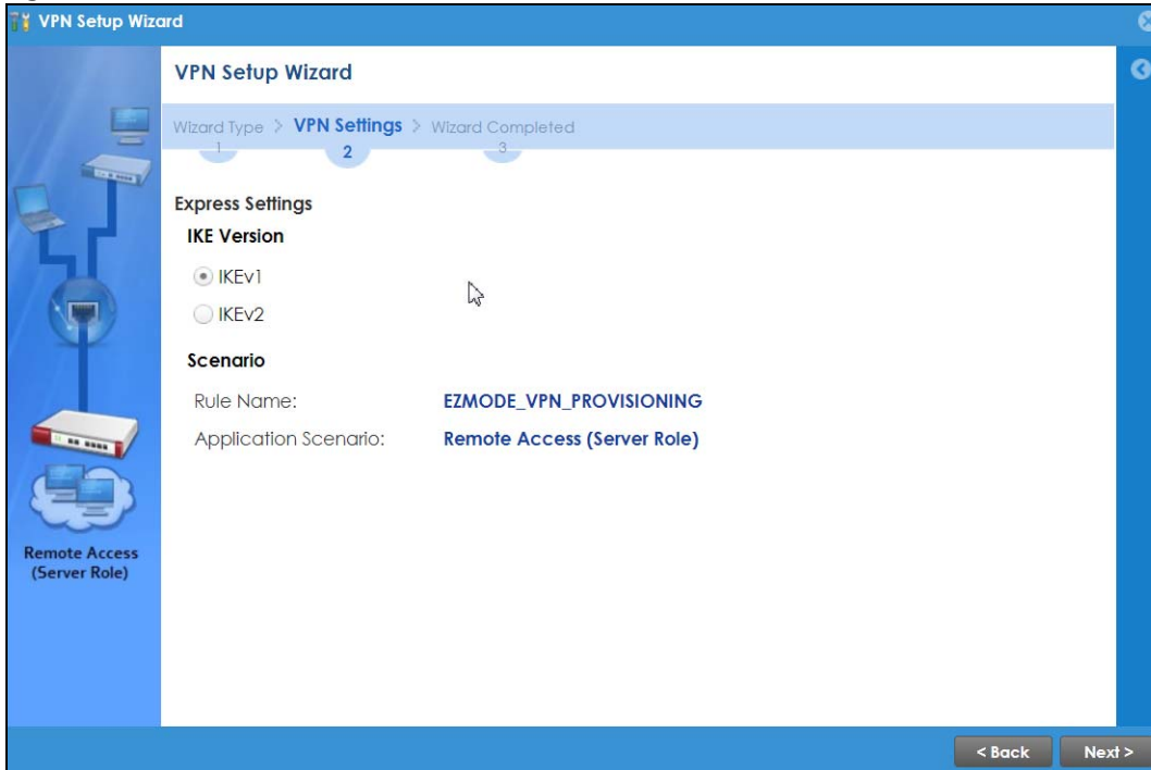
Figure 95 VPN for Configuration Provisioning Advanced Wizard: Scenario Settings
