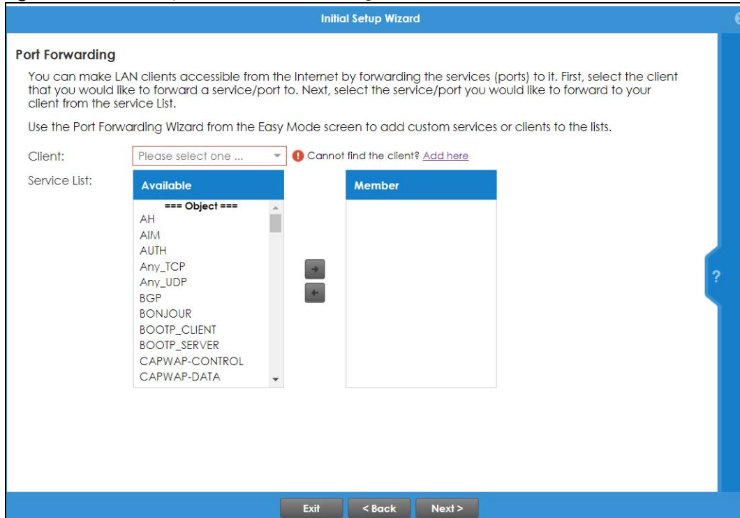
Figure 77 Initial Setup Wizard Port Forwarding
