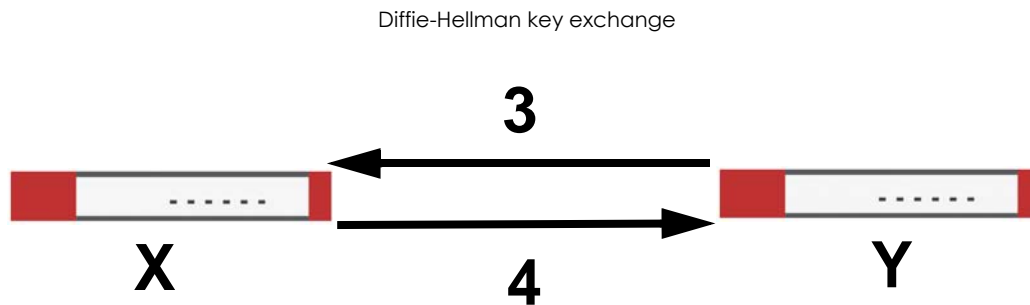
Figure 439 IKE SA: Main Negotiation Mode, Steps 3 - 4: DH Key Exchange
