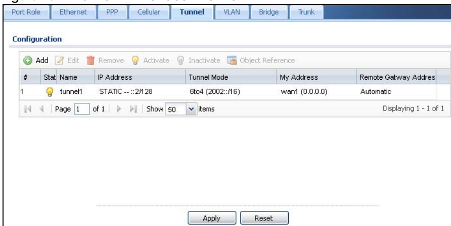
Figure 262 Network &gt; Interface &gt; Tunnel
