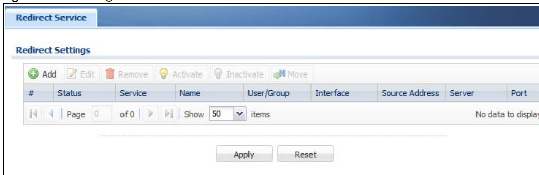
Figure 312 Configuration > Network > Redirect Service
