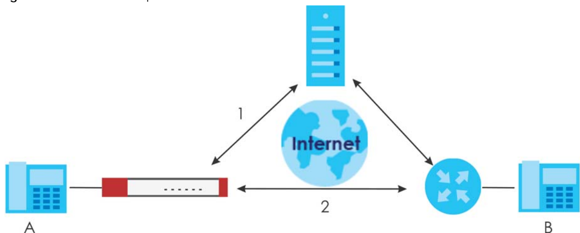
Figure 314 SIP ALG Example
