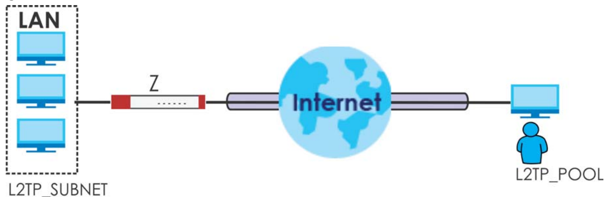
Figure 479 Policy Route for L2TP VPN
