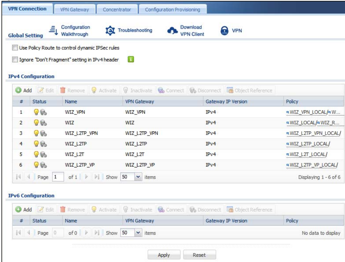
Figure 430 Configuration > VPN > IPsec VPN > VPN Connection
