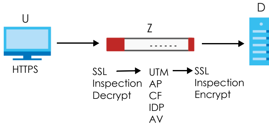
Figure 529 SSL Inspection Overview
