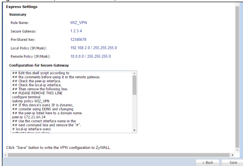
Figure 131 VPN Express Wizard: Summary
