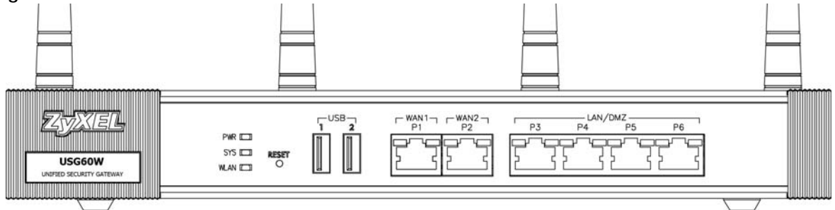
Figure 50 USG2200-VPN Front Panel
