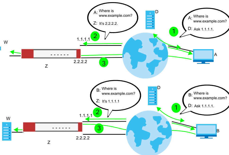
Figure 347 DNS Load Balancing Example
