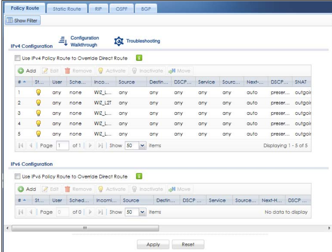
Figure 283 Configuration &gt; Network &gt; Routing &gt; Policy Route
