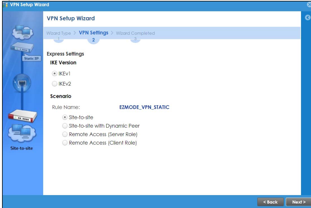
Figure 81 VPN Express Wizard: Scenario
