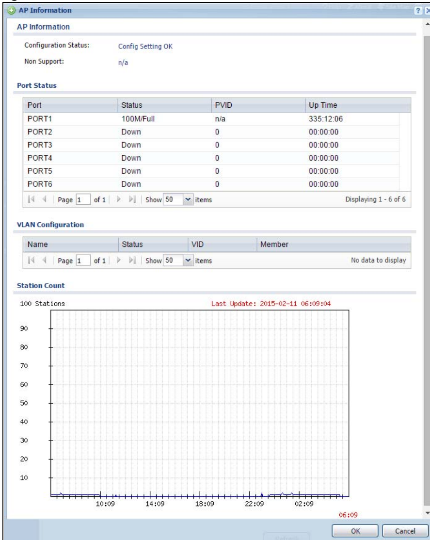
Figure 184 Monitor > Wireless > AP Information > AP List > More Information
