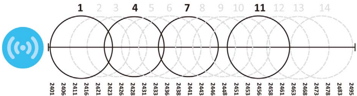
Figure 237 An Example Four-Channel Deployment
