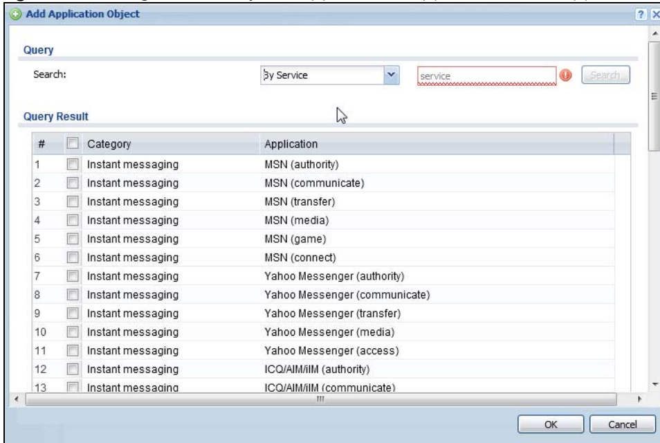
Figure 579 Configuration > Object > Application > Application > Add Application Rule > Add By Service
