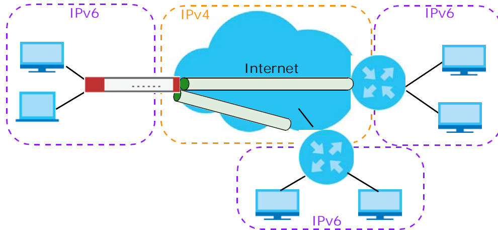
Figure 259 6to4 Tunnel
