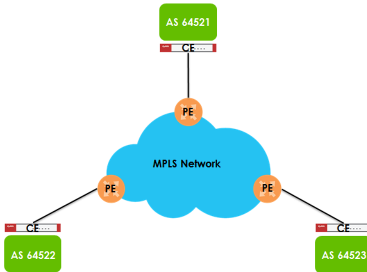
Figure 299 Scenario 1: CE Router - to - MPLS
