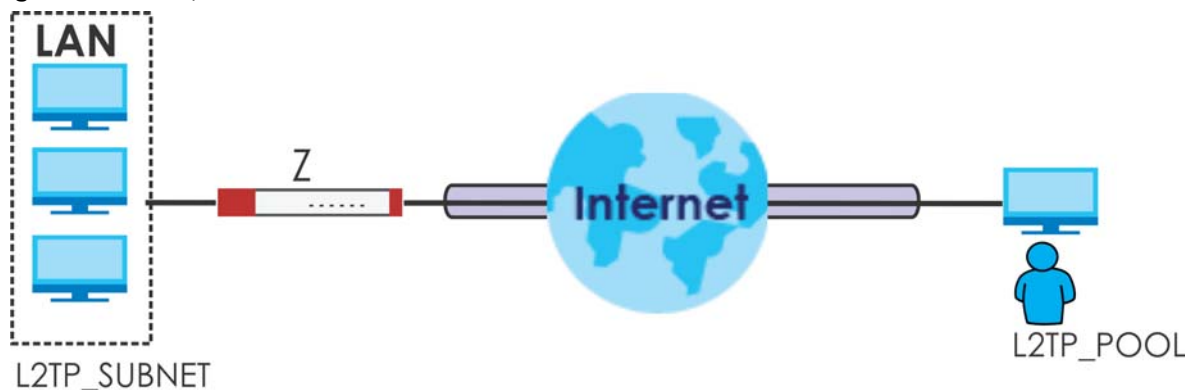
Figure 374 Policy Route for L2TP VPN
