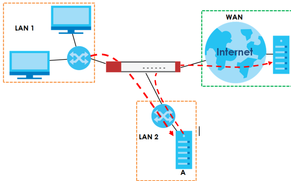
Figure 310 SMTP Redirect Example
