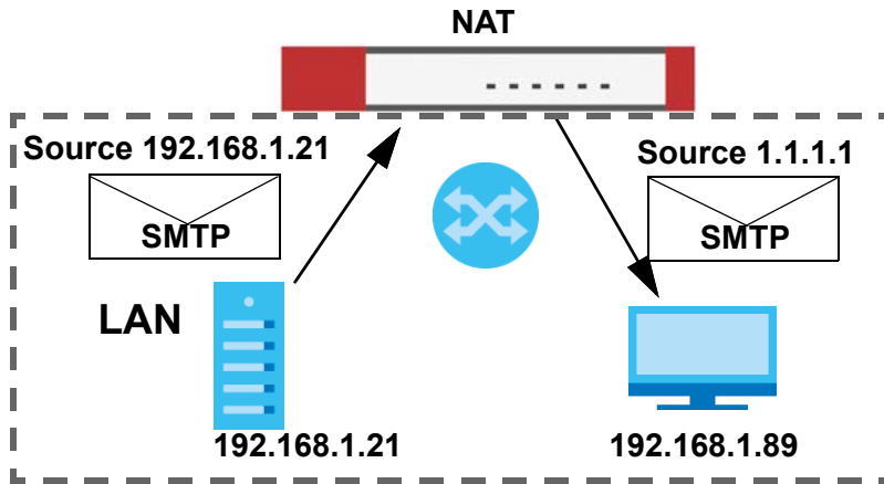
Figure 308 LAN to LAN Return Traffic
