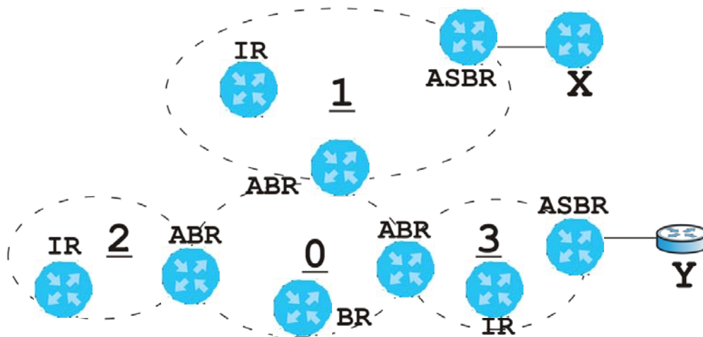
Figure 290 OSPF: Types of Routers
