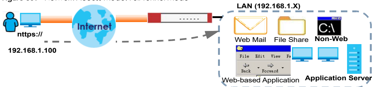
Figure 369 Network Access Mode: Full Tunnel Mode
