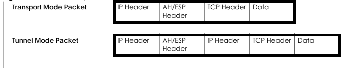
Figure 366 VPN: Transport and Tunnel Mode Encapsulation
