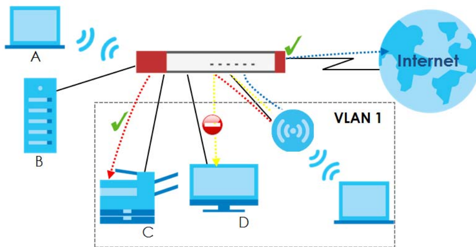
Figure 342 Layer-2 Isolation Application
