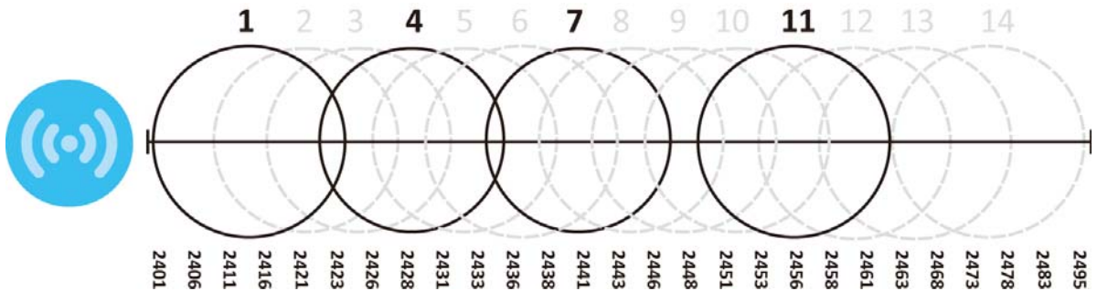
Figure 236 An Example Four-Channel Deployment
