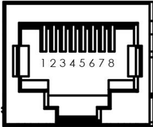
Figure 66 RJ-45 Connector Pins
