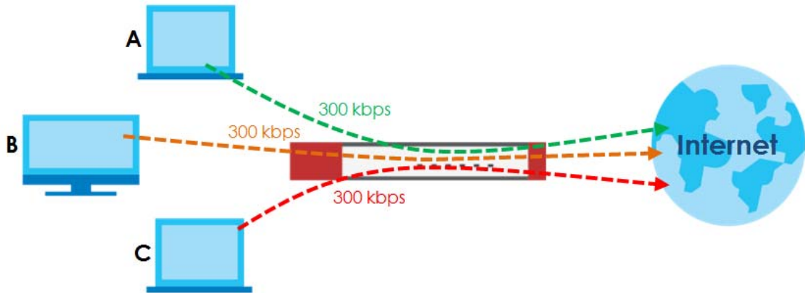
Figure 377 Bandwidth Management Per User Type
