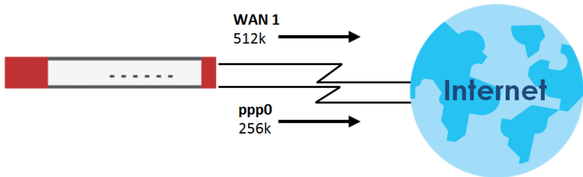
Figure 274 Load Balancing Least Load First Example
