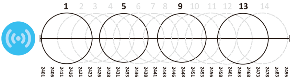
Figure 237 An Alternative Four-Channel Deployment
