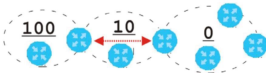
Figure 291 OSPF: Virtual Link
