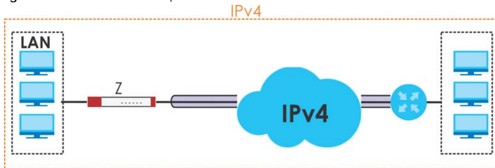
Figure 259 GRE Tunnel Example
