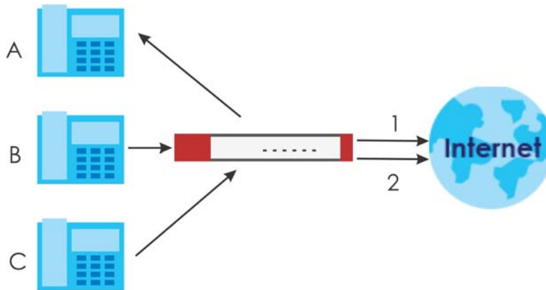
Figure 315 VoIP Calls from the WAN with Multiple Outgoing Calls
