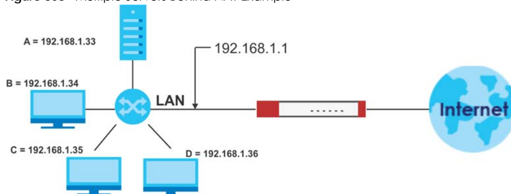
Figure 303 Multiple Servers Behind NAT Example
