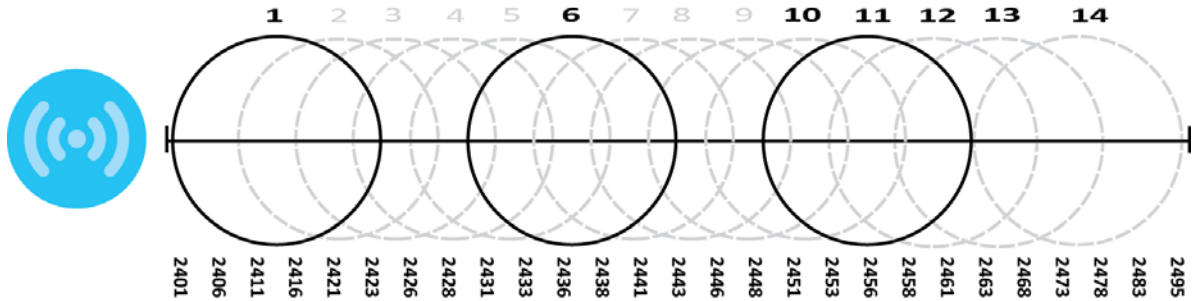
Figure 235 An Example Three-Channel Deployment
