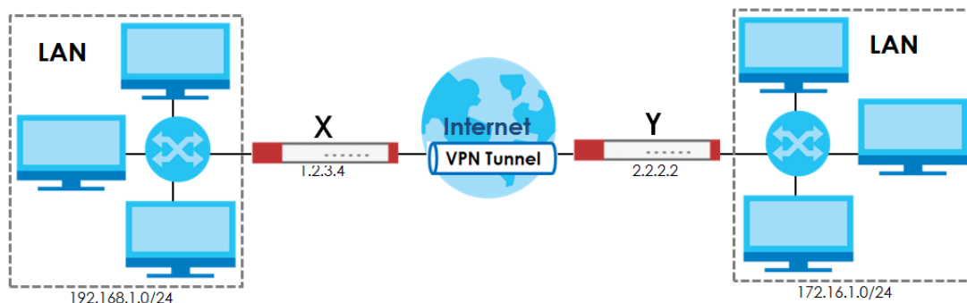
Figure 368 Site-to-site IPsec VPN Example
