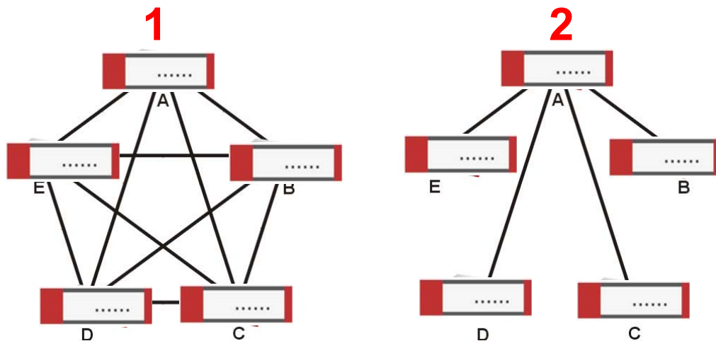
Figure 358 VPN Topologies (Fully Meshed and Hub and Spoke)
