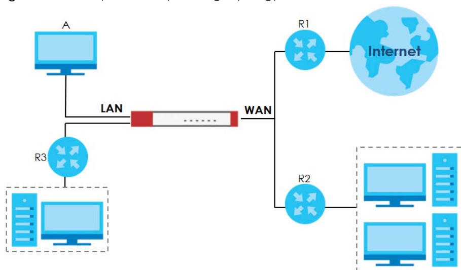
Figure 281 Example of Policy Routing Topology
