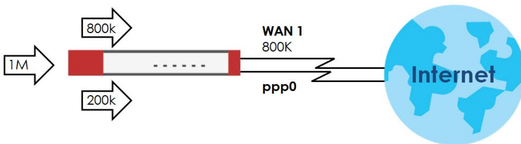
Figure 276 Spillover Algorithm Example
