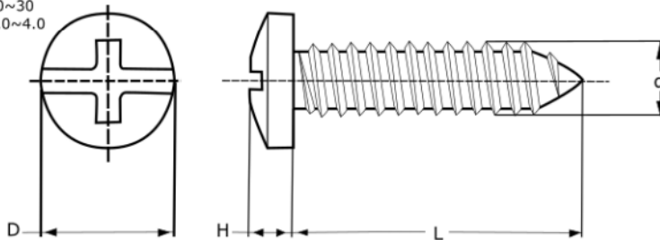
Figure 69 Wall Mounting Screw Specifications
