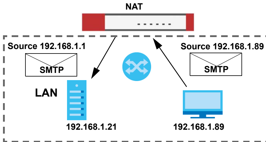
Figure 307 LAN to LAN Traffic
