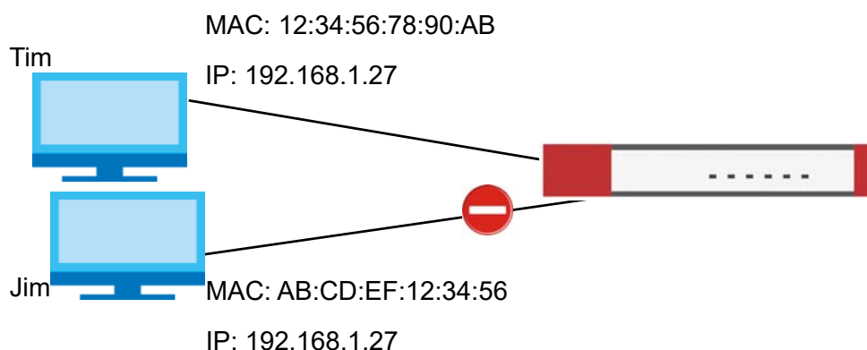
Figure 337 IP/MAC Binding Example
