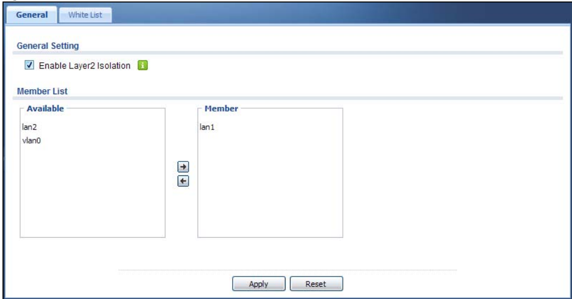
Figure 357 Configuration > Network > Layer 2 Isolation
