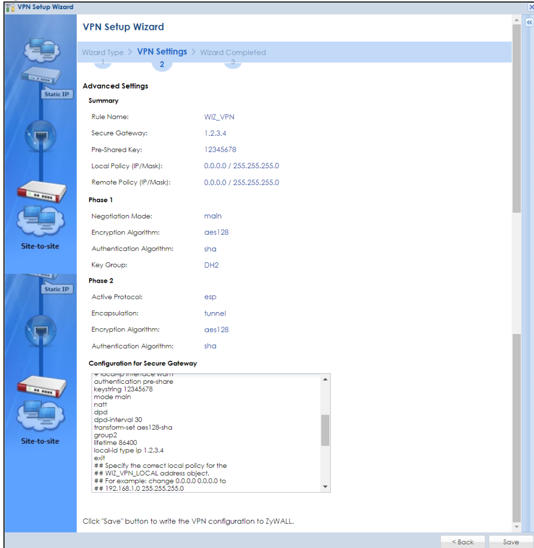
Figure 148 VPN Advanced Wizard: Summary
