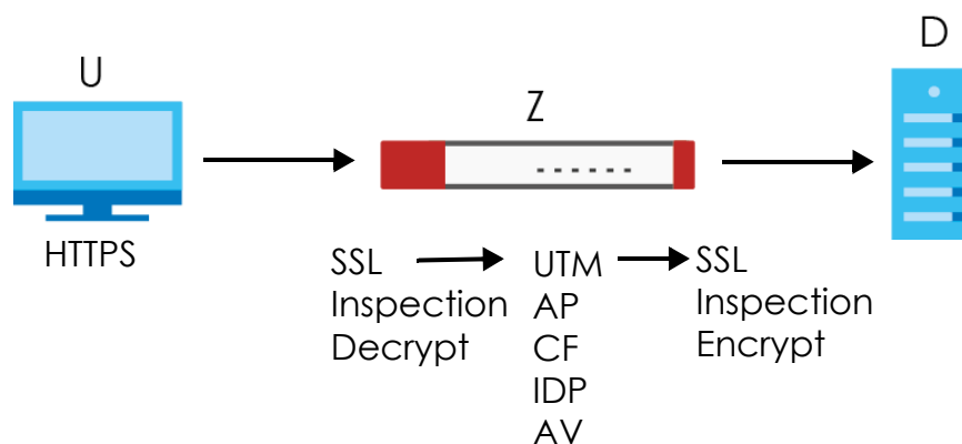
Figure 538 SSL Inspection Overview
