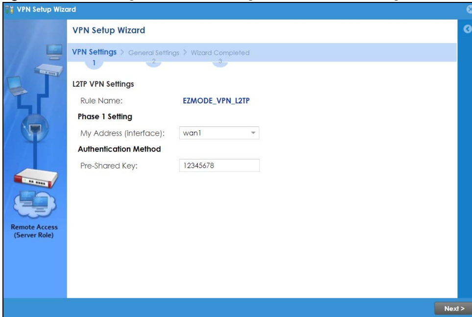
Figure 104 VPN Settings for L2TP VPN Settings Wizard: L2TP VPN Settings
