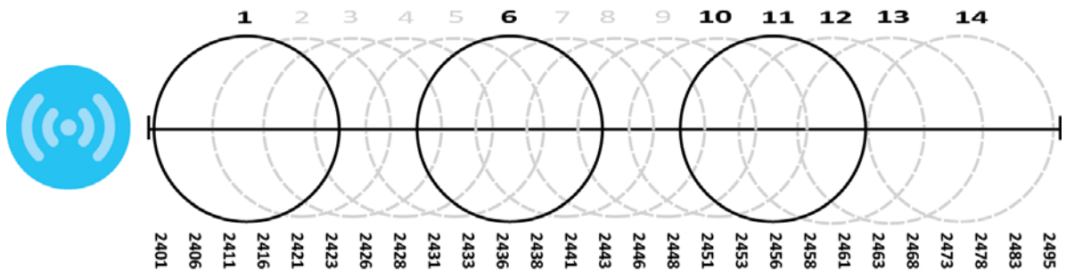
Figure 250 An Example Three-Channel Deployment
