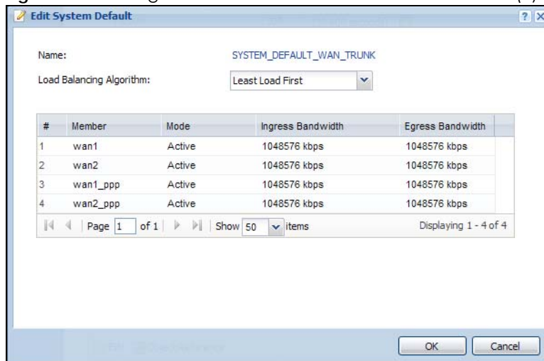
Figure 293 Configuration &gt; Network &gt; Interface &gt; Trunk &gt; Edit (System Default)
