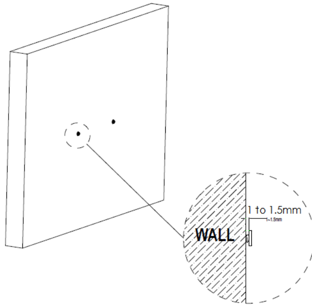
Figure 62 Gap for Cables
