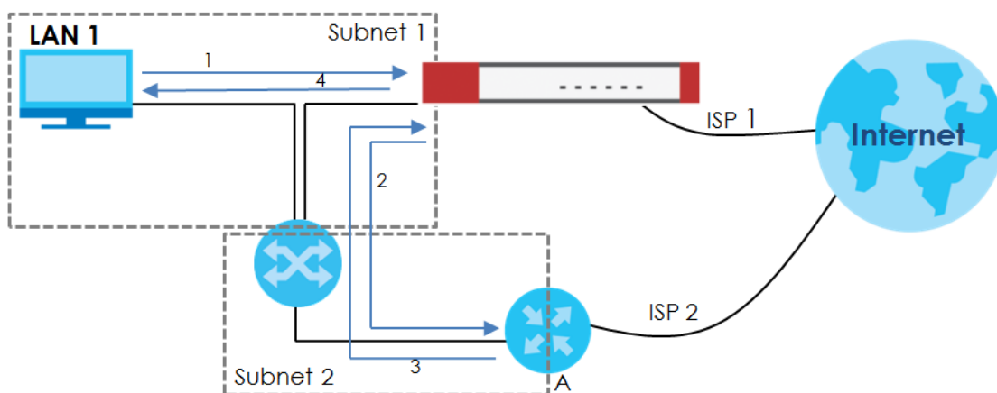
Figure 418 Using Virtual Interfaces to Avoid Asymmetrical Routes
