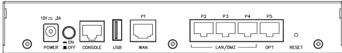
Figure 59 USG60 / USG60W Rear Panel
