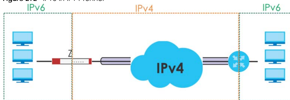
Figure 272 IPv6-in-IPv4 Tunnel
