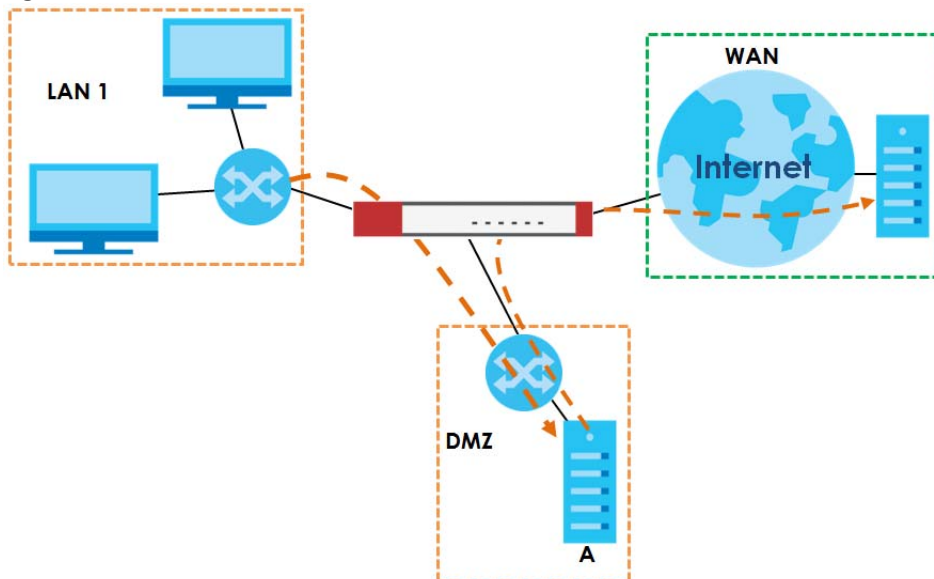
Figure 322 HTTP Redirect Example
