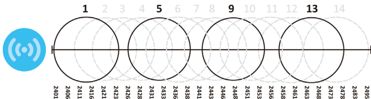
Figure 242 An Alternative Four-Channel Deployment
