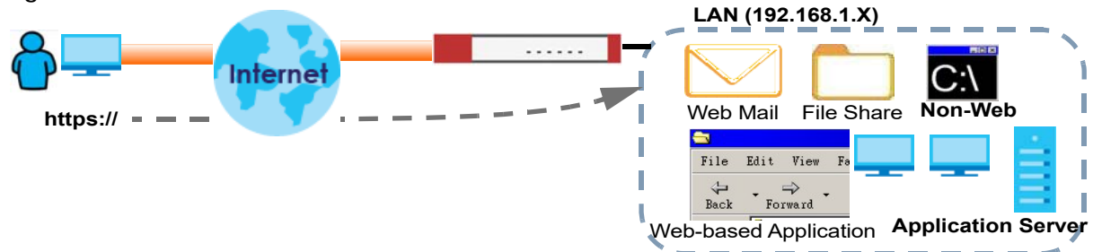
Figure 362 SSL VPN
