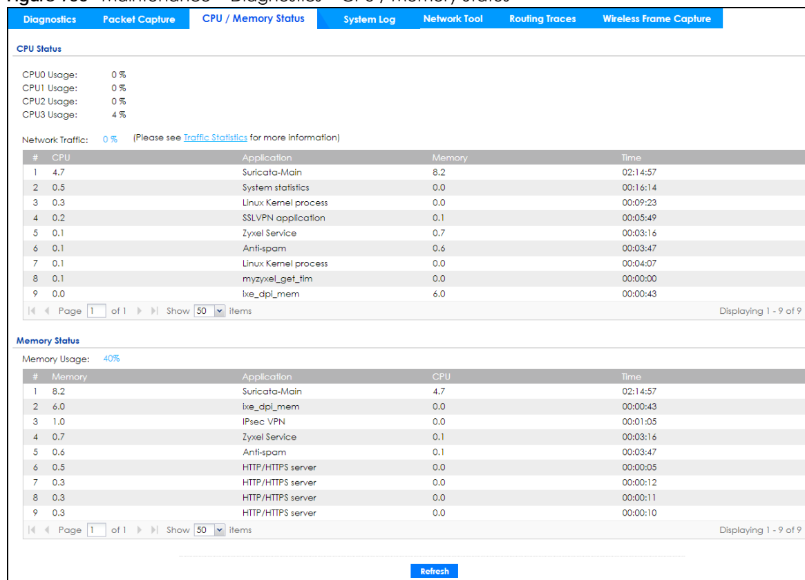
Figure 756 Maintenance > Diagnostics > CPU / Memory Status
