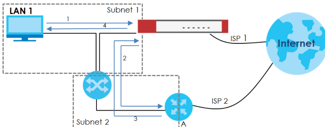
Figure 455 Using Virtual Interfaces to Avoid Asymmetrical Routes
