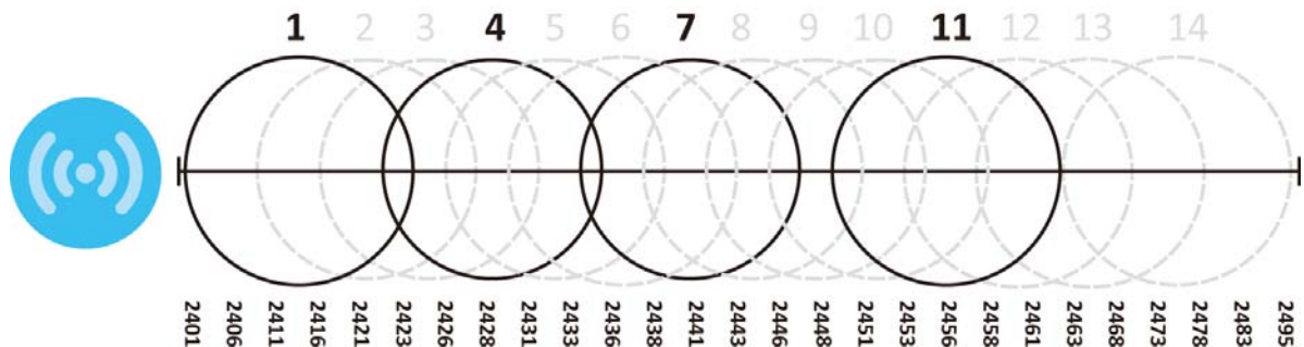
Figure 241 An Example Four-Channel Deployment
