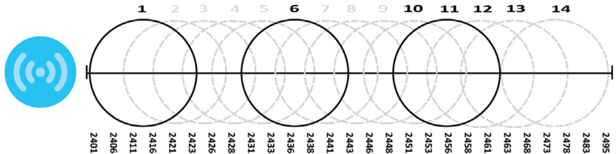
Figure 240 An Example Three-Channel Deployment
