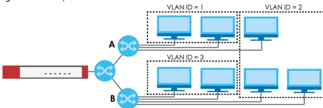
Figure 270 Example: After VLAN
