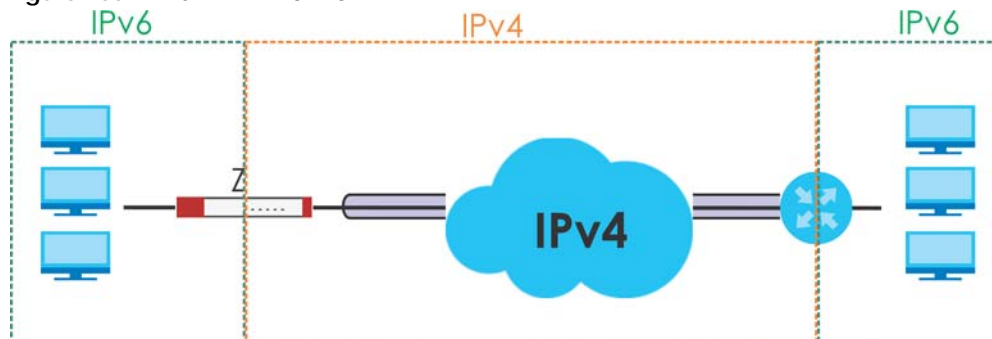
Figure 265 IPv6-in-IPv4 Tunnel
