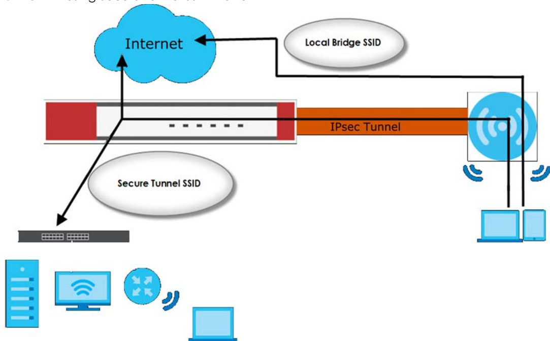
Figure 228 AP Using Secure Tunnel SSID Profile
