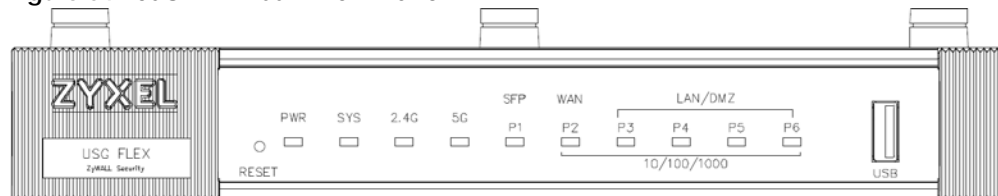
Figure 64 USG FLEX 100W Front Panel
