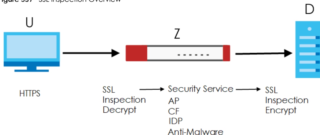
Figure 537 SSL Inspection Overview
