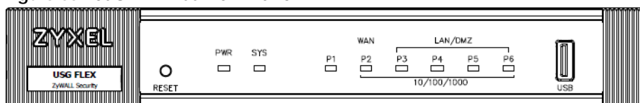
Figure 66 USG FLEX 100W Front Panel
