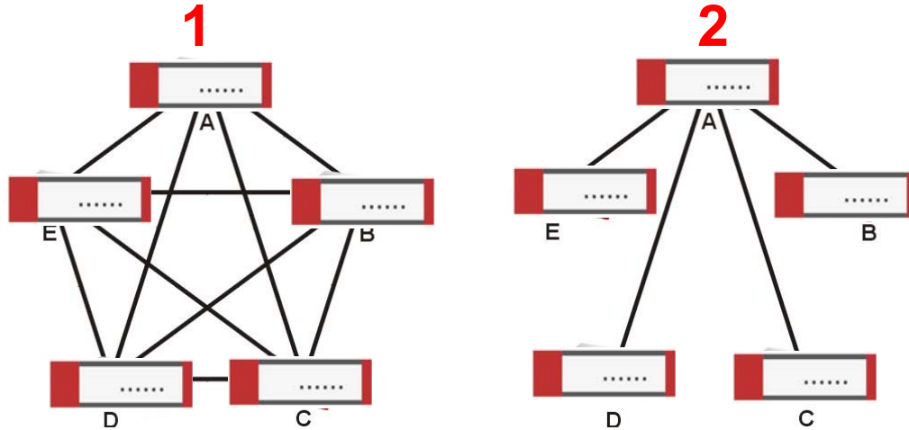
Figure 364 VPN Topologies (Fully Meshed and Hub and Spoke)
