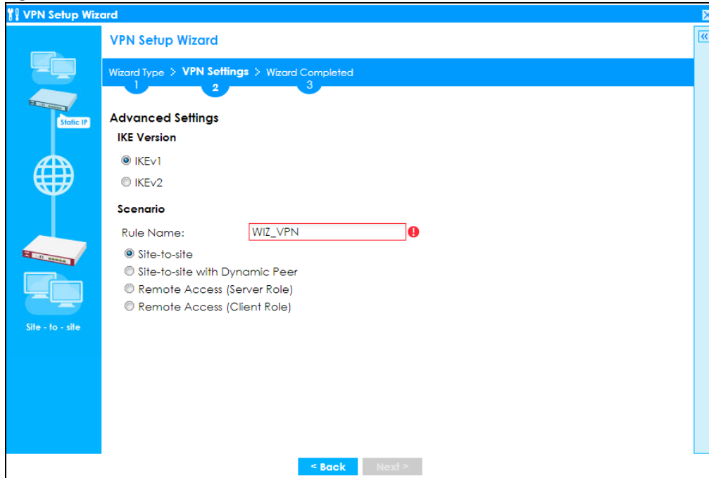
Figure 106 VPN Advanced Wizard: Scenario
