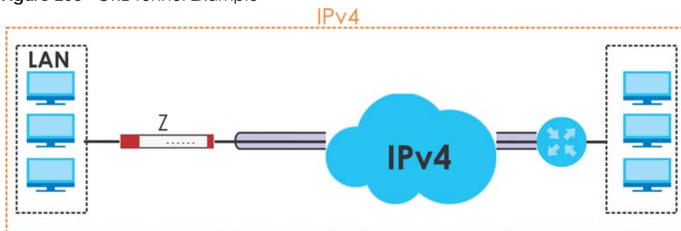
Figure 258 GRE Tunnel Example
