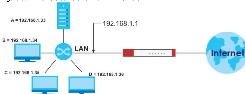
Figure 304 Multiple Servers Behind NAT Example
