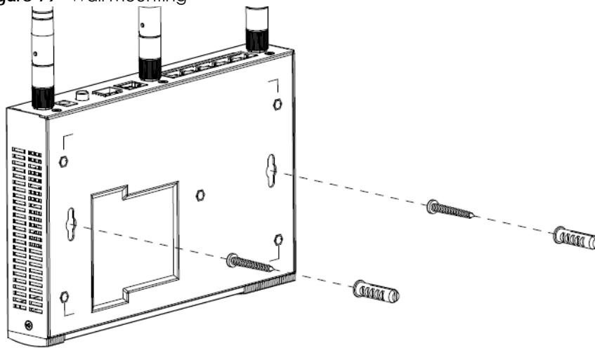
Figure 79 Wall Mounting
