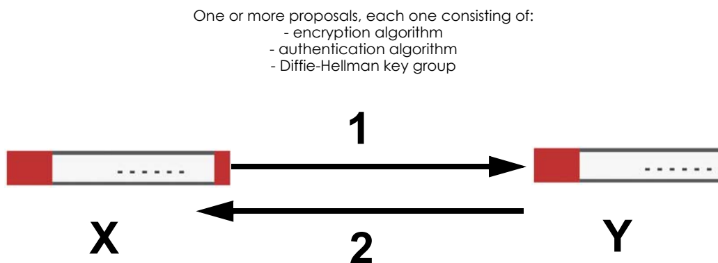
Figure 368 IKE SA: Main Negotiation Mode, Steps 1 - 2: IKE SA Proposal
