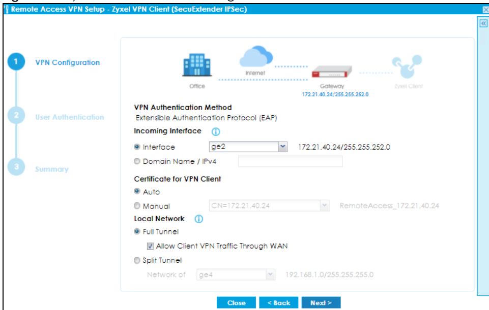
Figure 89 Zyxel VPN Client: VPN Configuration
