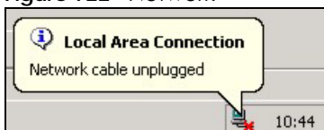
Figure 722 Network
