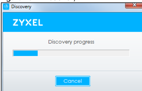
Figure 701 Discovery
