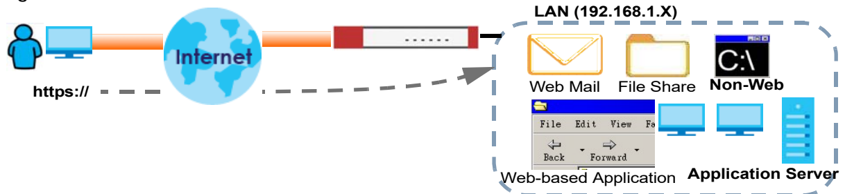
Figure 359 SSL VPN
