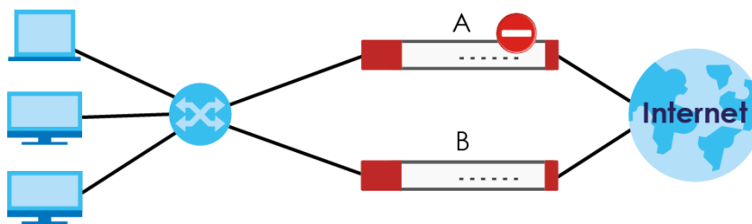
Figure 632 Device HA Backup Taking Over for the Master
