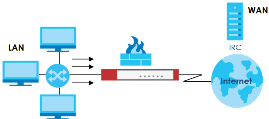
Figure 464 Blocking All LAN to WAN IRC Traffic Example
