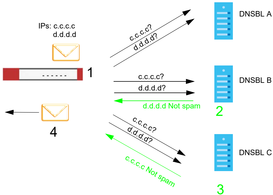
Figure 533 DNSBL Legitimate Email Detection Example
