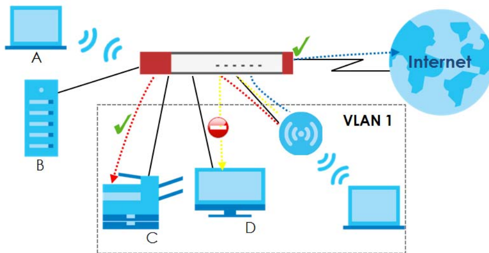
Figure 350 Layer-2 Isolation Application
