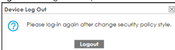
Figure 505 Logout Prompt
