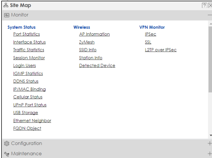
Figure 22 Site Map
