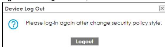
Figure 490 Logout Prompt
