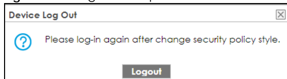
Figure 531 Logout Prompt
