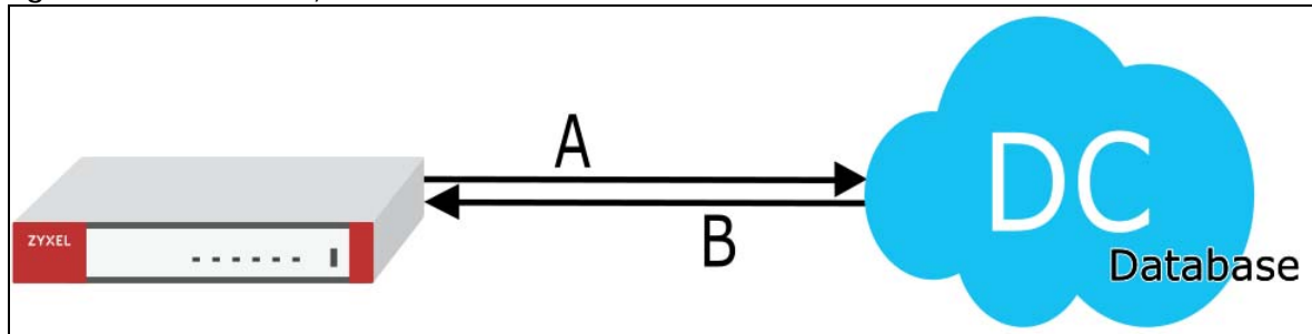
Figure 484 Cloud Query
