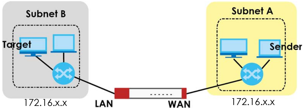
Figure 249 Proxy ARP
