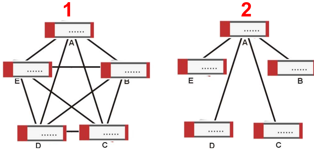
Figure 366 VPN Topologies (Fully Meshed and Hub and Spoke)
