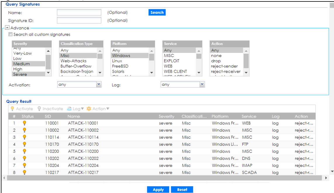
Figure 509 Query Example Search
