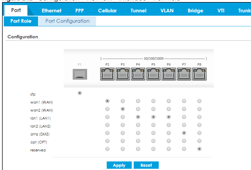
Figure 242 Configuration > Network > Interface > Port Role
