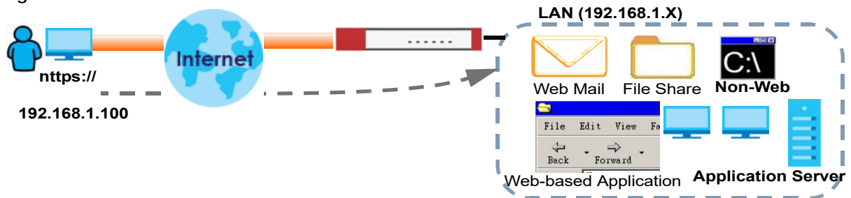
Figure 377 Network Access Mode: Full Tunnel Mode
