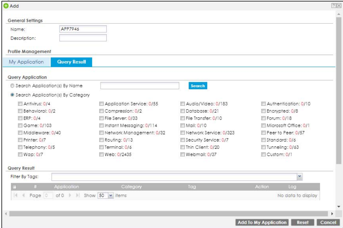
Figure 471 Configuration > Security Service > App Patrol > Add/Edit > Query Result
