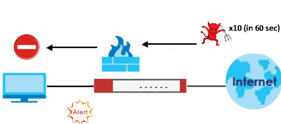
Figure 507 Rate Based Signatures Example
