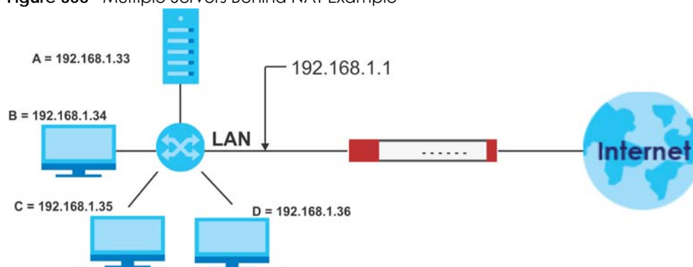
Figure 306 Multiple Servers Behind NAT Example
