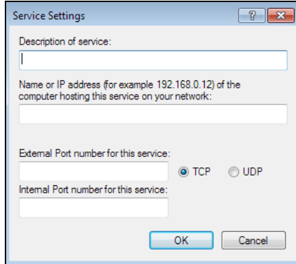
Figure 330 Internet Connection Properties: Advanced Settings: Add
