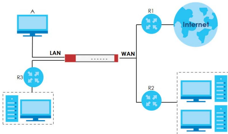
Figure 284 Example of Policy Routing Topology
