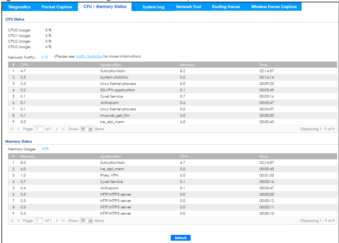
Figure 734 Maintenance > Diagnostics > CPU / Memory Status
