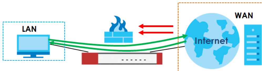
Figure 448 Default Directional Security Policy Example
