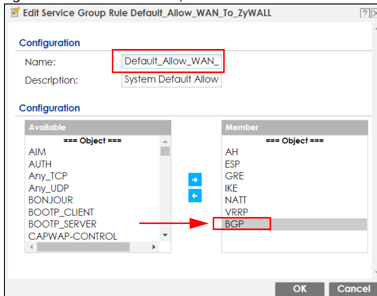
Figure 299 Allow BGP to the Zyxel Device
