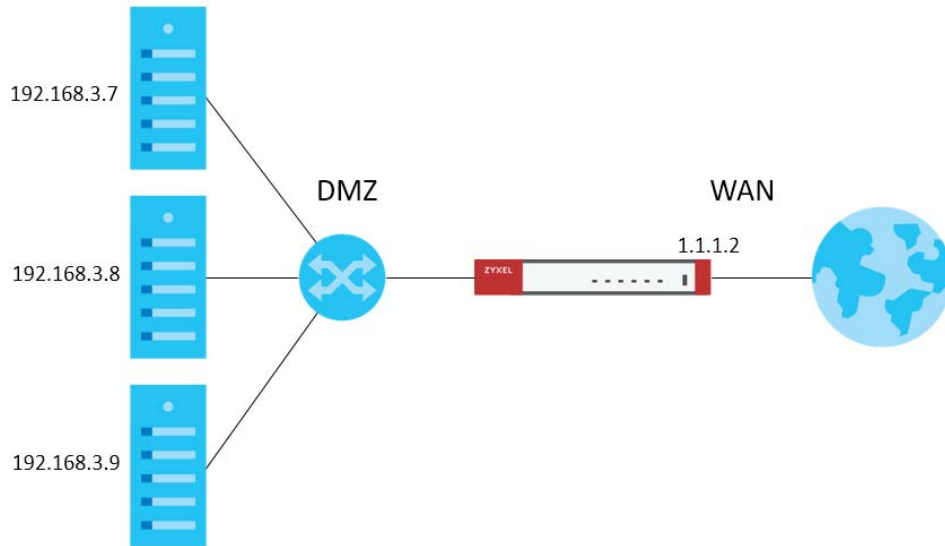
Figure 312 Virtual Server on the WAN- Example 1
