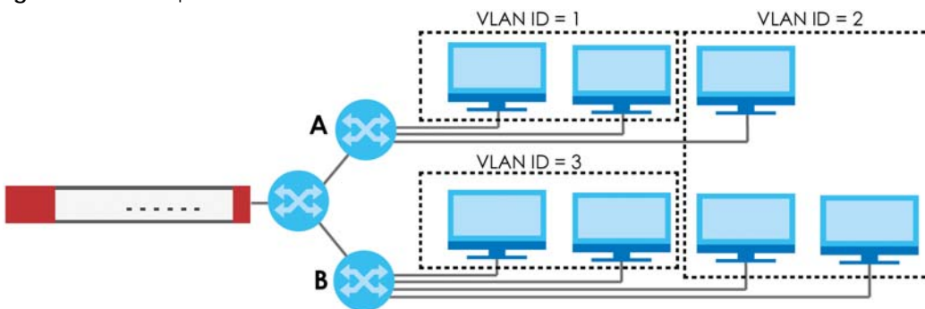
Figure 267 Example: After VLAN
