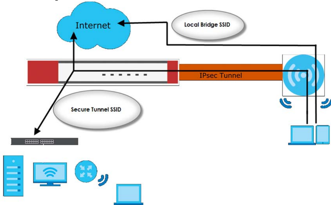
Figure 385 AP Using Secure Tunnel SSID Profile
