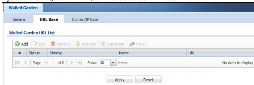
Figure 441 Configuration &gt; Hotspot &gt; Walled Garden: URL Base
