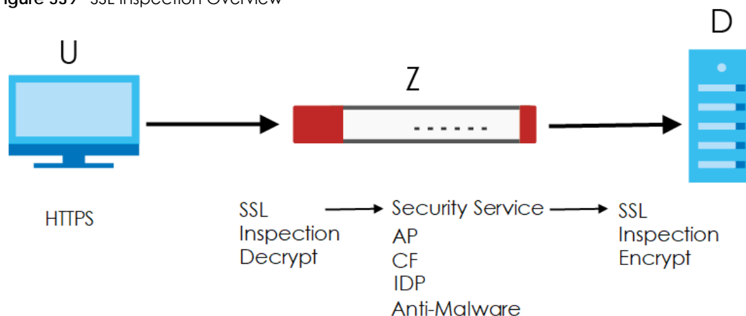
Figure 539 SSL Inspection Overview
