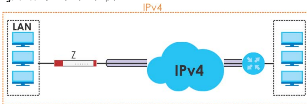
Figure 260 GRE Tunnel Example
