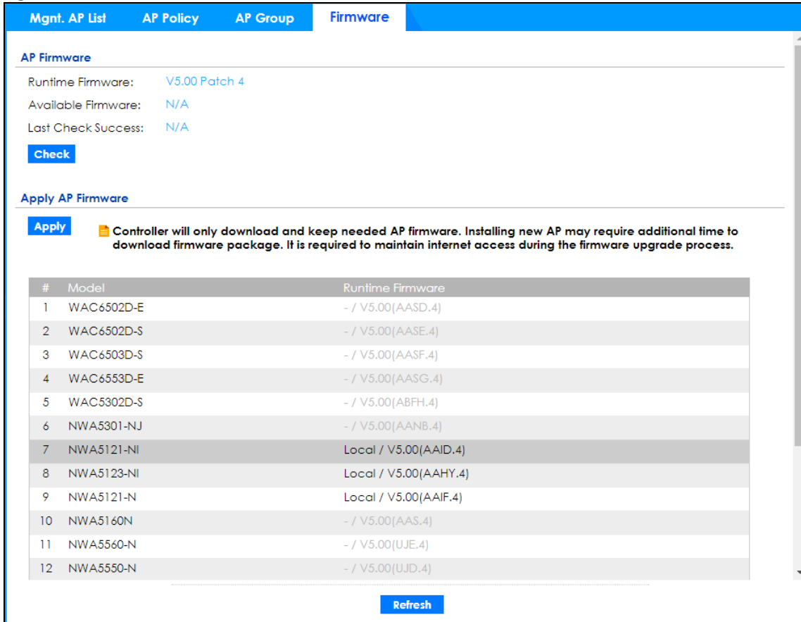
Figure 232 Configuration > Wireless > AP Management > Firmware
