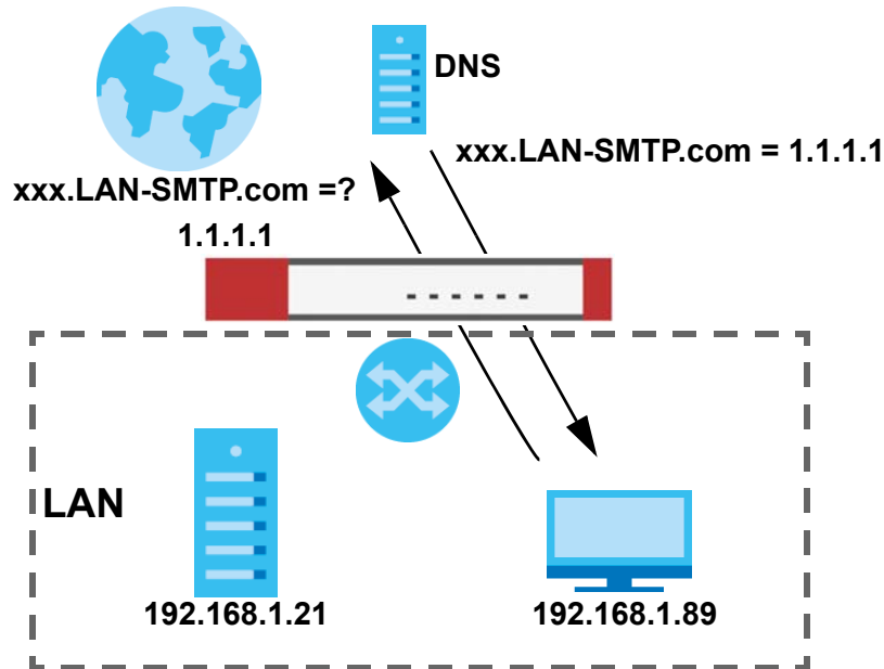
Figure 309 LAN Computer Queries a Public DNS Server
