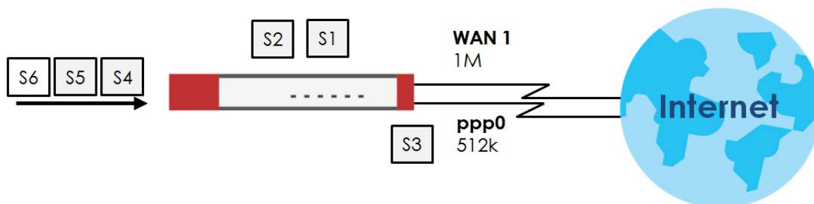
Figure 278 Weighted Round Robin Algorithm Example
