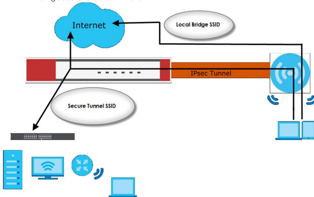
Figure 227 AP Using Secure Tunnel SSID Profile
