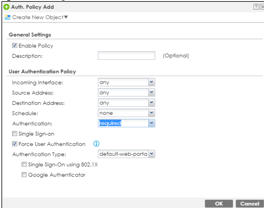
Figure 401 Configuration > Web Authentication > General > Add Authentication Policy
