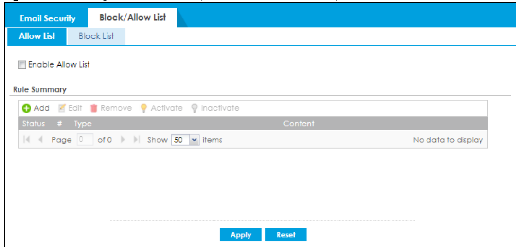
Figure 523 Configuration > Security Service > Email Security > Block/Allow List> Allow List
