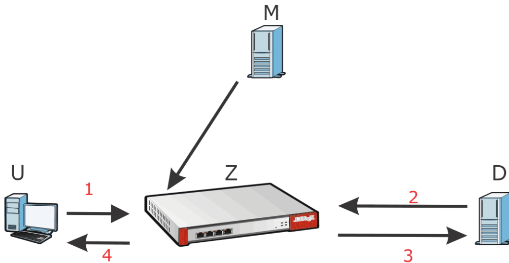
Figure 544 SSL Inspection Certificate Update Overview
