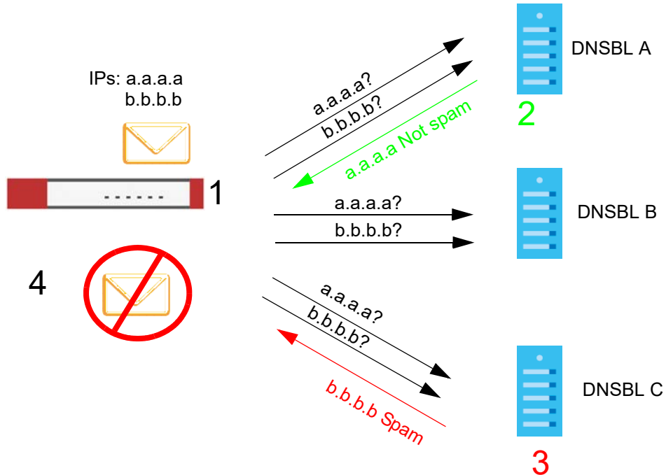
Figure 532 DNSBL Spam Detection Example
