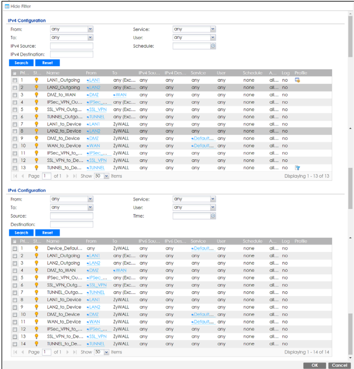
Figure 473 Configuration > Security Service > Content Filter > Action
