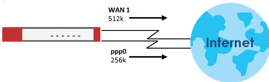
Figure 277 Load Balancing Least Load First Example
