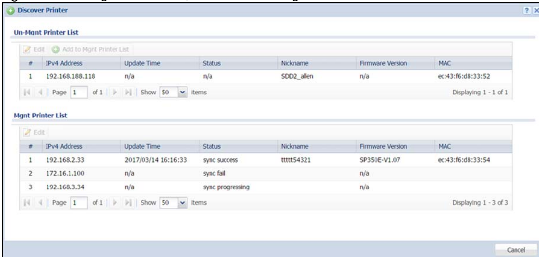
Figure 431 Configuration > Hotspot > Printer Manager > General: Discover Printer
