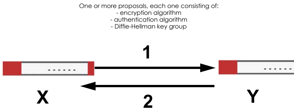
Figure 370 IKE SA: Main Negotiation Mode, Steps 1 - 2: IKE SA Proposal
