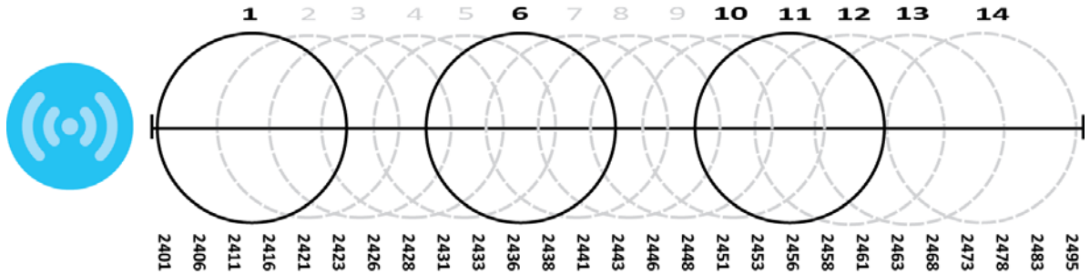
Figure 239 An Example Three-Channel Deployment
