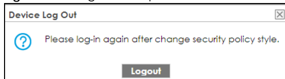
Figure 500 Logout Prompt
