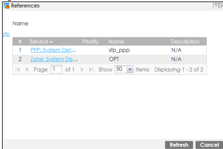
Figure 252 References
