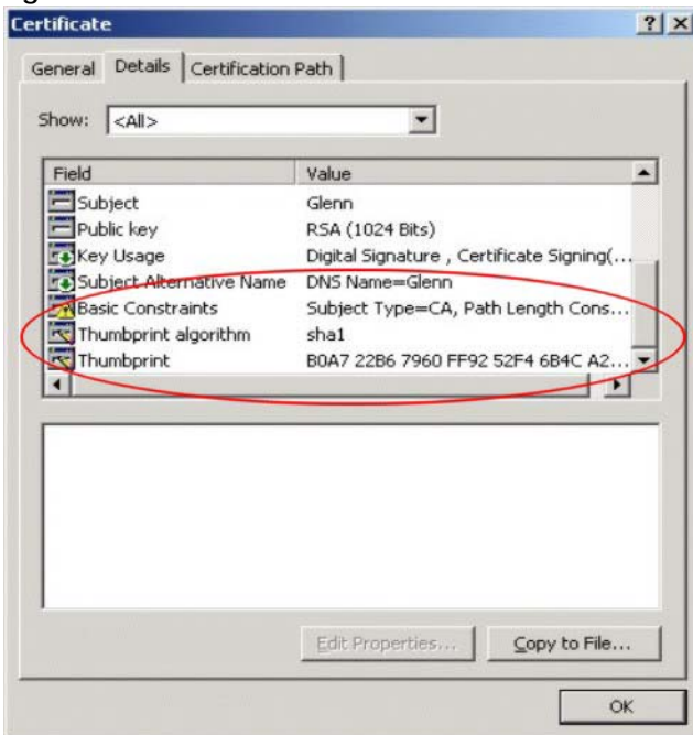
Figure 616 Certificate Details
