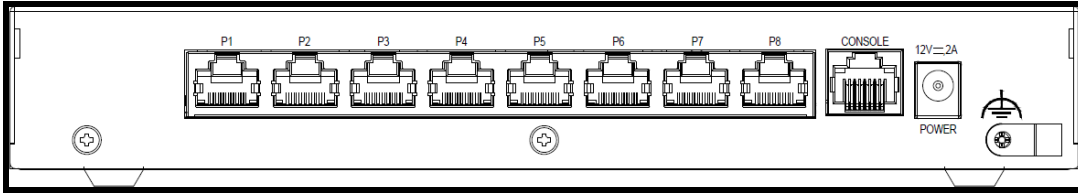
Figure 35 USG FLEX 100HP Rear Panel
