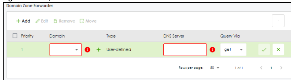
Figure 245 System > DNS & DDNS > DNS > Domain Zone Forwarder > Add
