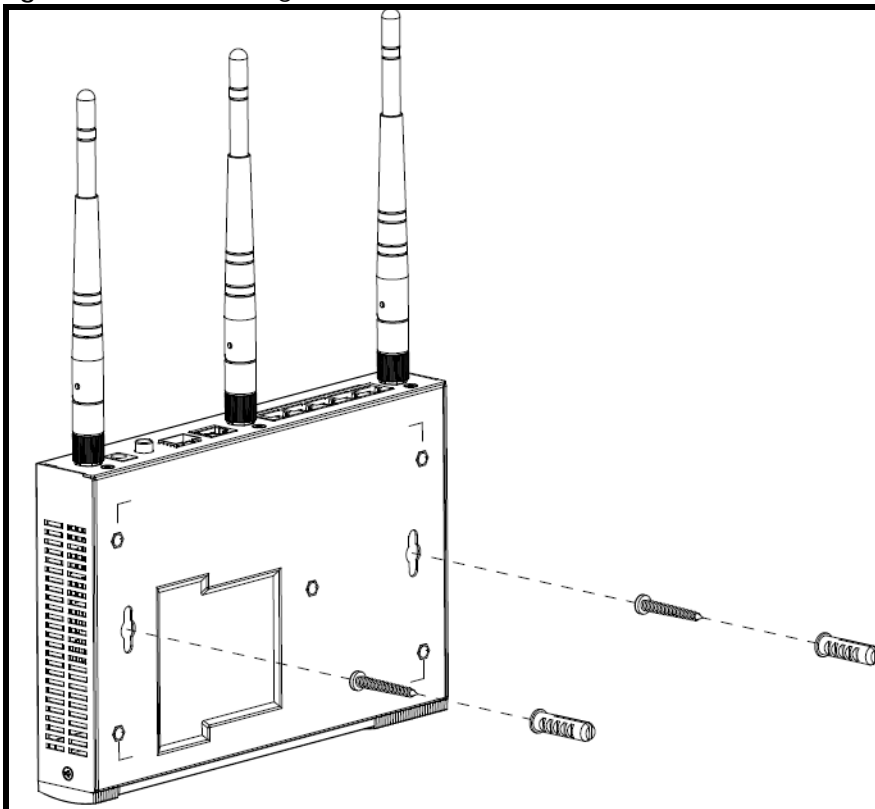
Figure 46 Wall Mounting
