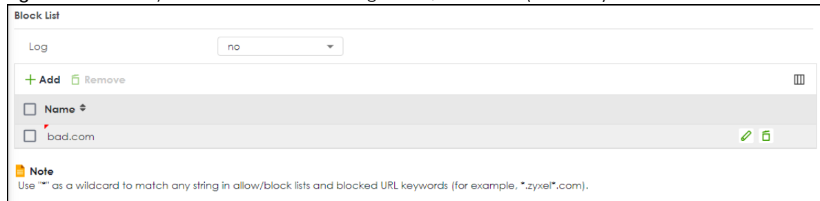
Figure 183 Security Service &gt; Content Filtering &gt; Add/Edit Profile (Block List)
