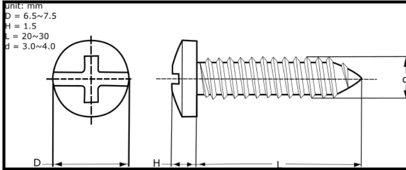
Figure 45 Wall Mounting Screw Specifications
