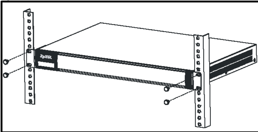
Figure 44 Mount on Rack
