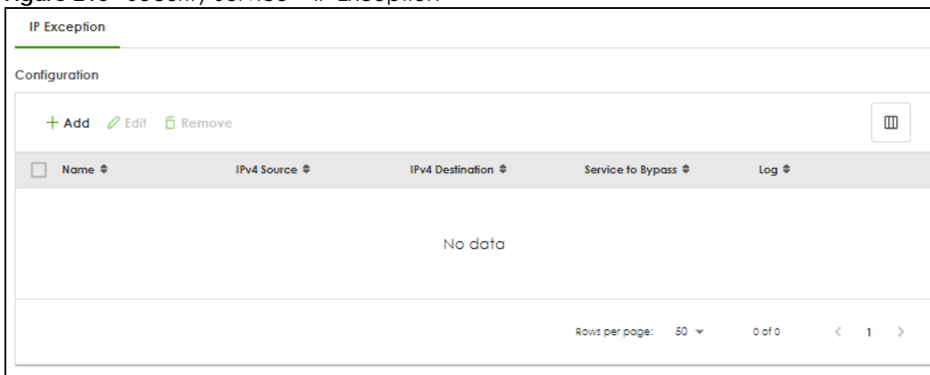
Figure 213 Security Service > IP Exception
