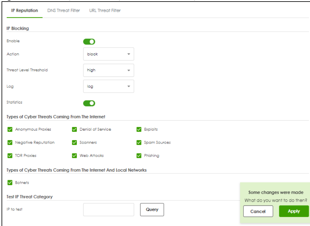
Figure 187 Security Service > Reputation Filter > IP Reputation
