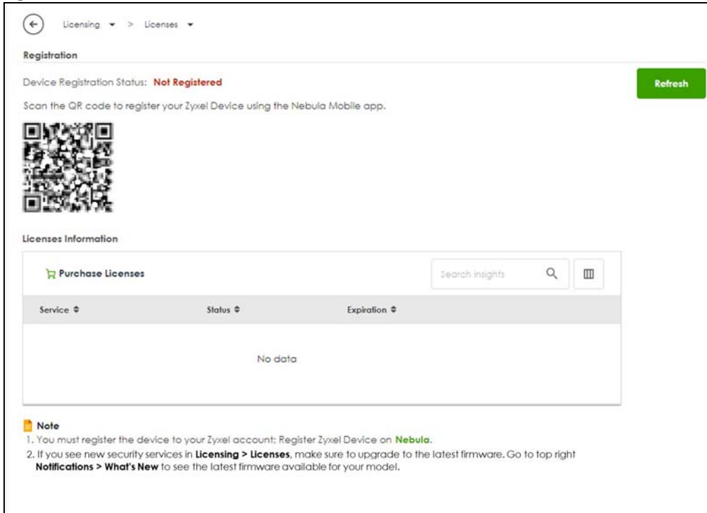
Figure 80 Licensing > Licenses (Not Registered)
