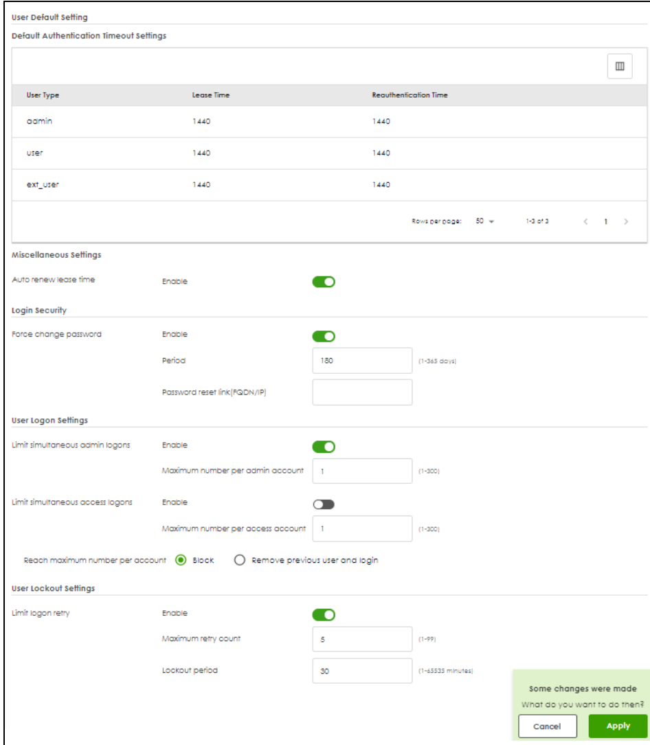
Figure 229 User & Authentication > User/Group > Setting
