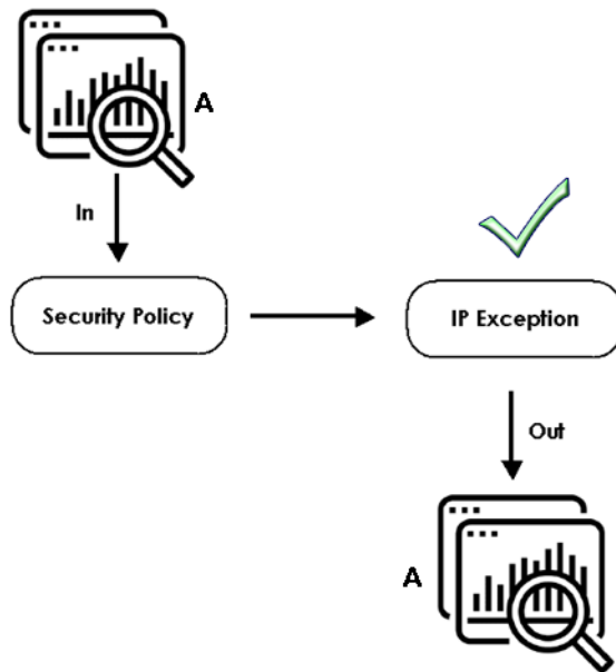
Figure 215 Bypass Security Services Flow
