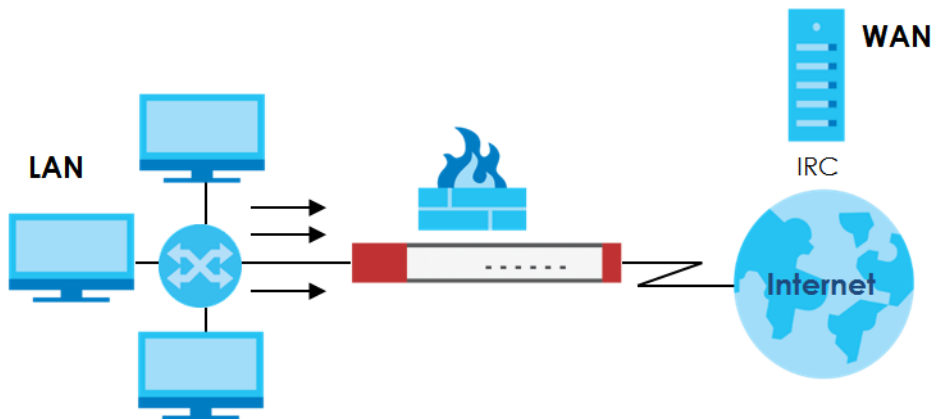
Figure 154 Blocking All LAN to WAN IRC Traffic Example
