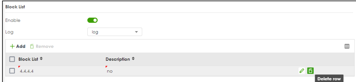
Figure 197 Security Service > Reputation Filter > URL Threat Filter (Block List)
