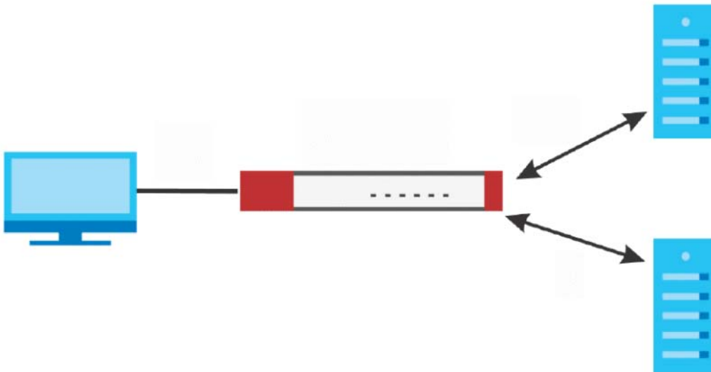
Figure 179 Content Filtering Lookup Procedure
