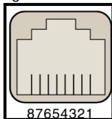
Figure 40 RJ-45 Connector Pins
