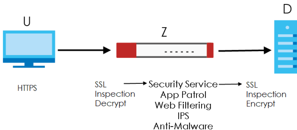
Figure 216 SSL Inspection Overview
