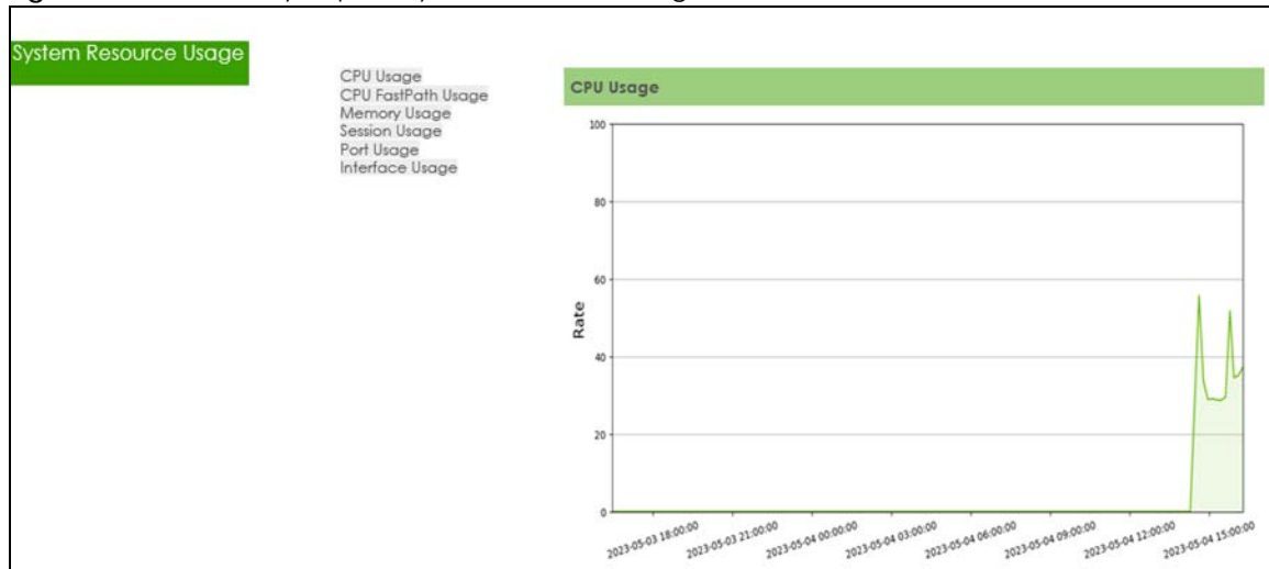
Figure 269 Email Daily Report: System Resource Usage
