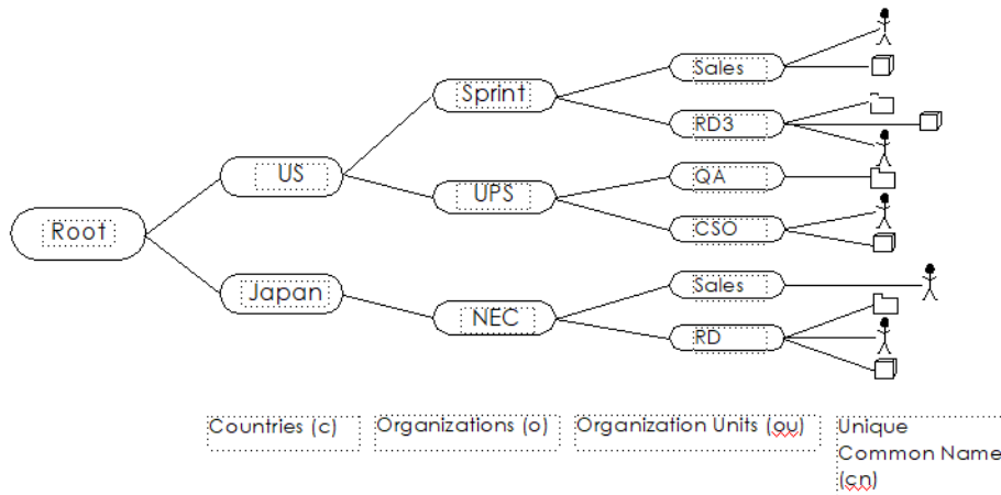
Figure 230 Basic Directory Structure
