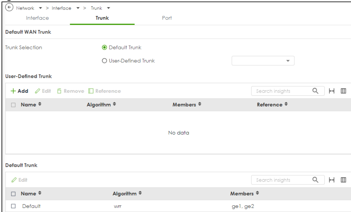
Figure 99 Network > Interface > Trunk
