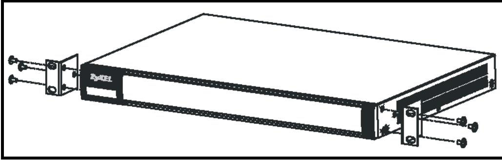
Figure 43 Attach Brackets
