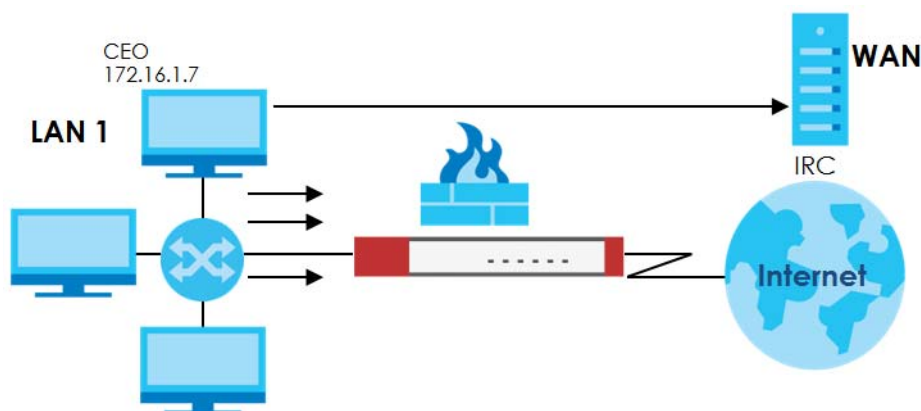
Figure 155 Limited LAN to WAN IRC Traffic Example
