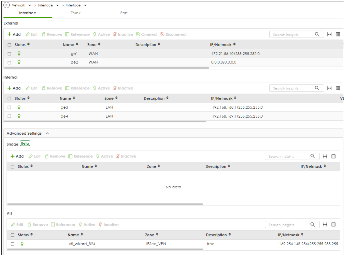
Figure 87 Network > Interface > Interface
