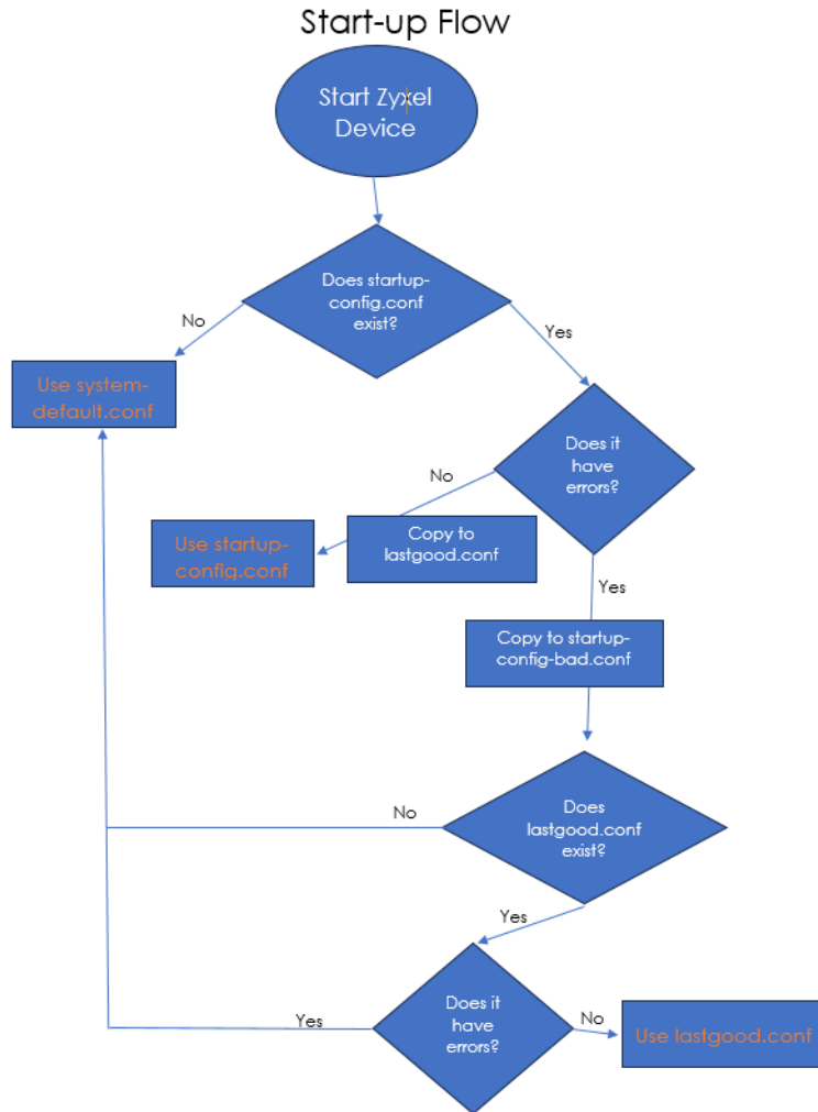
Figure 273 Zyxel Device Start-up Flow
