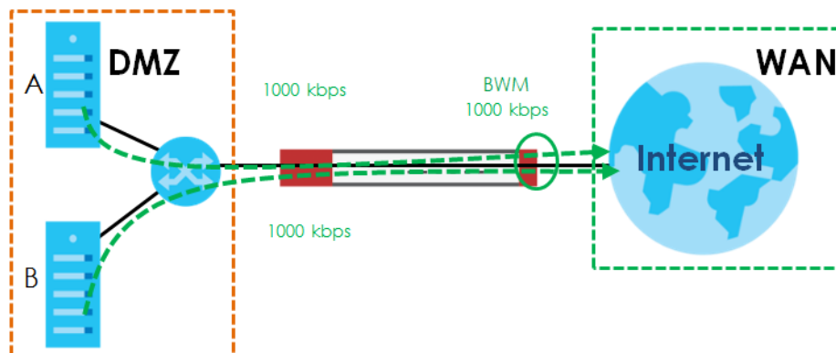
Figure 378 Bandwidth Management Behavior
