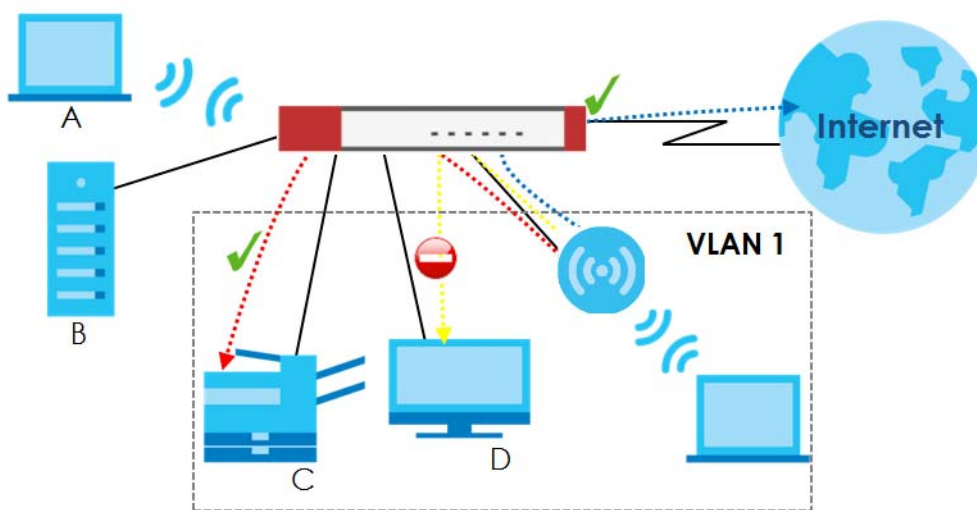
Figure 340 Layer-2 Isolation Application
