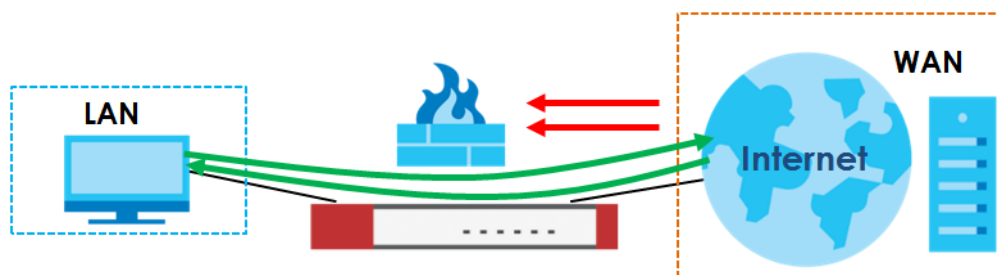
Figure 405 Default Directional Security Policy Example
