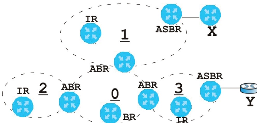
Figure 288 OSPF: Types of Routers
