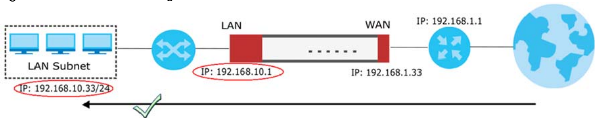
Figure 240 IP Address Change
