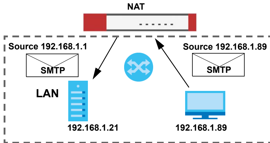
Figure 305 LAN to LAN Traffic
