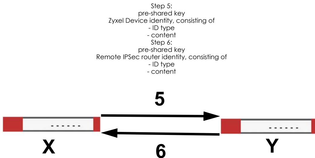
Figure 362 IKE SA: Main Negotiation Mode, Steps 5 - 6: Authentication (continued)
