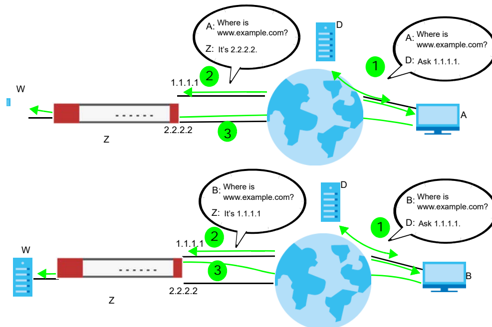
Figure 344 DNS Load Balancing Example
