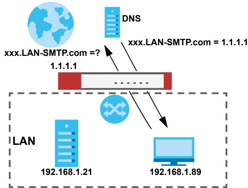
Figure 304 LAN Computer Queries a Public DNS Server
