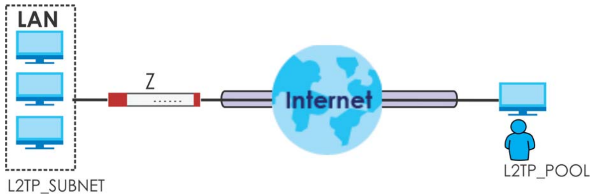
Figure 372 Policy Route for L2TP VPN
