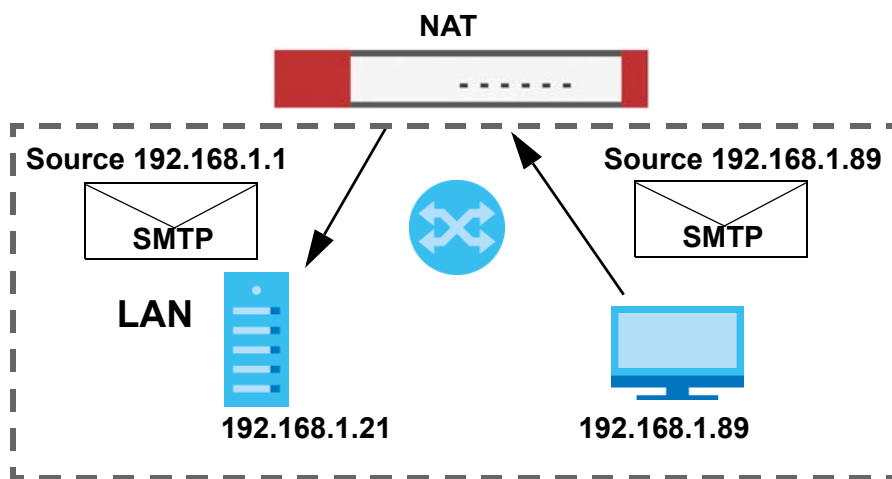
Figure 281 LAN to LAN Traffic
