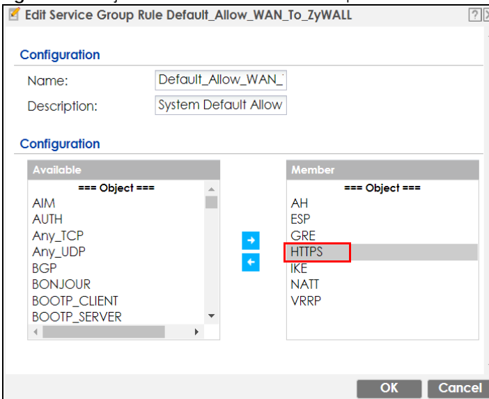
Figure 44 Object &gt; Service &gt; Service Group - HTTPS
