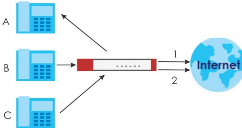
Figure 294 VoIP Calls from the WAN with Multiple Outgoing Calls
