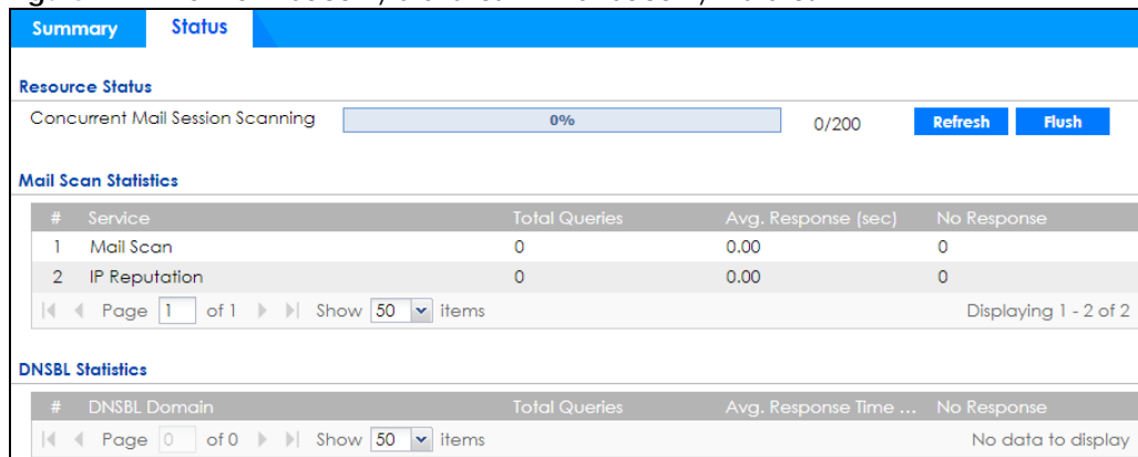
Figure 177 Monitor &gt; Security Statistics &gt; Email Security &gt; Status
