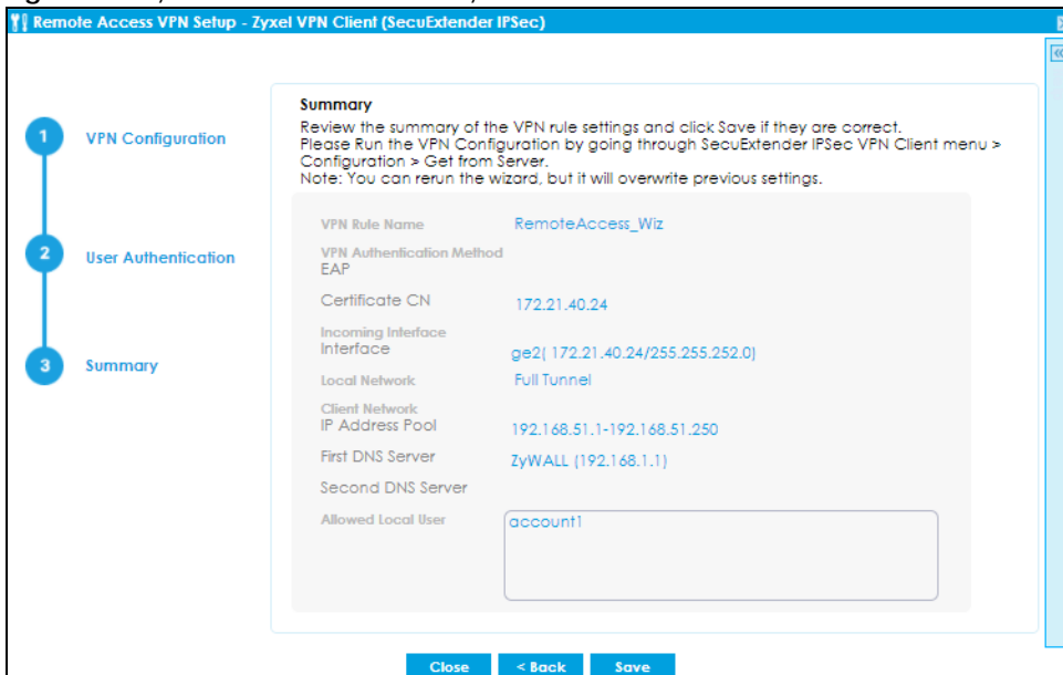
Figure 74 Zyxel VPN Client: Summary
