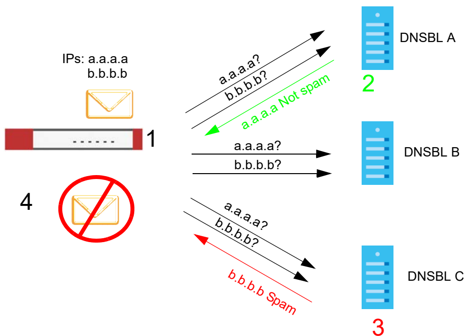
Figure 498 DNSBL Spam Detection Example
