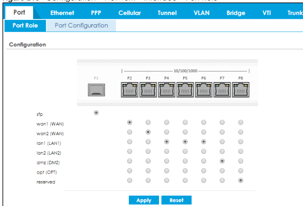
Figure 213 Configuration > Network > Interface > Port Role
