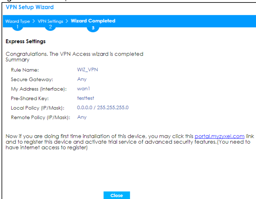
Figure 86 VPN Express Wizard: Finish
