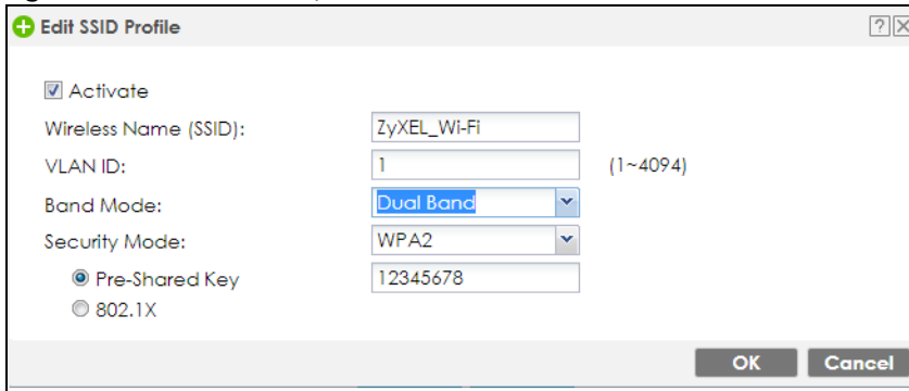
Figure 111 Wireless Setup Wizard &gt; SSID - Built-in AP &gt; Edit SSID - Pre-Shared Key
