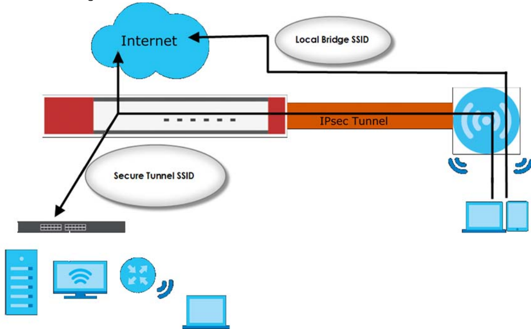
Figure 356 AP Using Secure Tunnel SSID Profile
