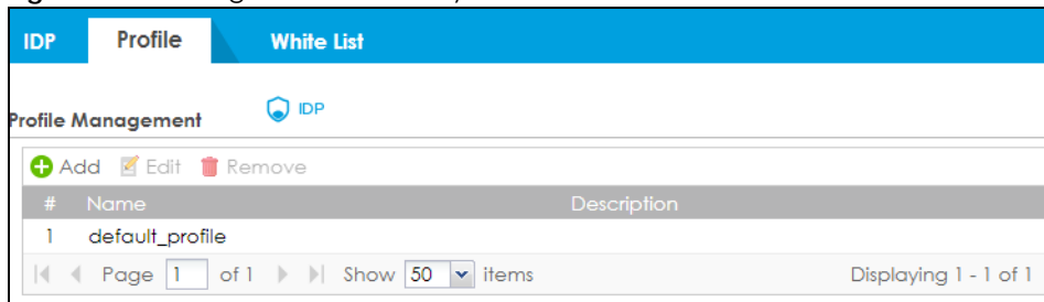
Figure 483 Configuration > Security Service > IDP> Profile
