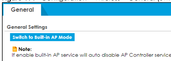
Figure 191 Configuration > Wireless > General (Switch to Built-in Mode)
