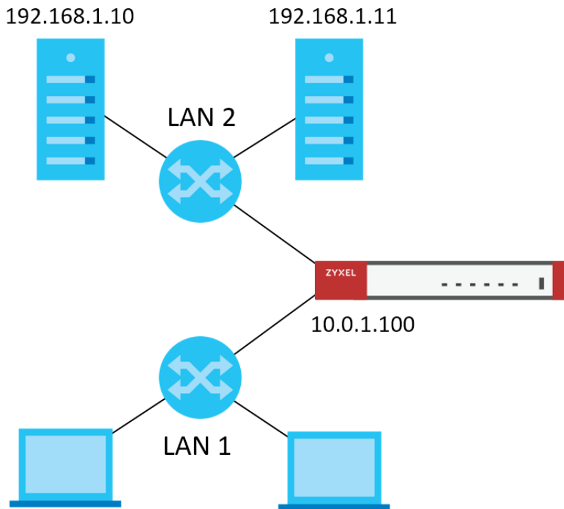
Figure 284 Virtual Server on the LAN - Example 2
