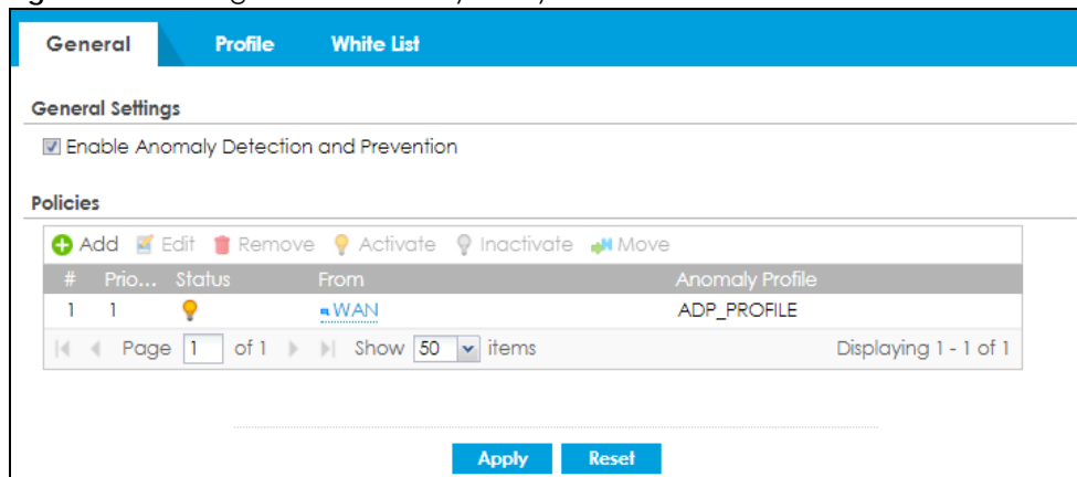
Figure 426 Configuration > Security Policy > ADP > General
