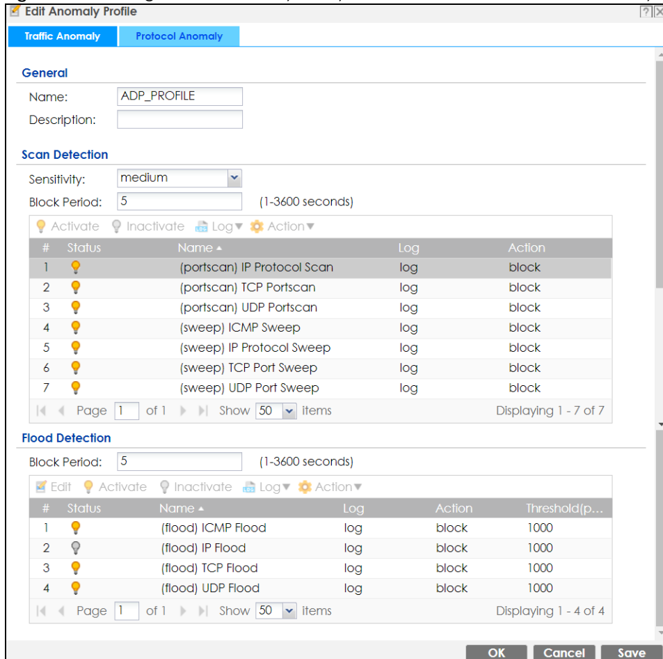
Figure 428 Configuration > Security Policy > ADP > Profile > Add-Traffic-Anomaly
