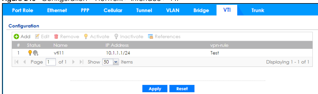
Figure 246 Configuration > Network > Interface > VTI
