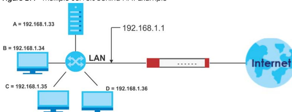
Figure 277 Multiple Servers Behind NAT Example
