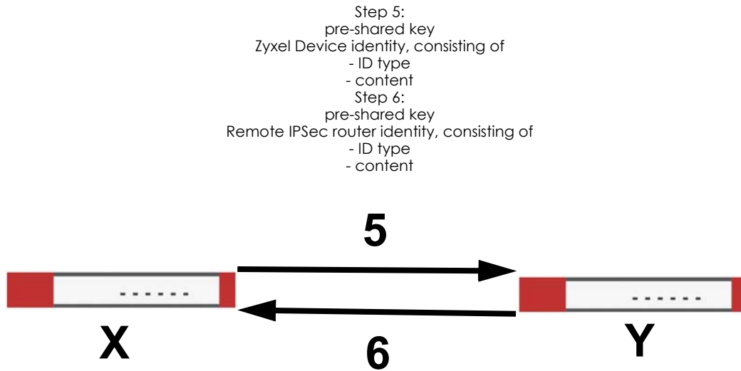
Figure 343 IKE SA: Main Negotiation Mode, Steps 5 - 6: Authentication (continued)
