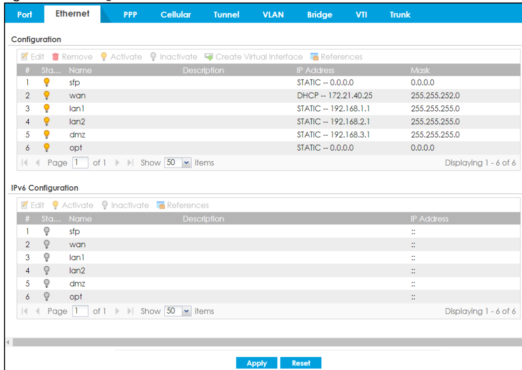
Figure 215 Configuration > Network > Interface > Ethernet
