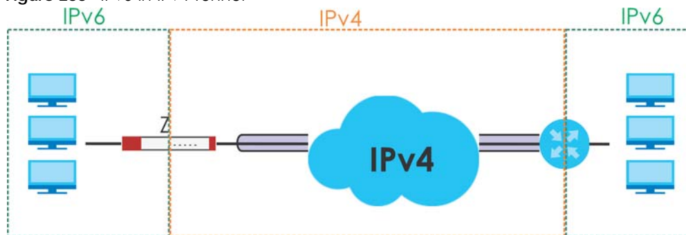
Figure 233 IPv6-in-IPv4 Tunnel
