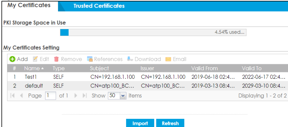
Figure 580 Configuration > Object > Certificate > My Certificates
