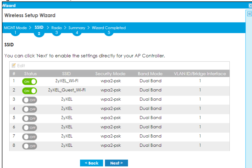
Figure 109 Wireless Setup Wizard > SSID - AP Controller
