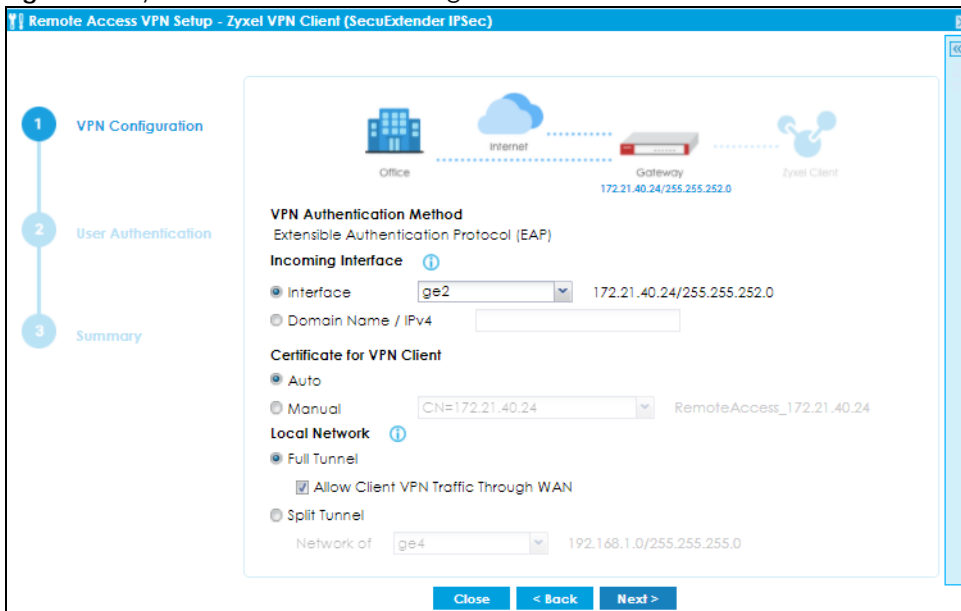
Figure 71 Zyxel VPN Client: VPN Configuration
