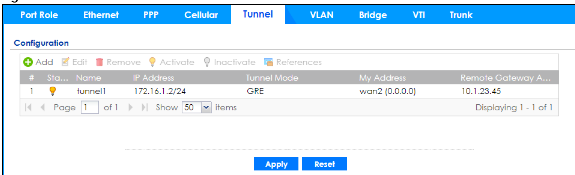
Figure 235 Network > Interface > Tunnel
