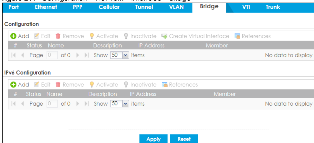
Figure 241 Configuration > Network > Interface > Bridge
