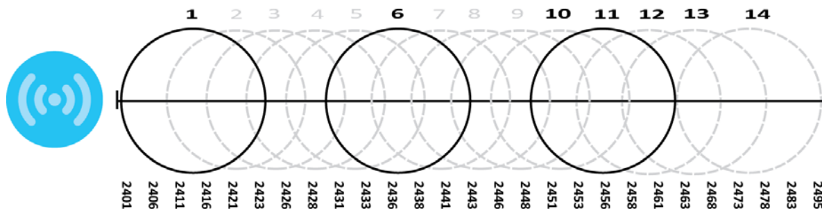
Figure 210 An Example Three-Channel Deployment
