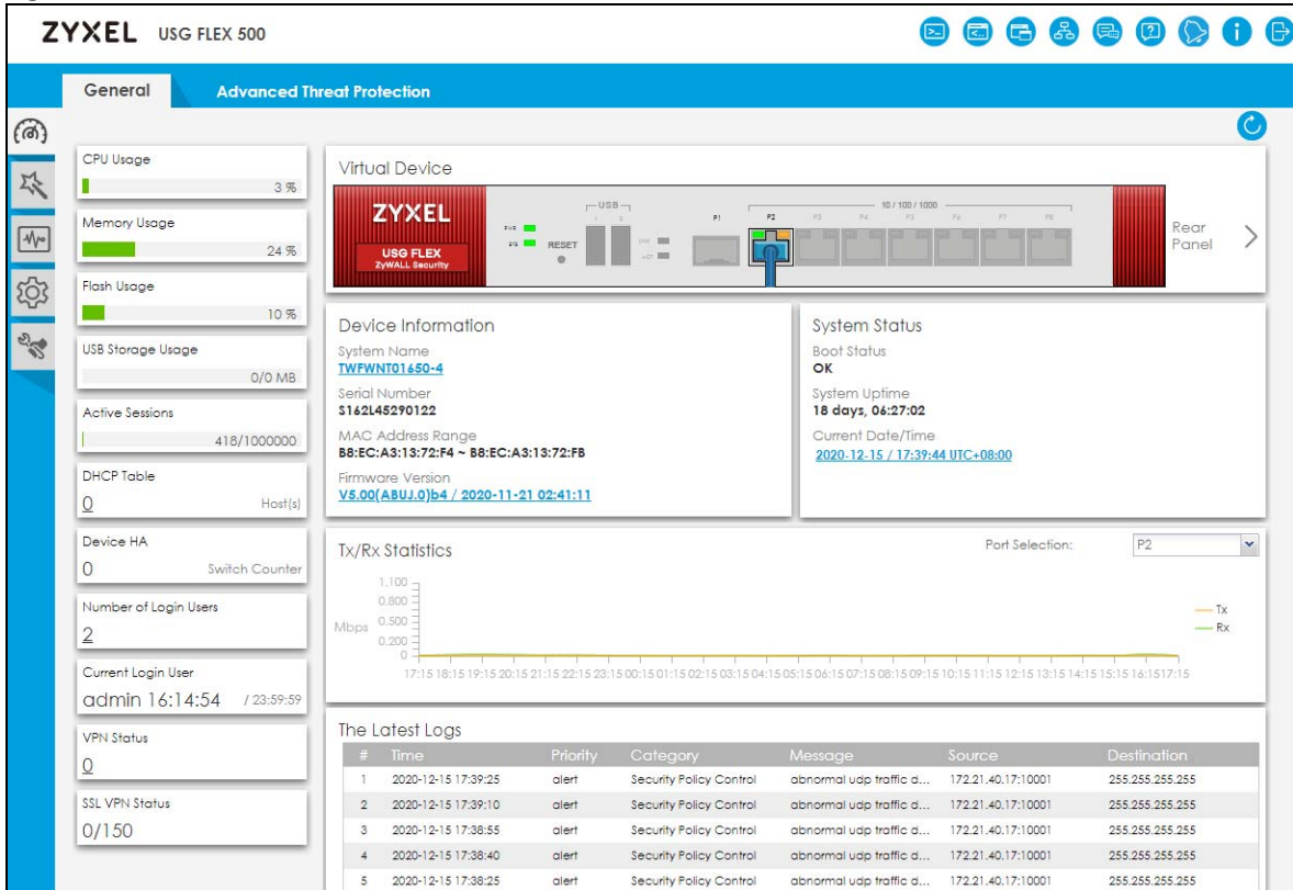
Figure 116 Dashboard USG FLEX
