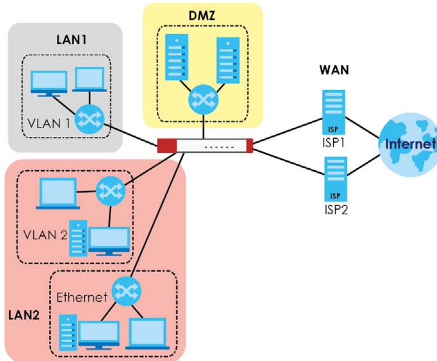
Figure 514 Example: Zones
