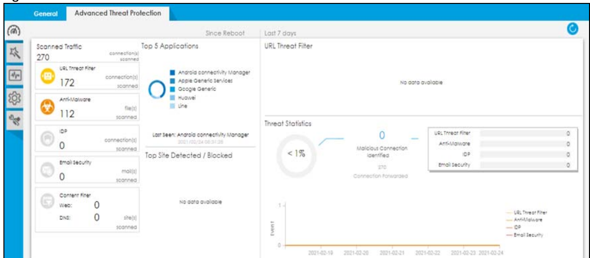
Figure 127 Dashboard > Advanced Threat Protection - USG FLEX Series
