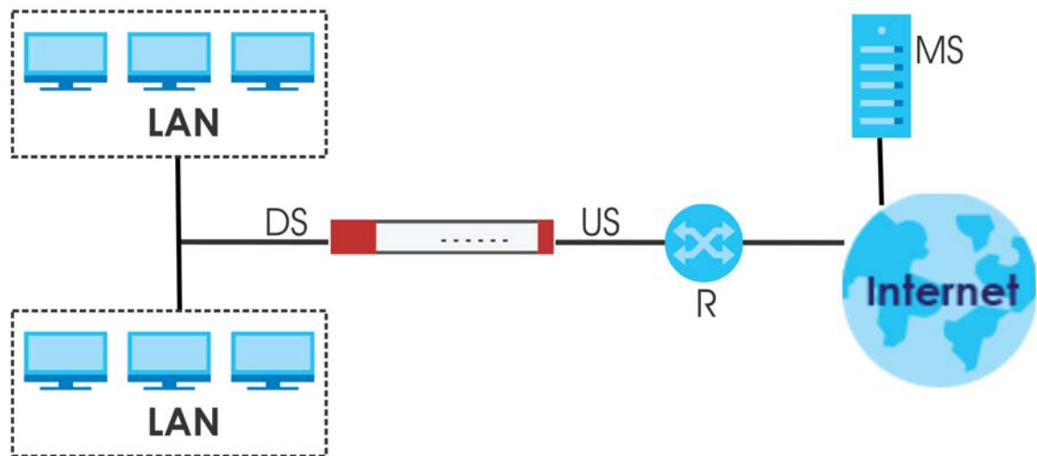
Figure 216 IGMP Proxy
