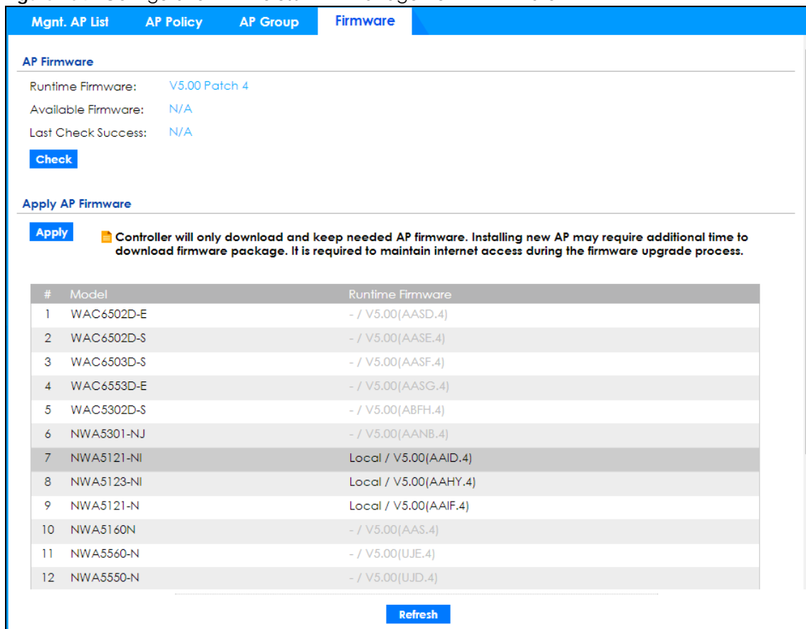
Figure 204 Configuration > Wireless > AP Management > Firmware
