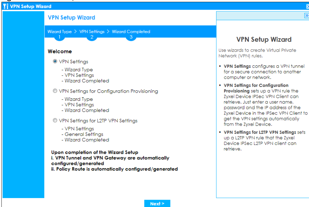
Figure 81 VPN Setup Wizard Welcome
