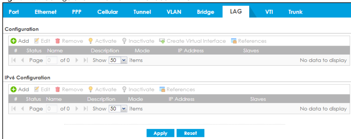
Figure 243 Configuration > Network > Interface > LAG
