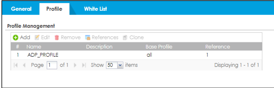
Figure 427 Configuration &gt; Security Policy &gt; ADP &gt; Profile
