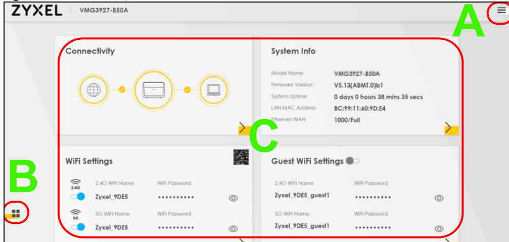
Figure 47 Screen Layout
