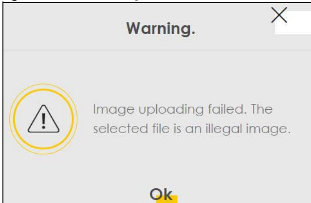
Figure 261 Error Message
