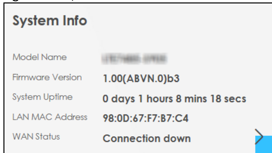
Figure 72 System Info
