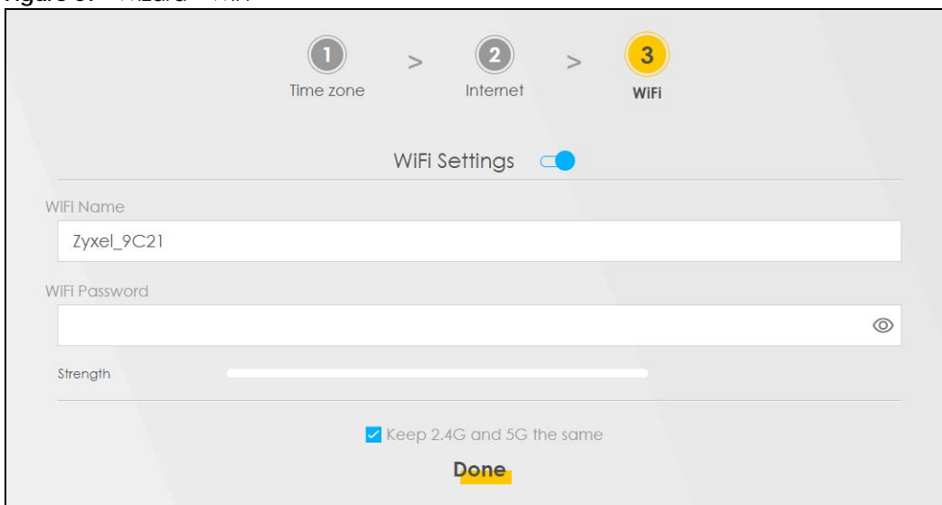
Figure 57 Wizard – WiFi
