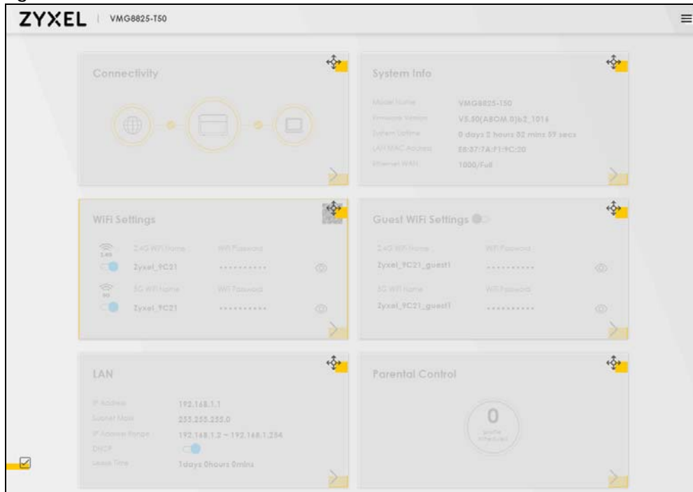
Figure 51 Screen Order
