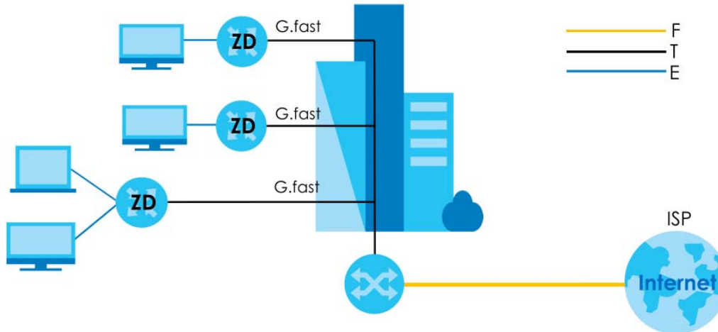
Figure 1 Fiber-To-The-Building (FTTB) with G.fast
