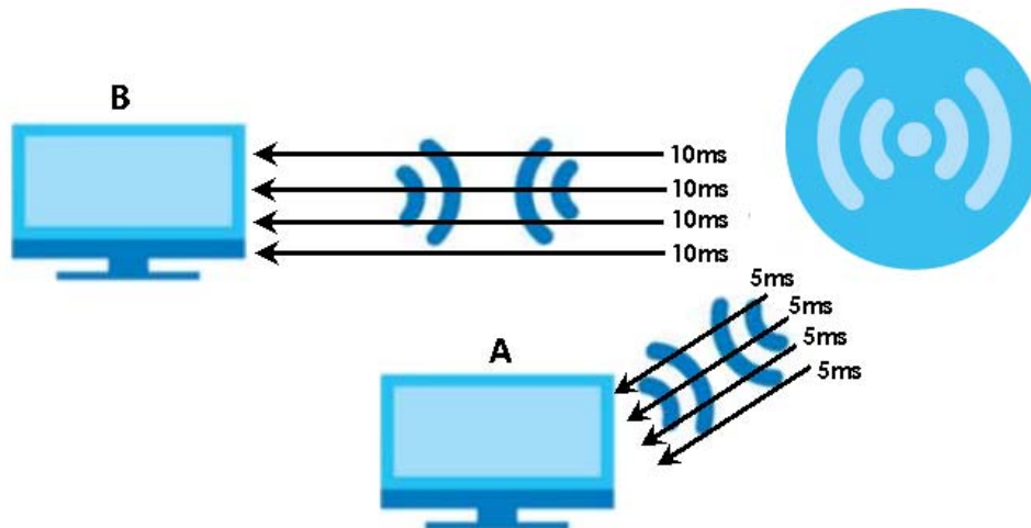
Figure 171 Airtime Fairness Example-Disabled
