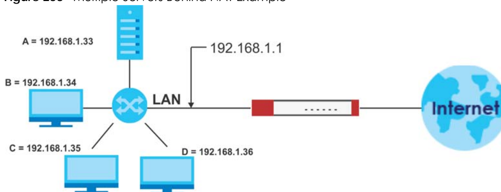
Figure 253 Multiple Servers Behind NAT Example
