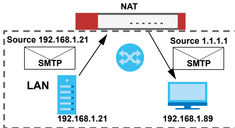
Figure 258 LAN to LAN Return Traffic
