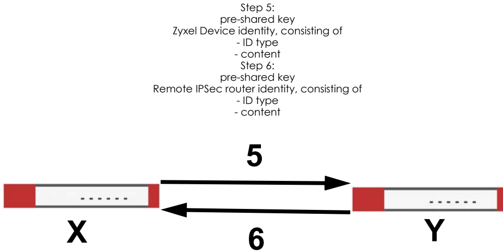
Figure 319 IKE SA: Main Negotiation Mode, Steps 5 - 6: Authentication (continued)
