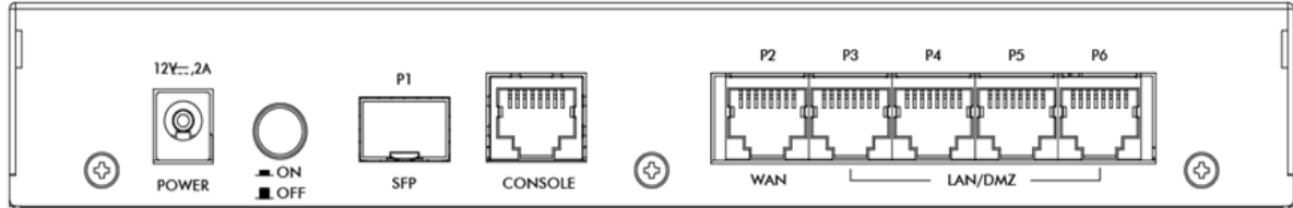
Figure 52 VPN100 Rear Panel
