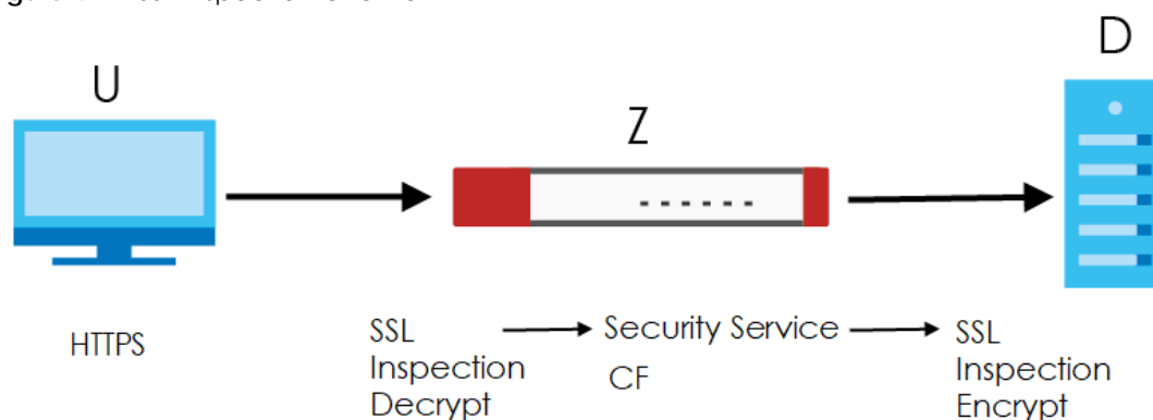
Figure 422 SSL Inspection Overview
