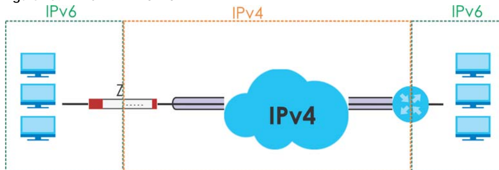
Figure 209 IPv6-in-IPv4 Tunnel
