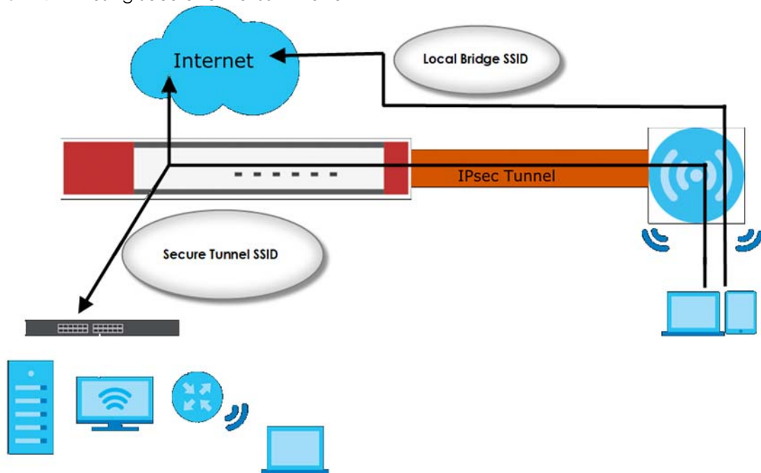
Figure 174 AP Using Secure Tunnel SSID Profile
