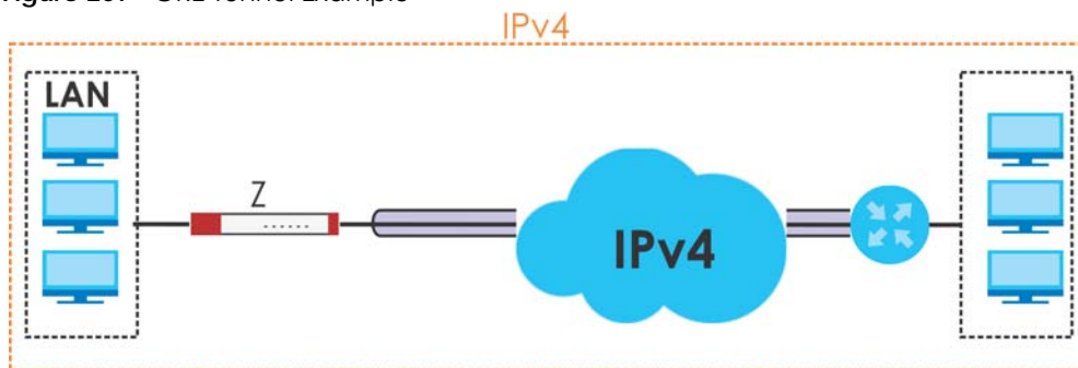
Figure 207 GRE Tunnel Example
