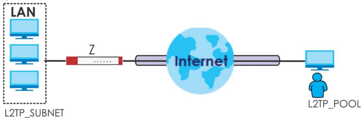
Figure 329 Policy Route for L2TP VPN
