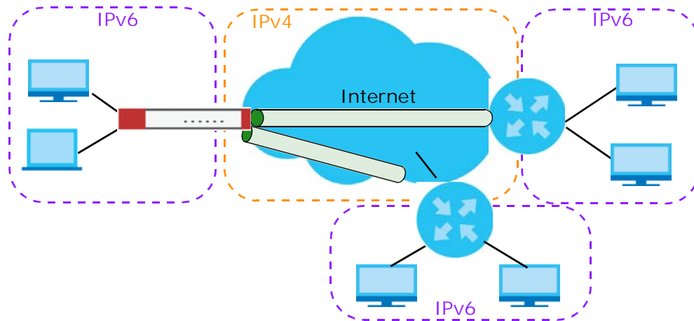
Figure 210 6to4 Tunnel
