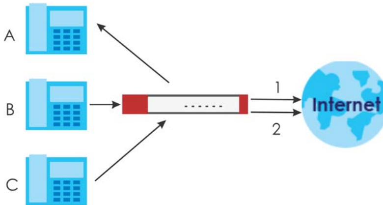
Figure 270 VoIP Calls from the WAN with Multiple Outgoing Calls
