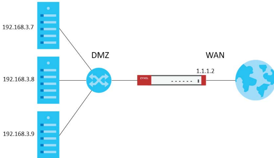
Figure 259 Virtual Server on the WAN- Example 1
