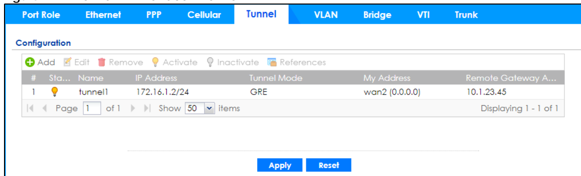
Figure 212 Network > Interface > Tunnel
