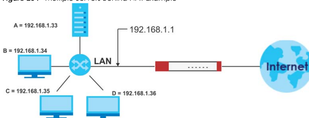
Figure 254 Multiple Servers Behind NAT Example
