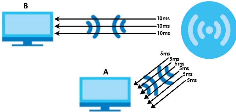
Figure 173 Airtime Fairness Example-Enabled
