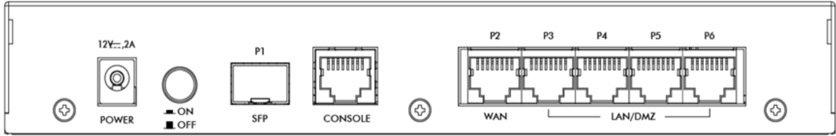
Figure 52 VPN100 Rear Panel
