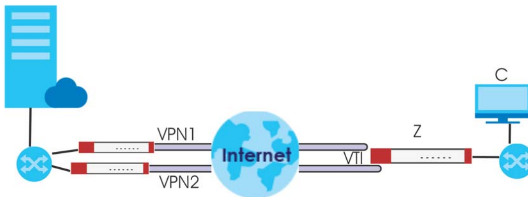
Figure 222 VTI and Trunk for VPN Load Balancing
