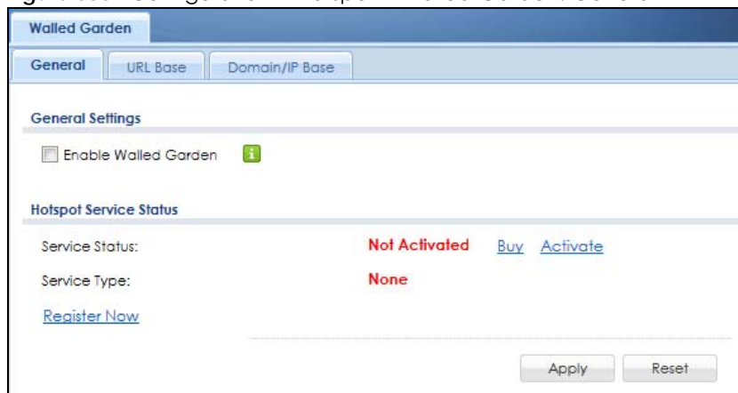
Figure 388 Configuration > Hotspot > Walled Garden: General
