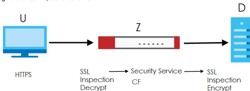
Figure 423 SSL Inspection Overview
