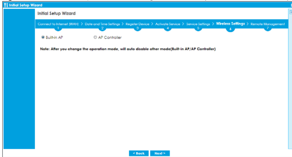
Figure 42 Wireless Setup Wizard > Management Mode (Models with Built-in AP)
