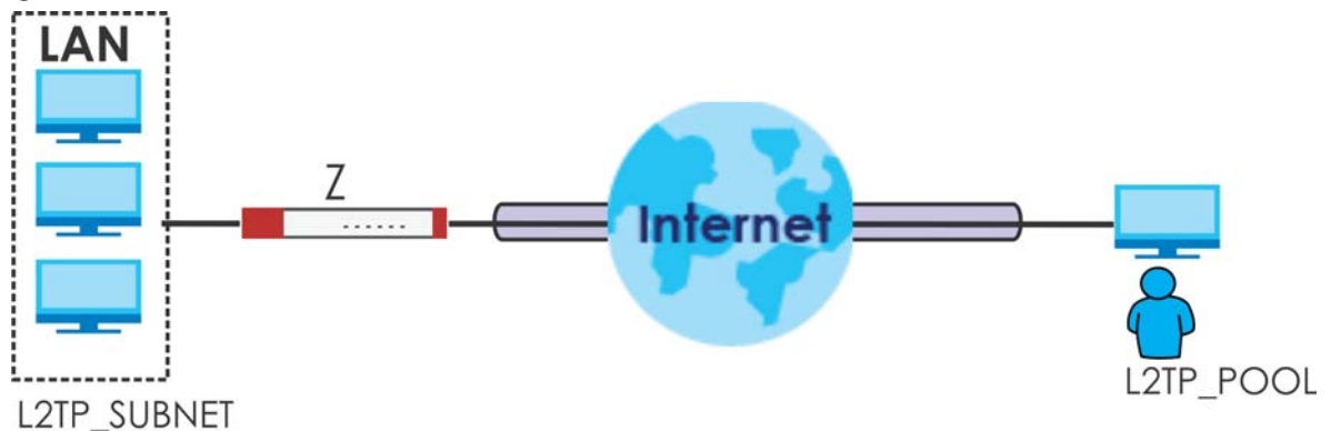
Figure 330 Policy Route for L2TP VPN
