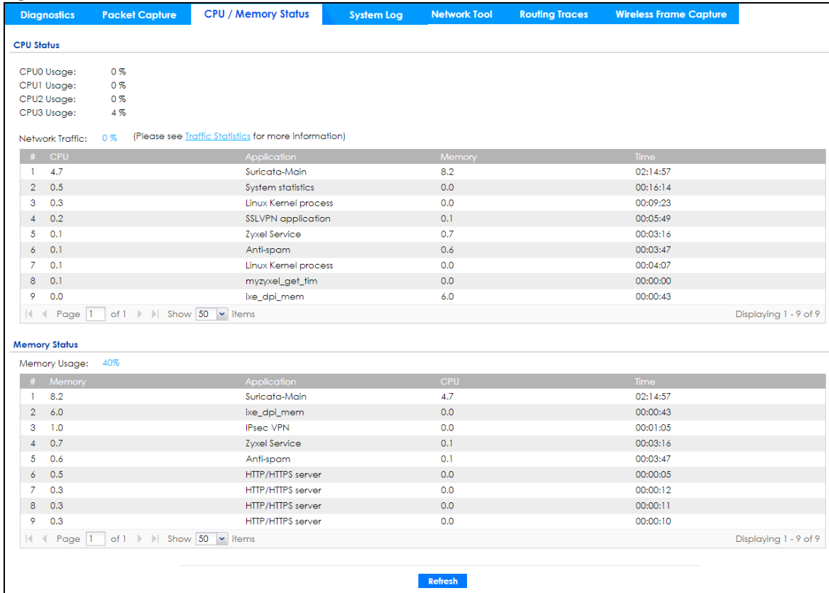
Figure 609 Maintenance > Diagnostics > CPU / Memory Status
