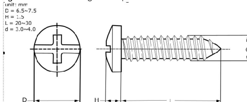
Figure 56 Wall Mounting Screw Specifications
