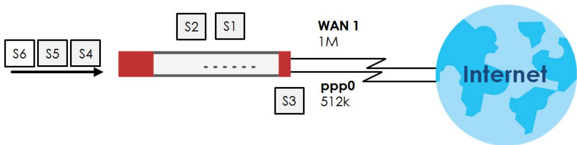
Figure 226 Weighted Round Robin Algorithm Example
