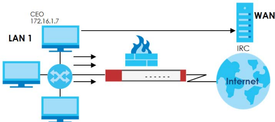
Figure 413 Limited LAN to WAN IRC Traffic Example
