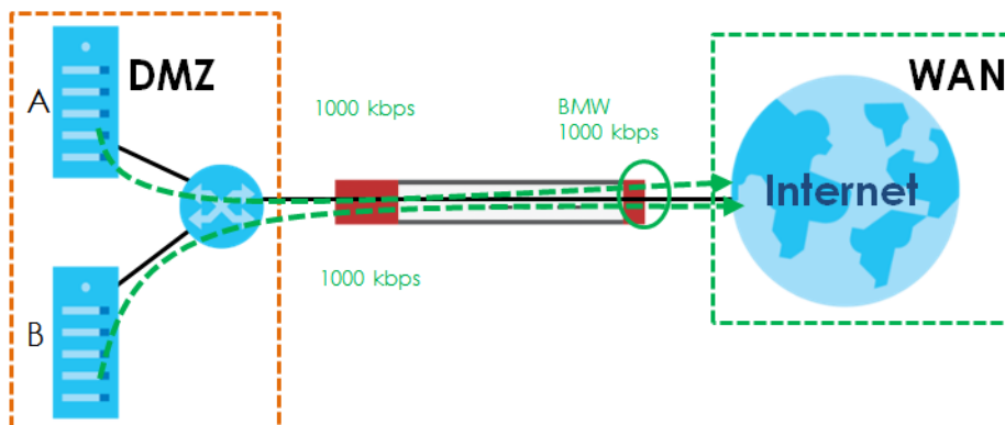
Figure 338 Bandwidth Management Behavior
