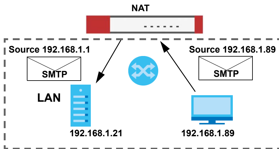
Figure 258 LAN to LAN Traffic
