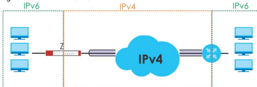
Figure 210 IPv6-in-IPv4 Tunnel
