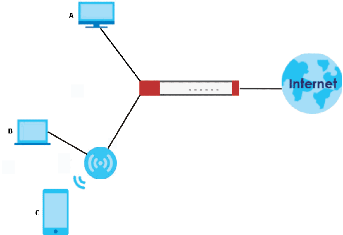
Figure 126 Clients' Device Insight Example
