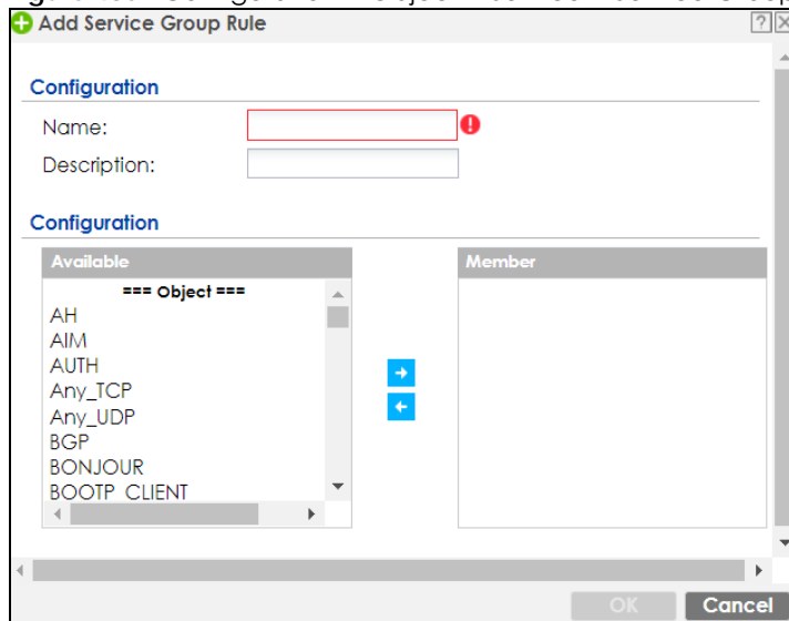
Figure 480 Configuration &gt; Object &gt; Service &gt; Service Group &gt; Edit
