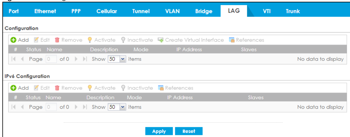
Figure 220 Configuration > Network > Interface > LAG
