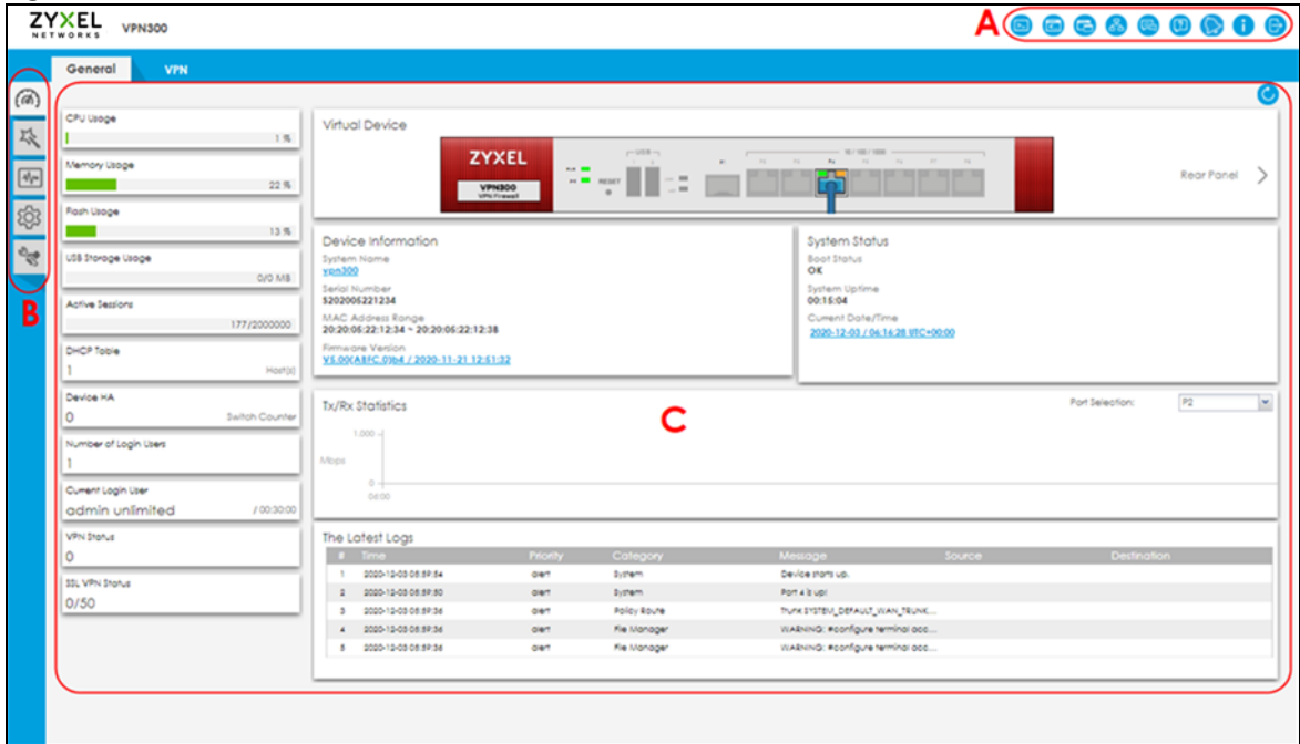
Figure 14 Web Configurator Screen Overview
