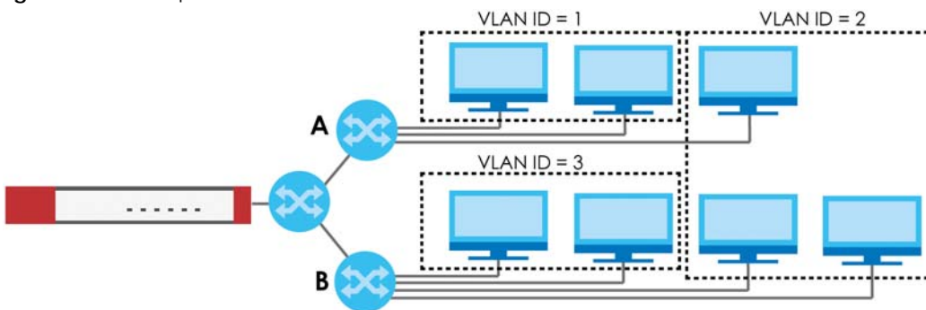
Figure 221 Example: After VLAN
