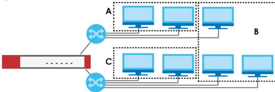
Figure 220 Example: Before VLAN
