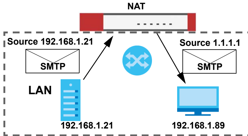
Figure 239 LAN to LAN Return Traffic
