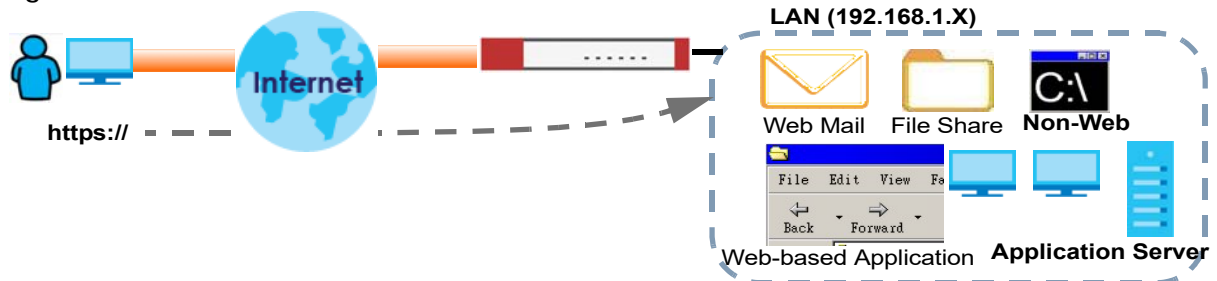
Figure 287 SSL VPN
