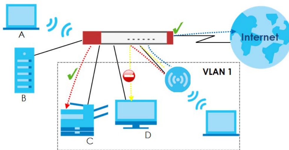
Figure 278 Layer-2 Isolation Application
