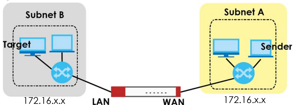
Figure 177 Proxy ARP
