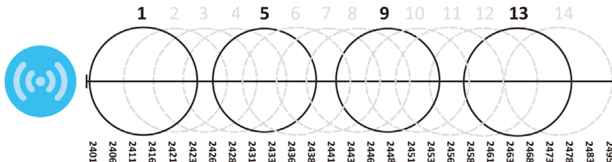
Figure 169 An Alternative Four-Channel Deployment
