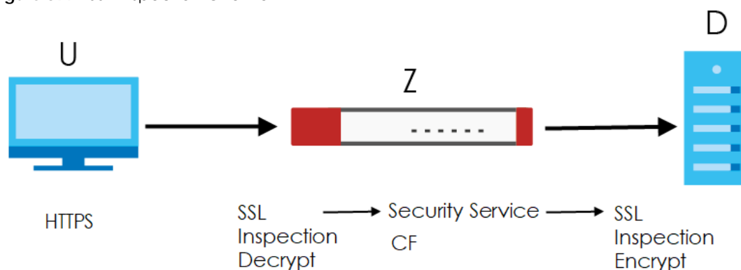
Figure 399 SSL Inspection Overview
