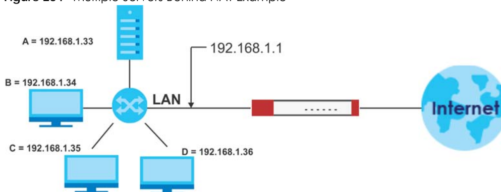
Figure 234 Multiple Servers Behind NAT Example
