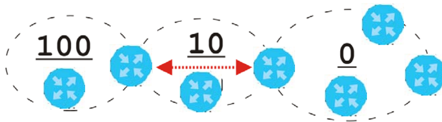
Figure 222 OSPF: Virtual Link
