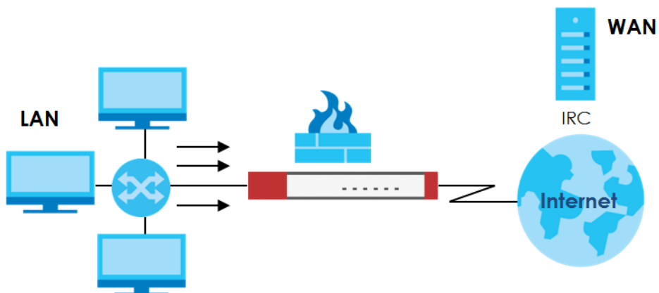
Figure 390 Blocking All LAN to WAN IRC Traffic Example
