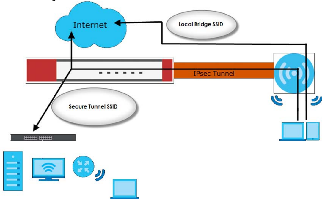
Figure 156 AP Using Secure Tunnel SSID Profile
