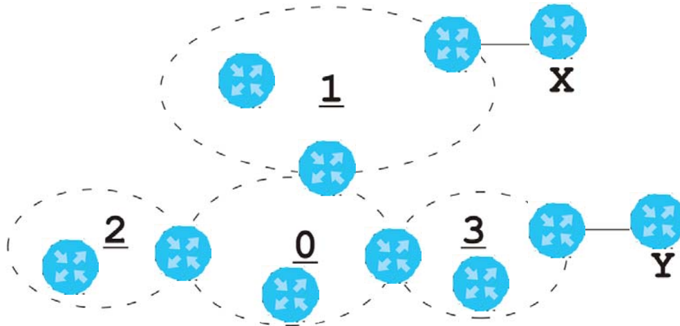
Figure 220 OSPF: Types of Areas
