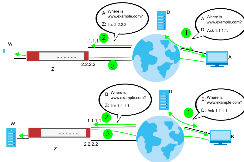
Figure 282 DNS Load Balancing Example
