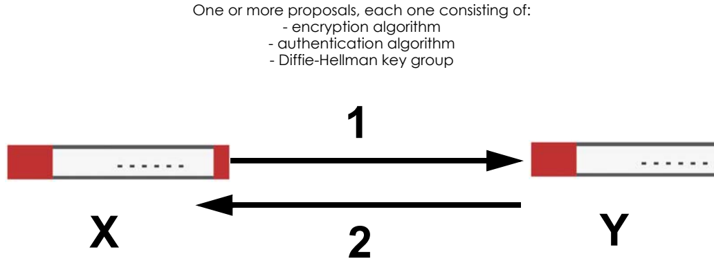
Figure 298 IKE SA: Main Negotiation Mode, Steps 1 - 2: IKE SA Proposal
