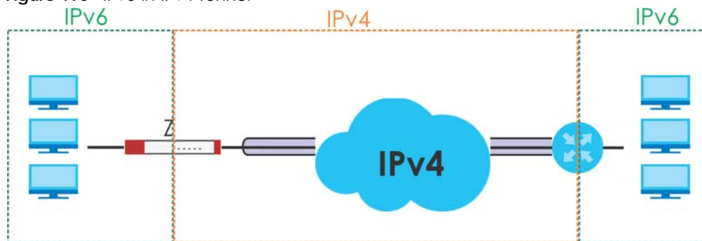
Figure 190 IPv6-in-IPv4 Tunnel
