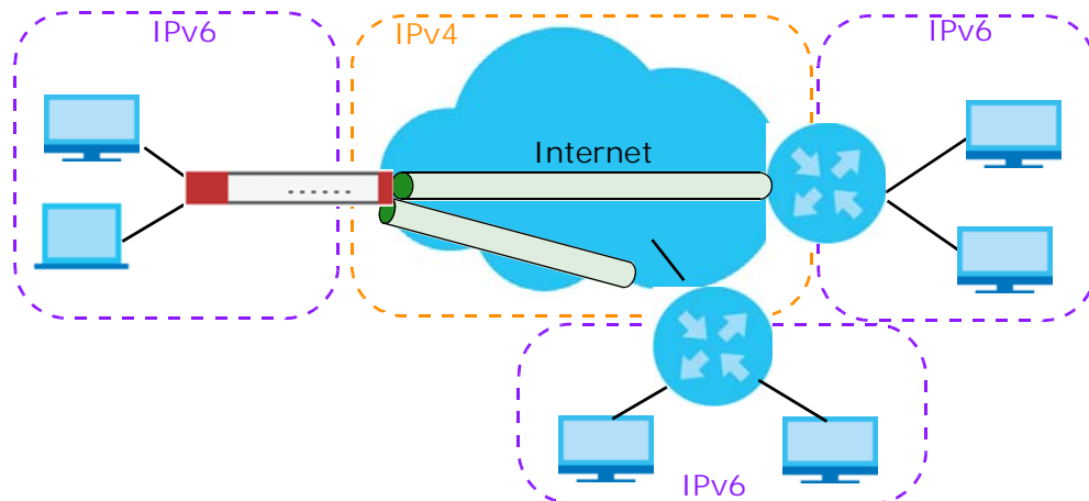
Figure 191 6to4 Tunnel
