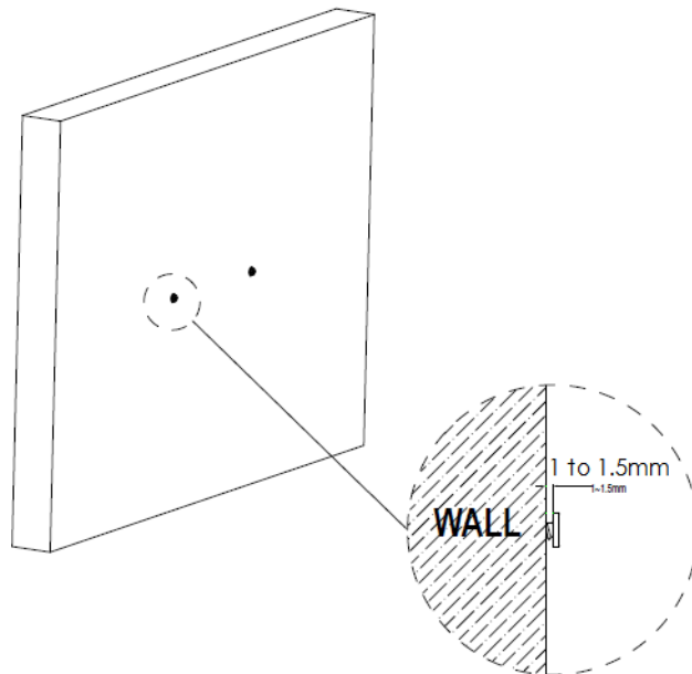
Figure 53 Gap for Cables
