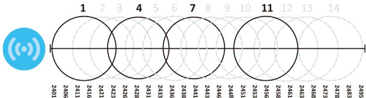
Figure 168 An Example Four-Channel Deployment
