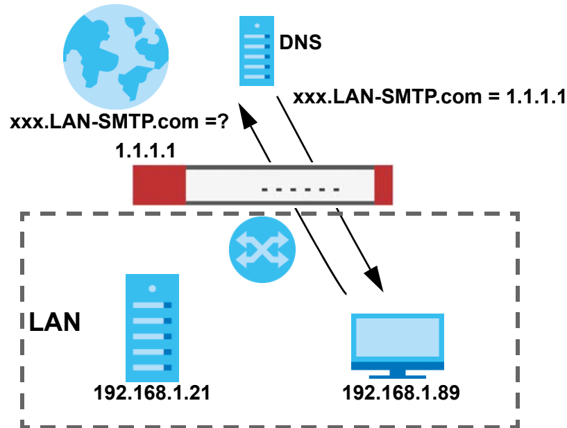
Figure 237 LAN Computer Queries a Public DNS Server
