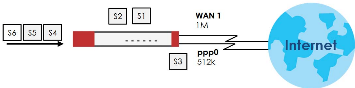
Figure 206 Weighted Round Robin Algorithm Example
