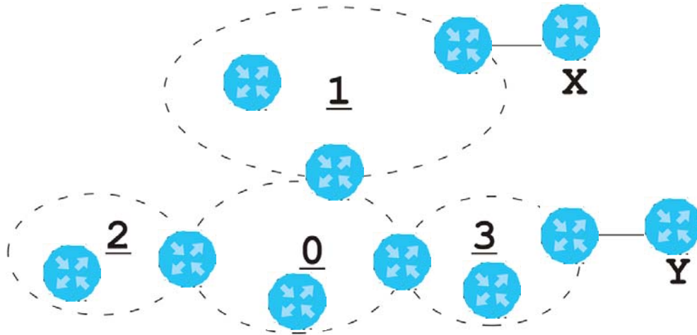
Figure 246 OSPF: Types of Areas
