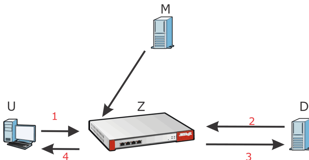
Figure 432 SSL Inspection Certificate Update Overview
