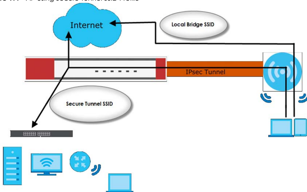
Figure 177 AP Using Secure Tunnel SSID Profile
