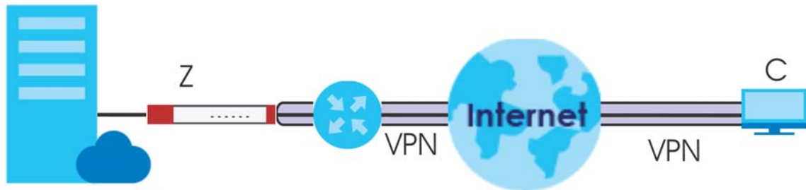
Figure 338 L2TP and Zyxel Device Behind a NAT Router
