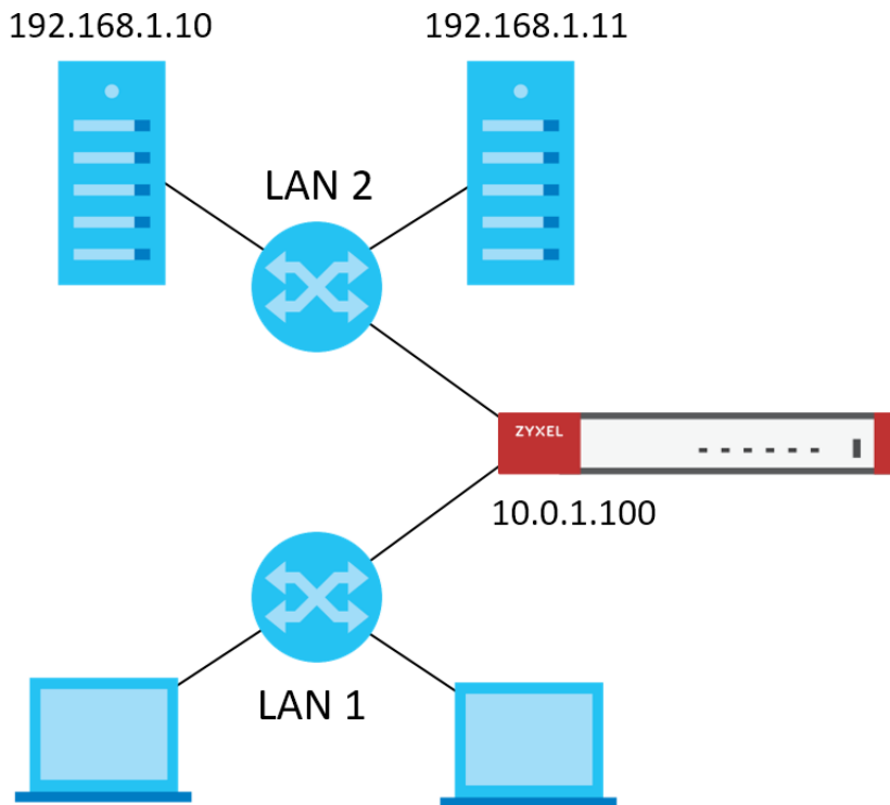
Figure 267 Virtual Server on the LAN - Example 2
