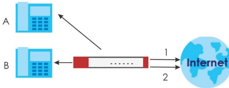
Figure 278 VoIP with Multiple WAN IP Addresses
