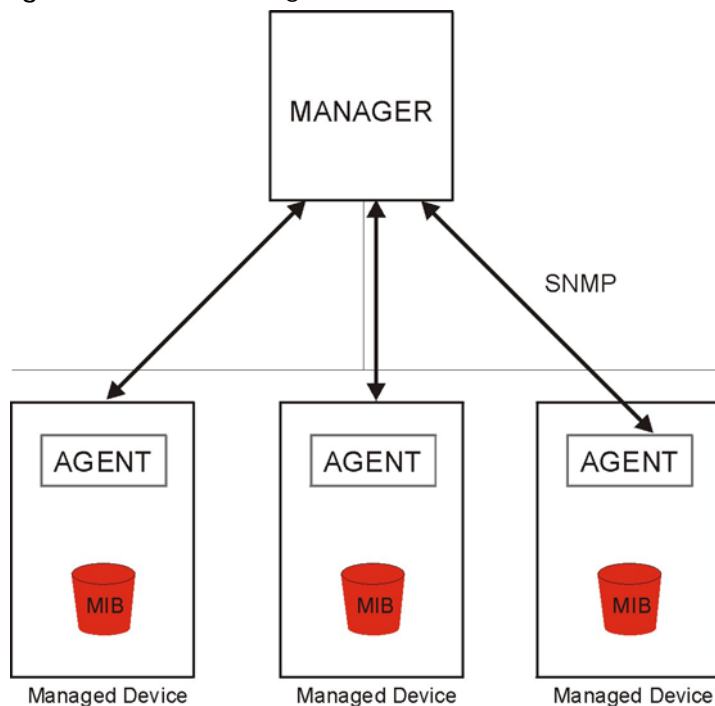
Figure 570 SNMP Management Model
