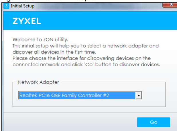
Figure 583 Network Adapter
