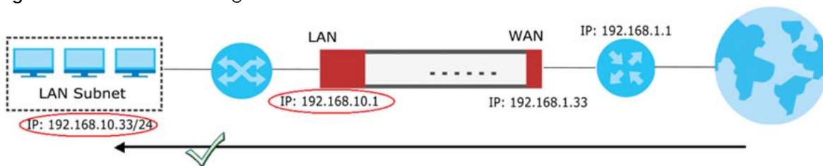
Figure 197 IP Address Change
