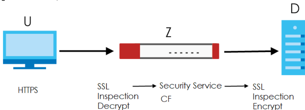
Figure 427 SSL Inspection Overview
