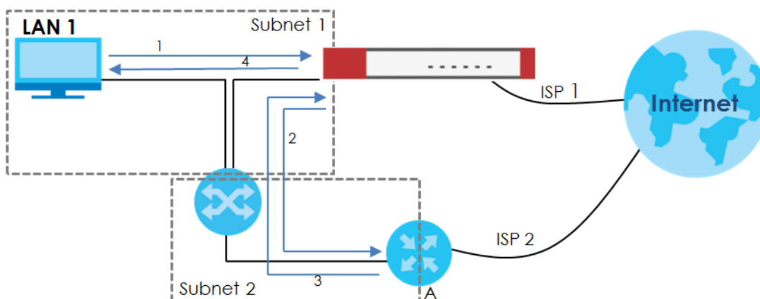
Figure 405 Using Virtual Interfaces to Avoid Asymmetrical Routes
