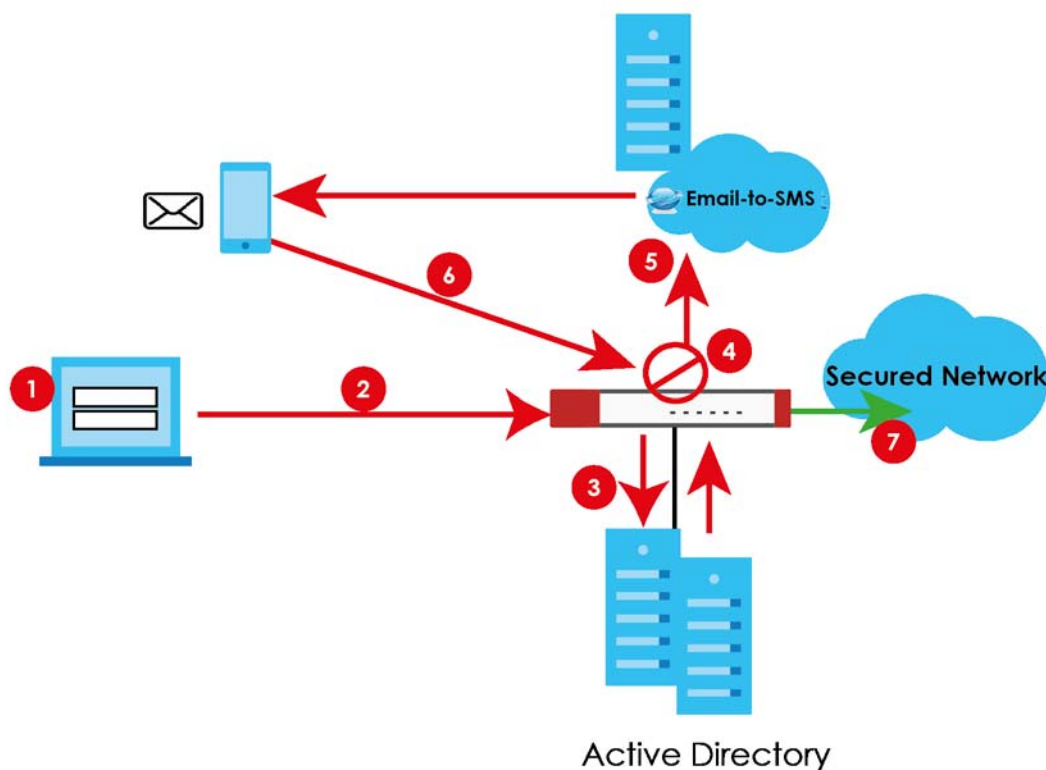
Figure 500 Two-Factor Authentication
