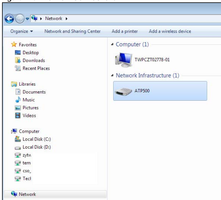
Figure 293 Network Connections
