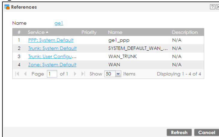
Figure 206 References
