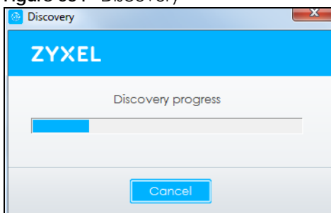
Figure 584 Discovery
