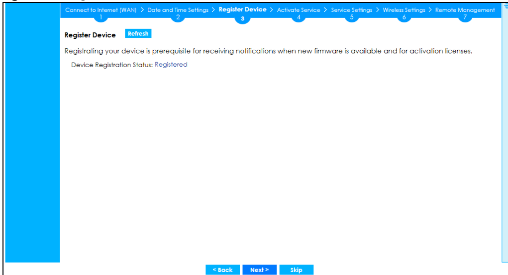
Figure 40 Registered Device
