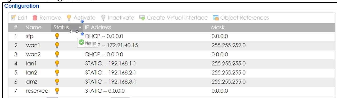
Figure 25 Moving Columns
