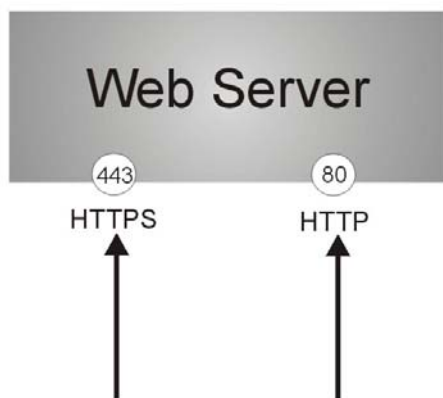
Figure 541 HTTP/HTTPS Implementation
