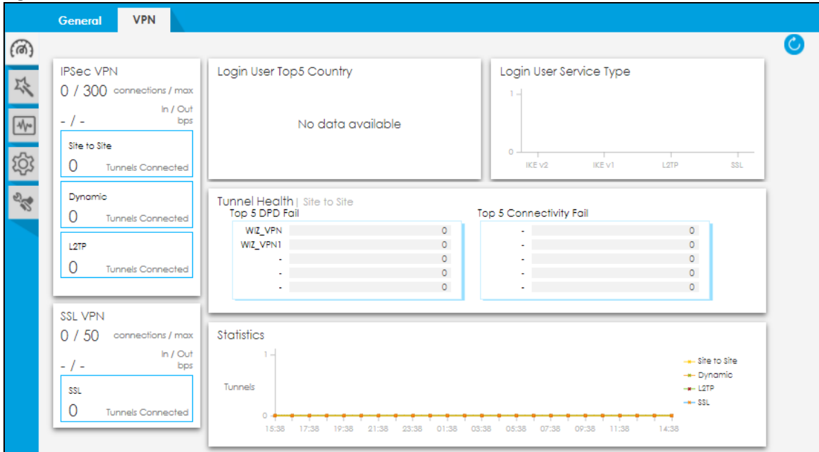
Figure 119 Dashboard > VPN-VPN
