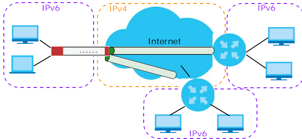
Figure 217 6to4 Tunnel
