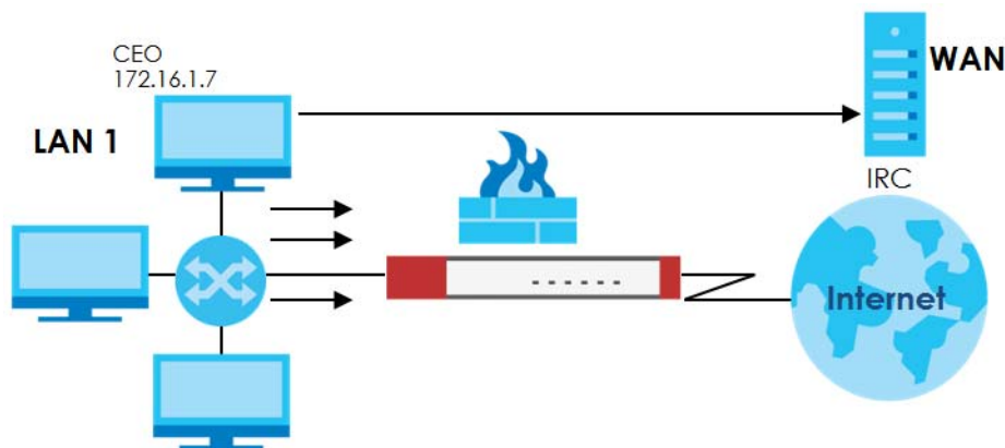
Figure 418 Limited LAN to WAN IRC Traffic Example
