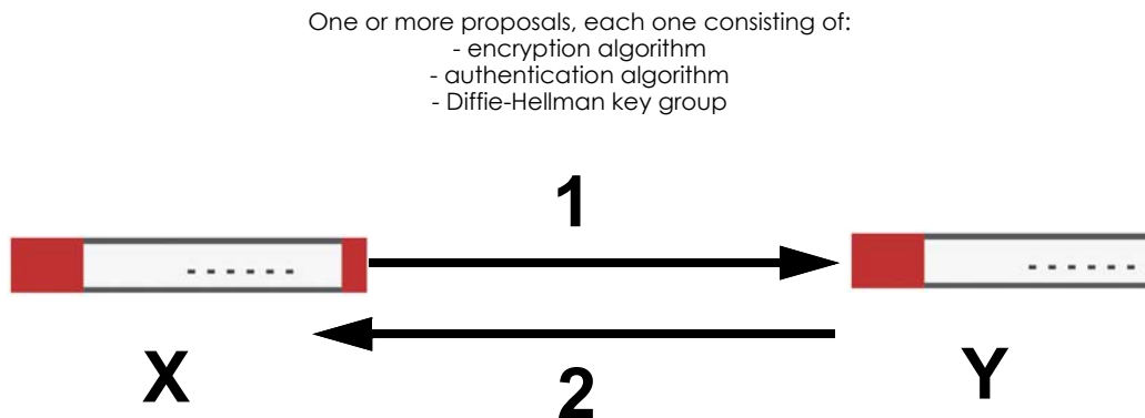
Figure 324 IKE SA: Main Negotiation Mode, Steps 1 - 2: IKE SA Proposal
