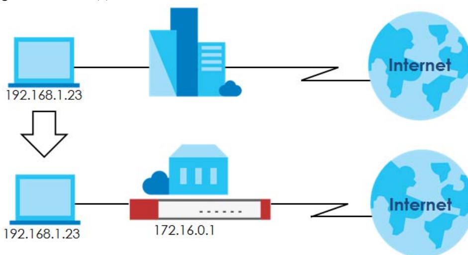
Figure 391 IPnP Application
