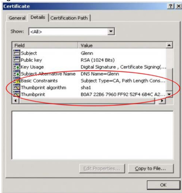
Figure 504 Certificate Details
