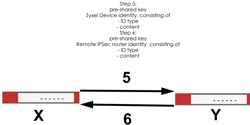
Figure 326 IKE SA: Main Negotiation Mode, Steps 5 - 6: Authentication (continued)
