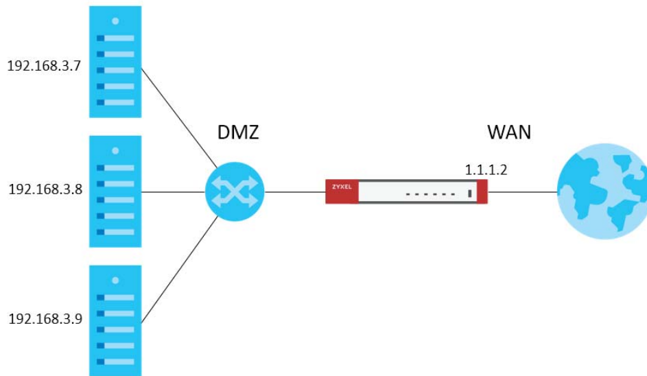
Figure 266 Virtual Server on the WAN- Example 1
