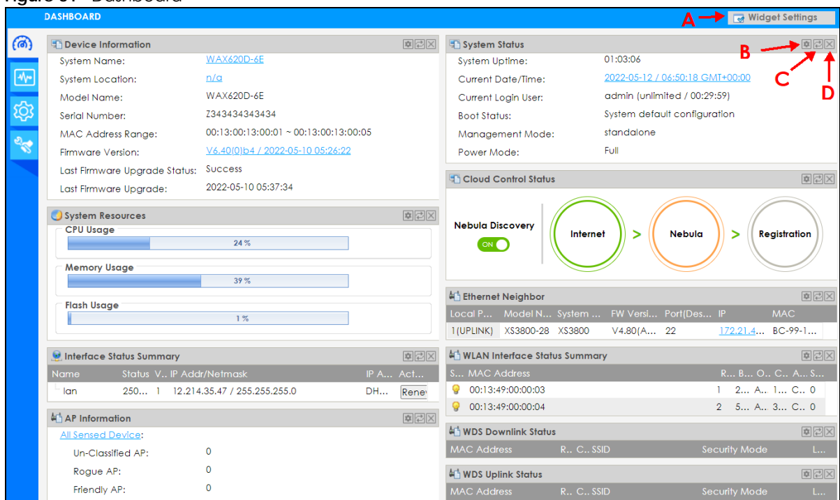
Figure 31 Dashboard
