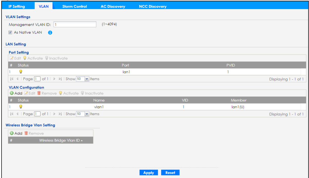
Figure 58 Configuration > Network > VLAN (for Zyxel Device with one Ethernet port)
