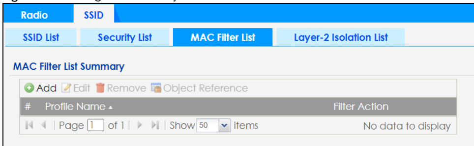
Figure 95 Configuration > Object > AP Profile > SSID > MAC Filter List
