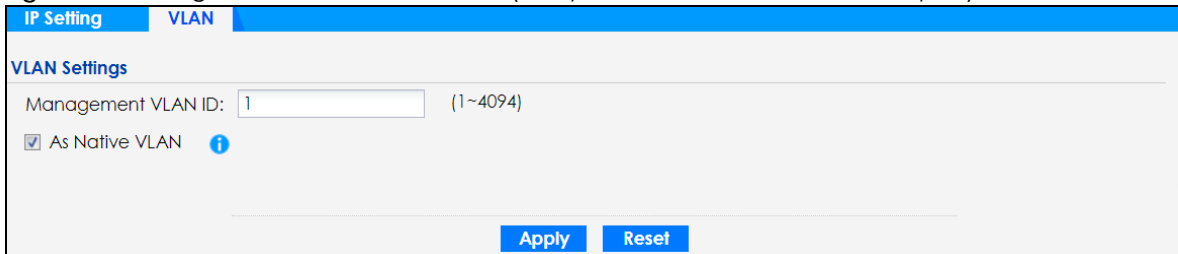
Figure 58 Configuration > Network > VLAN (for Zyxel Device with one Ethernet port)
