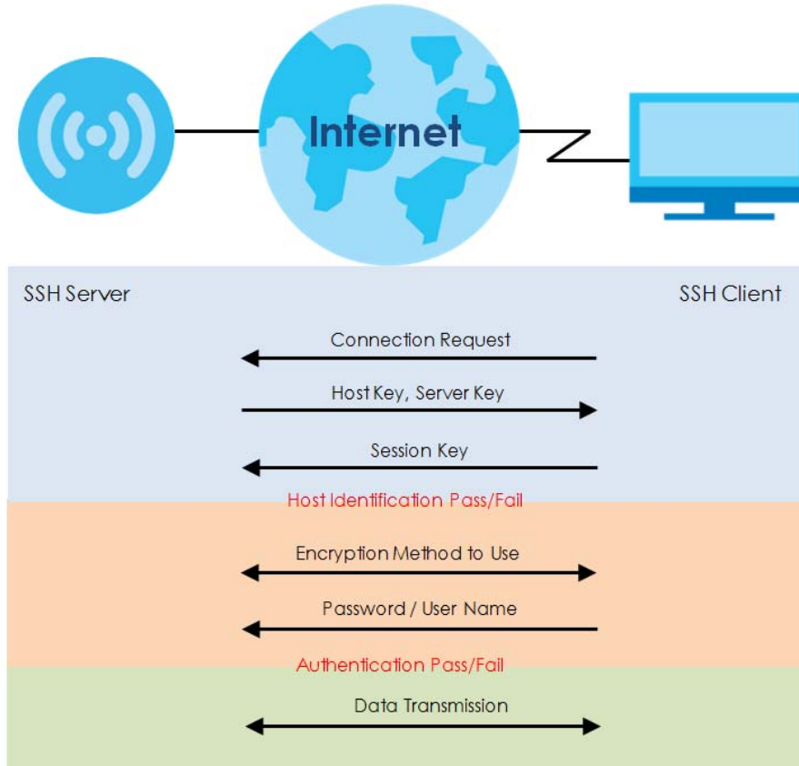
Figure 141 How SSH v1 Works Example
