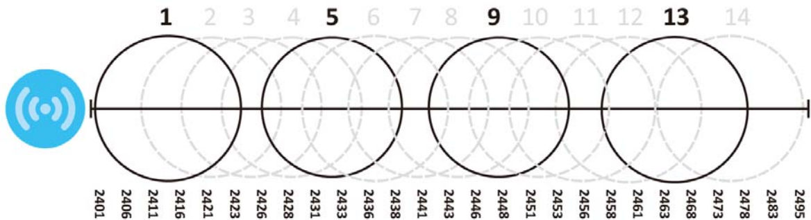
Figure 93 An Alternative Four-Channel Deployment
