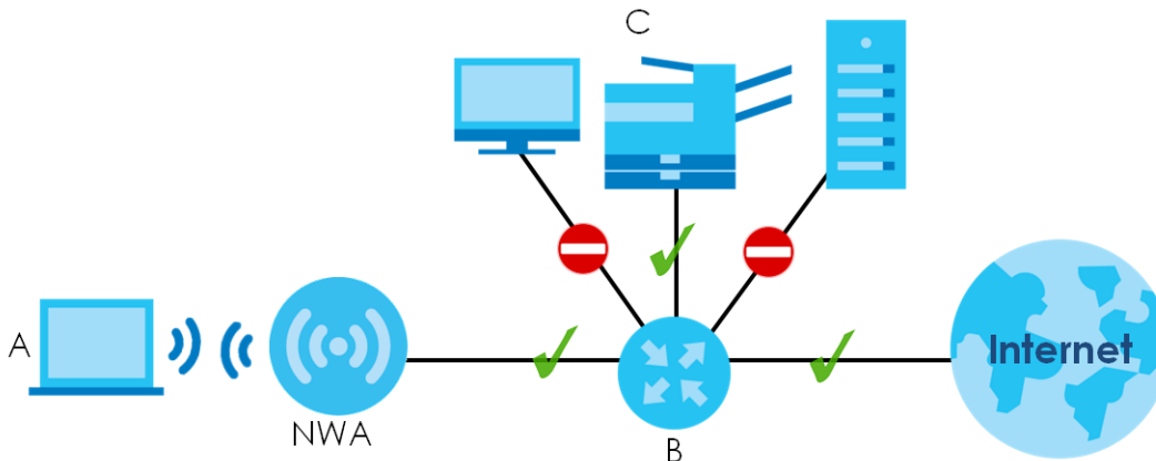
Figure 118 Layer-2 Isolation Application
