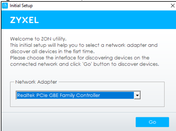
Figure 12 Network Adapter
