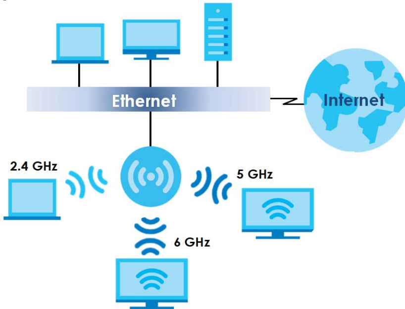
Figure 8 Triple-Radio Application
