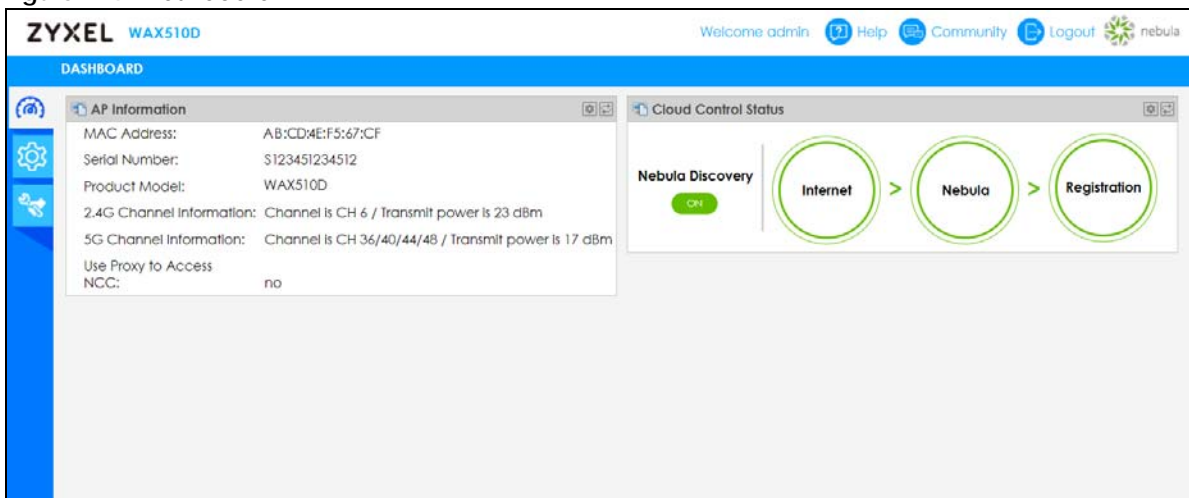
Figure 174 Dashboard
