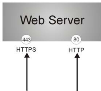
Figure 135 HTTP/HTTPS Implementation
