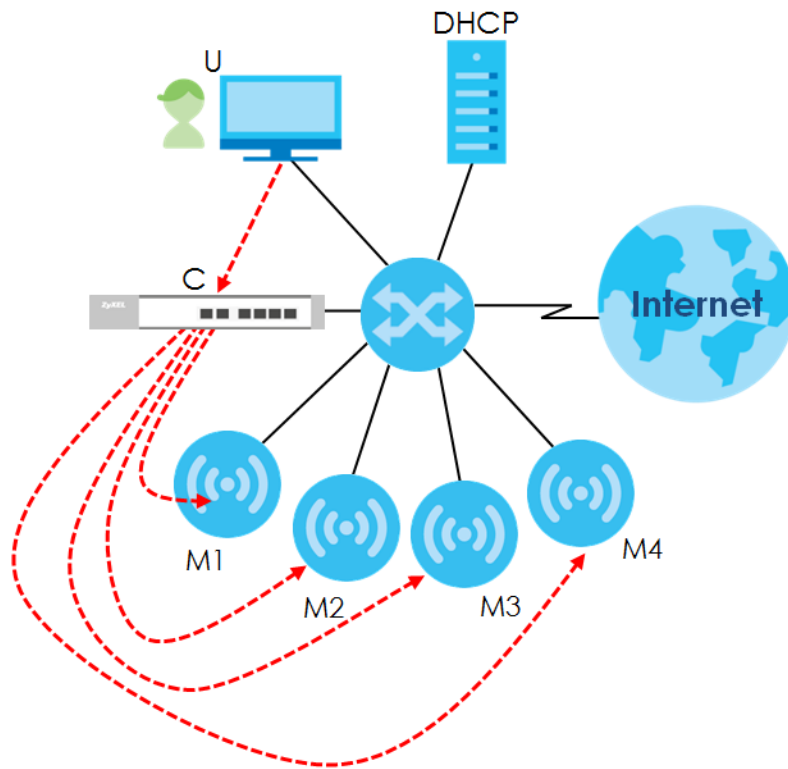
Figure 70 AC managed Network Example
