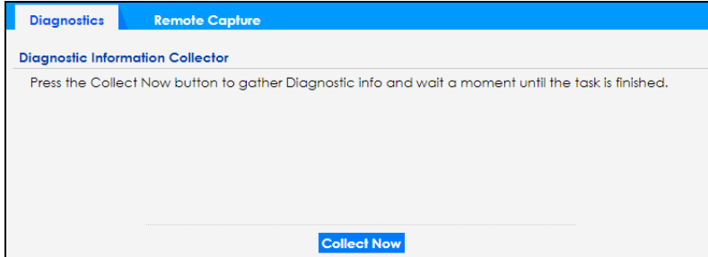
Figure 178 Maintenance > Diagnostics
