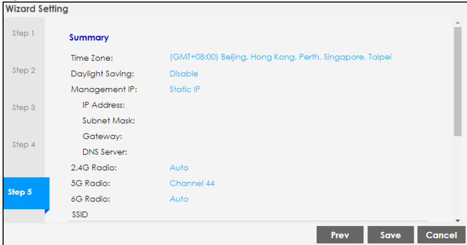
Figure 51 Wizard: Summary
