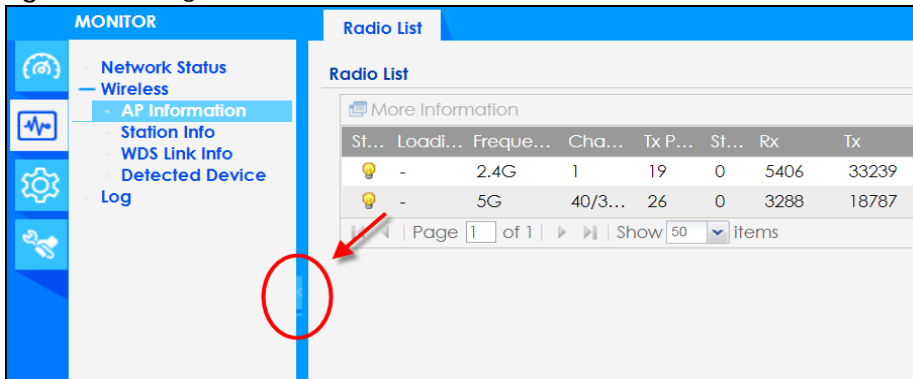
Figure 38 Navigation Panel
