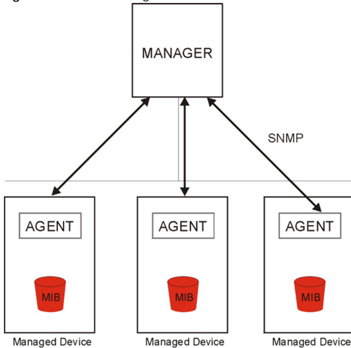
Figure 146 SNMP Management Model
