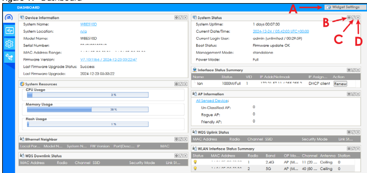
Figure 41 Dashboard
