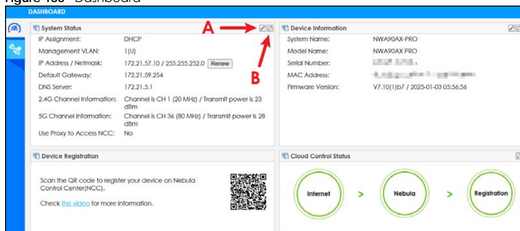
Figure 188 Dashboard
