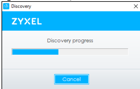
Figure 17 Discovery
