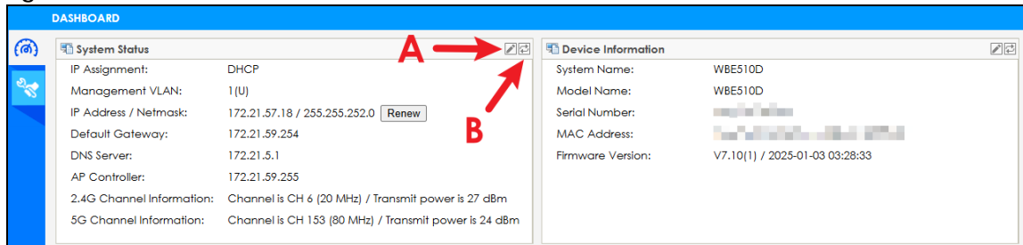
Figure 171 Dashboard
