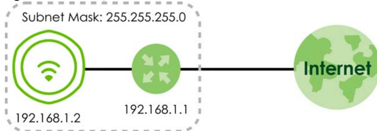
Figure 70 IP Setup
