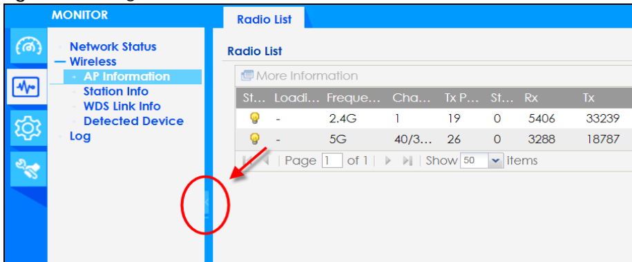
Figure 39 Navigation Panel
