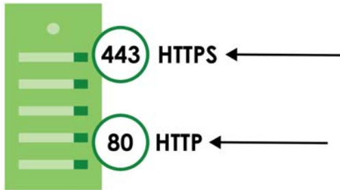
Figure 132 HTTP/HTTPS Implementation
