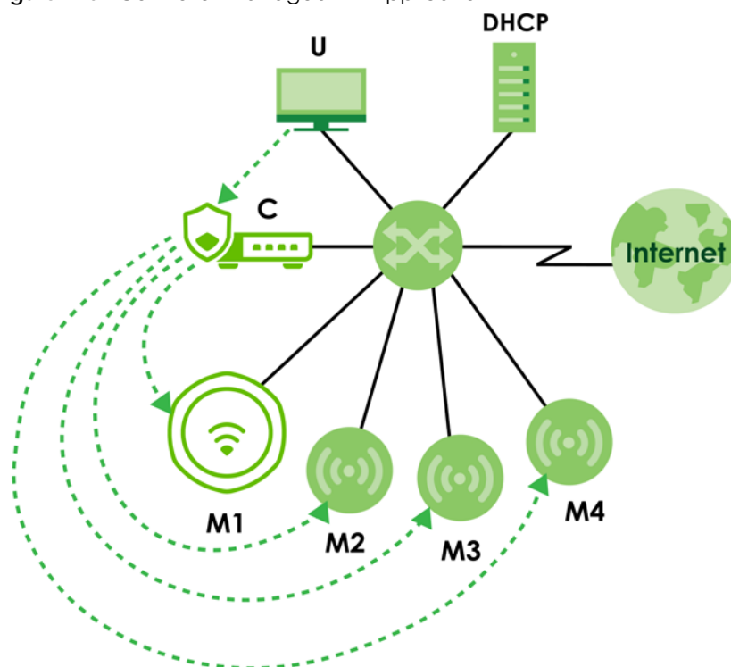
Figure 170 Controller Managed AP Application
