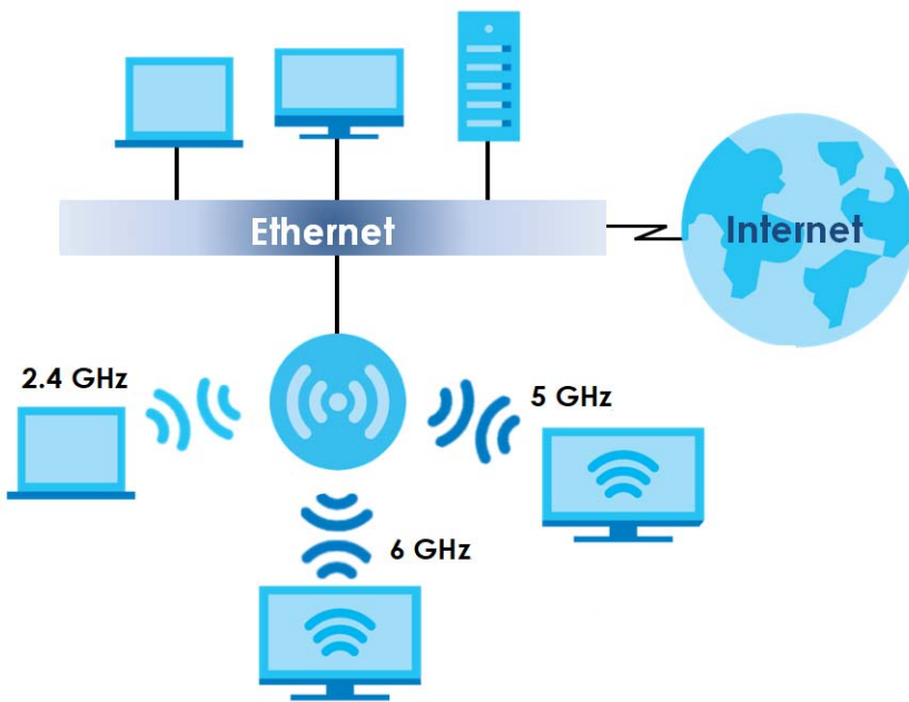
Figure 7 Triple-Radio Application
