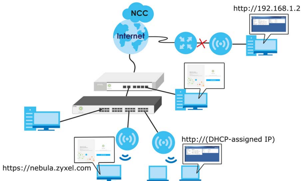
Figure 162 Cloud Mode Application
