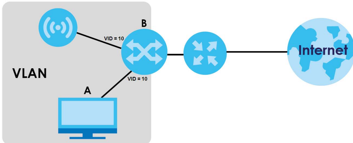
Figure 60 Management VLAN Setup
