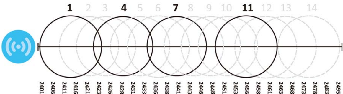
Figure 79 An Example Four-Channel Deployment
