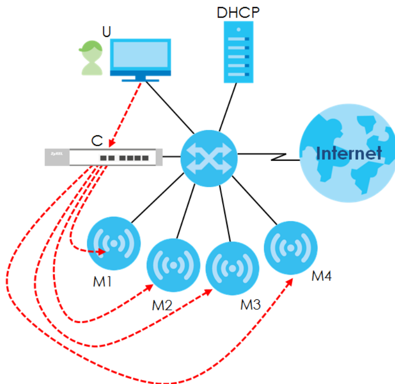
Figure 57 AC managed Network Example
