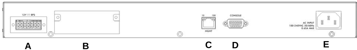
Figure 15 Rear Panel
