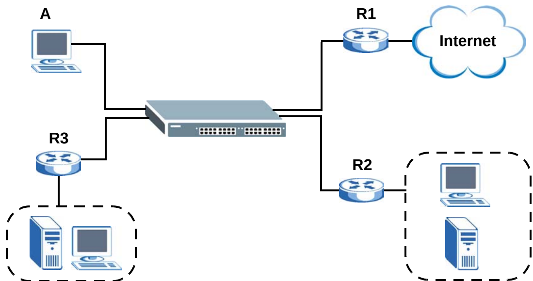
Figure 154 Example of Static Routing Topology
