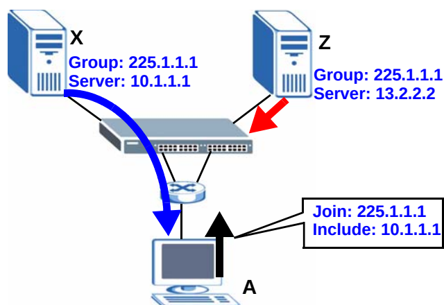
Figure 171 IGMP Version 3 Example
