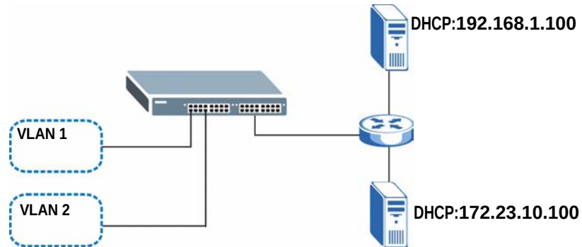
Figure 191 DHCP Relay for Two VLANs
