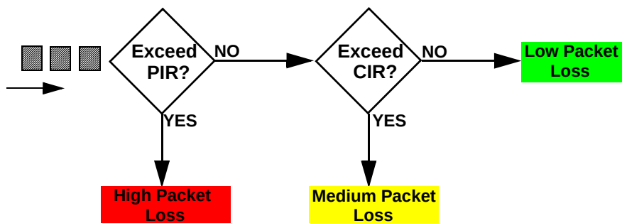
Figure 180 TRTCM - Color-blind Mode
