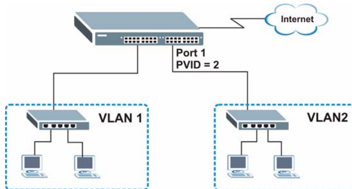
Figure 26 Initial Setup Network Example: Port VID
