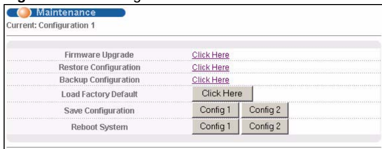
Figure 210 Management > Maintenance
