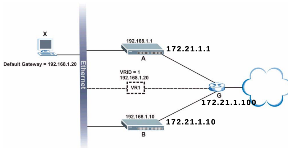
Figure 193 VRRP: Example 1
