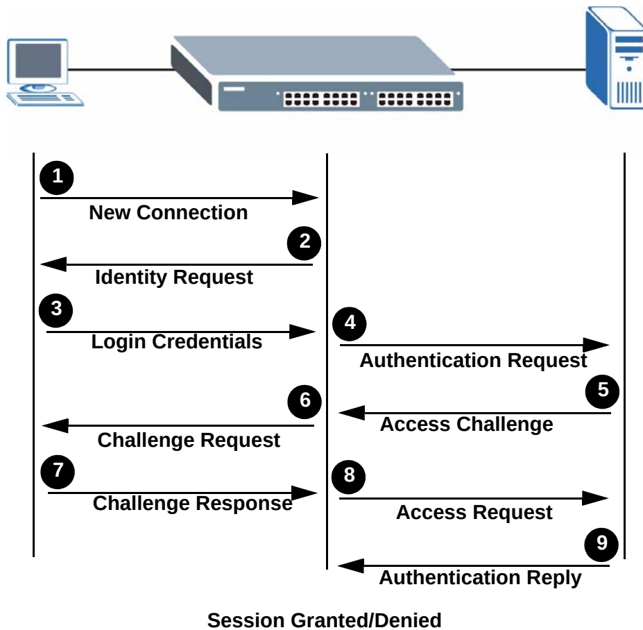
Figure 78 IEEE 802.1x Authentication Process
