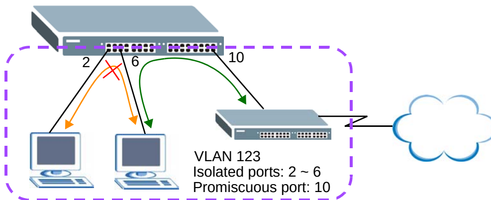
Figure 152 Private VLAN Example
