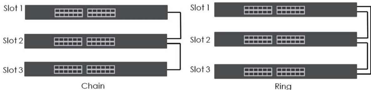
Figure 149 Stacking Topology
