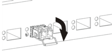
Figure 24 Transceiver Removal Example
