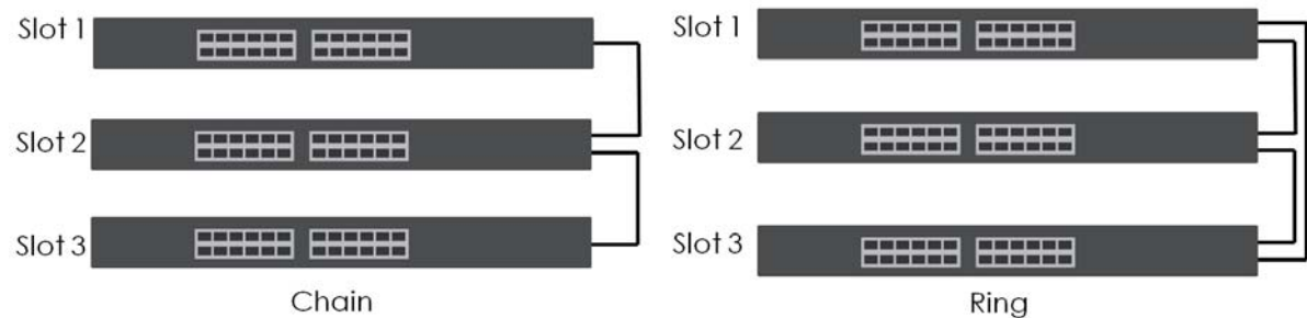
Figure 149 Stacking Topology
