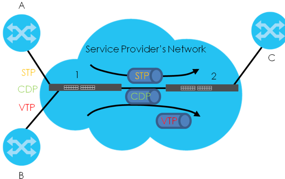
Figure 162 Layer 2 Protocol Tunneling Network Scenario
