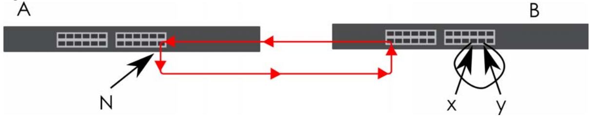
Figure 158 Switch in Loop State
