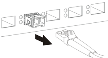
Figure 17 Removing the Fiber Optic Cables
