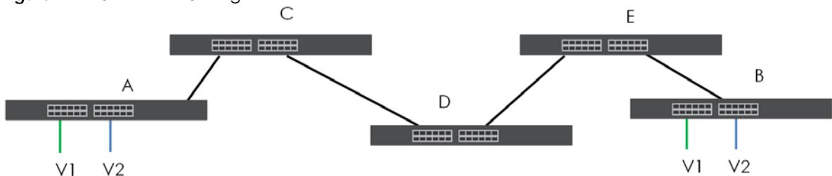
Figure 91 Port VLAN Trunking
