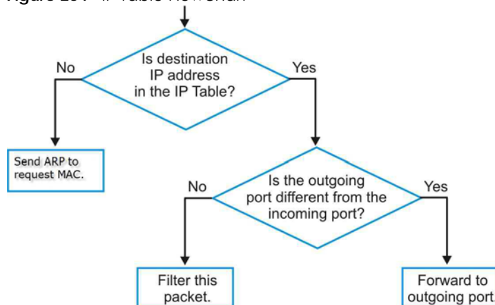
Figure 254 IP Table Flowchart
