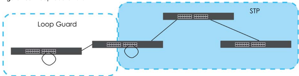
Figure 188 Loop Guard vs. STP
