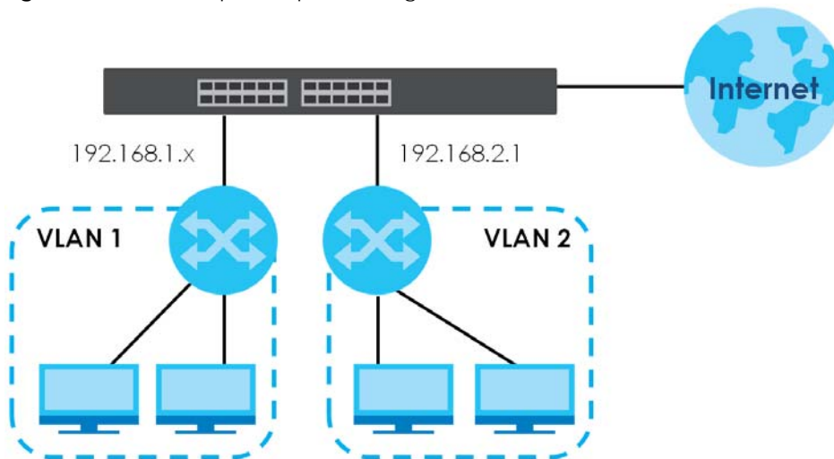
Figure 67 Initial Setup Example: Management IP Address
