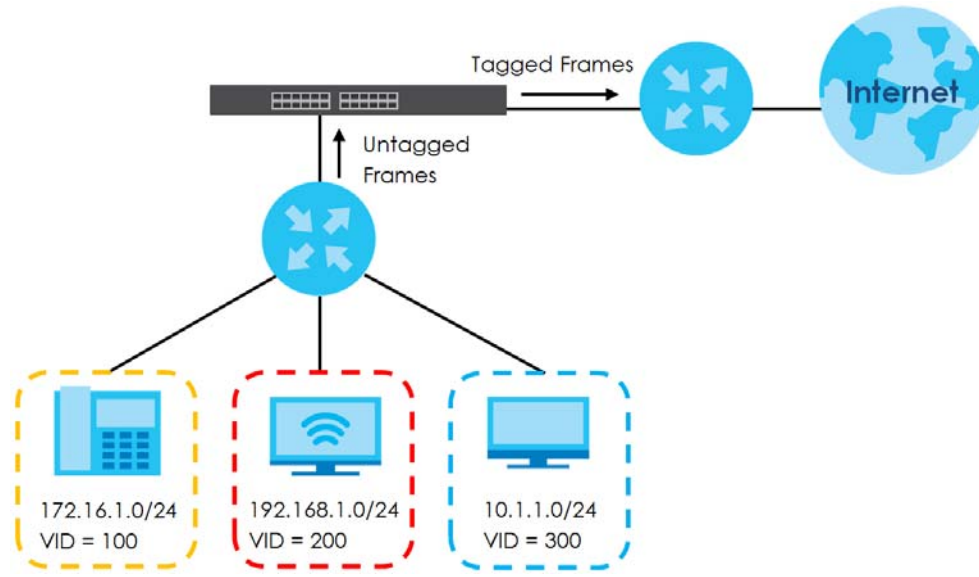
Figure 275 Subnet Based VLAN Application Example
