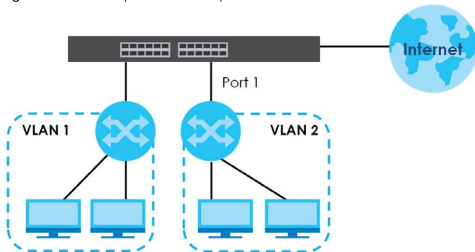
Figure 65 Initial Setup Network Example: VLAN
