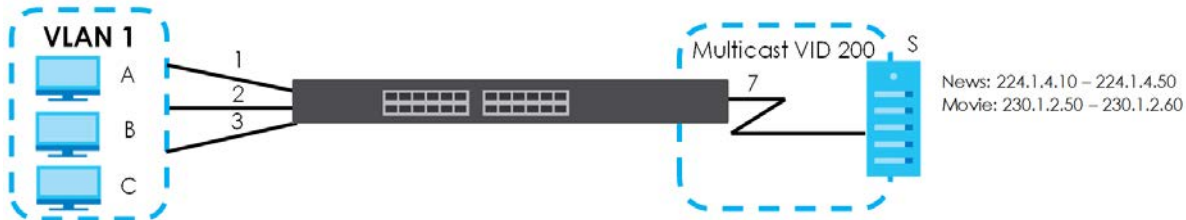
Figure 217 MVR Configuration Example
