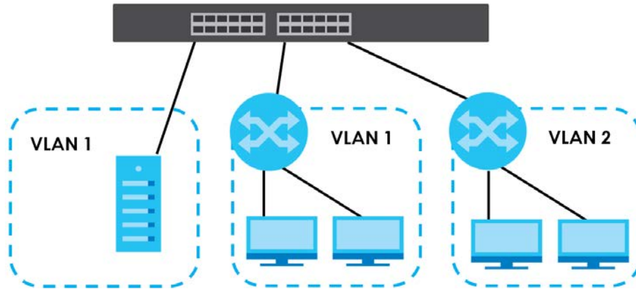
Figure 458 Shared Server Using VLAN Example
