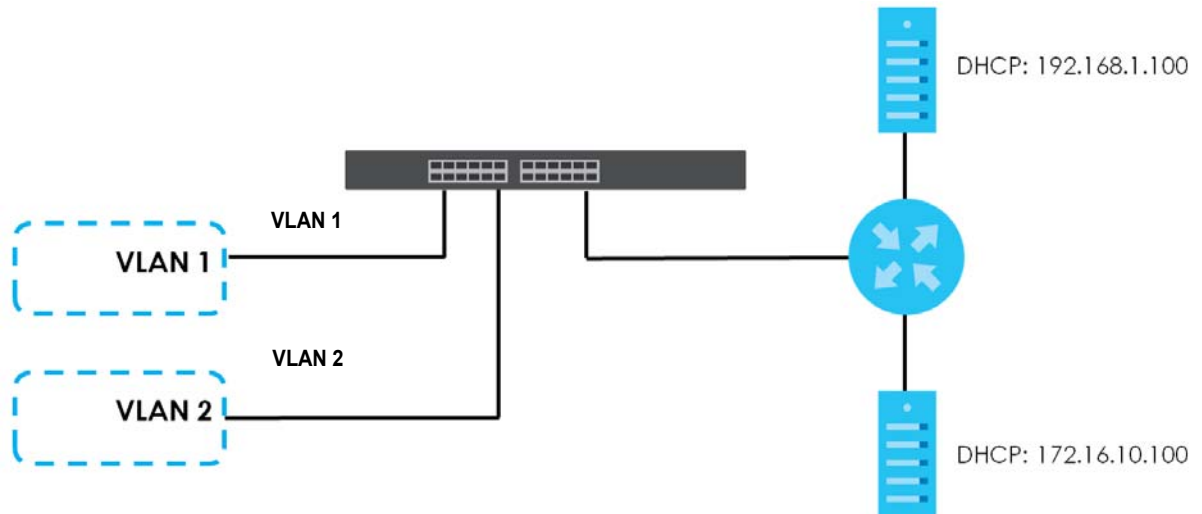
Figure 315 DHCP Relay for Two VLANs
