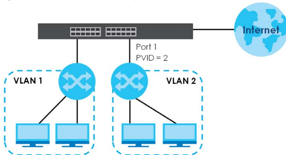
Figure 66 Initial Setup Network Example: Port VID
