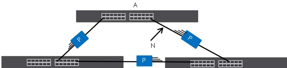
Figure 191 Loop Guard – Network Loop
