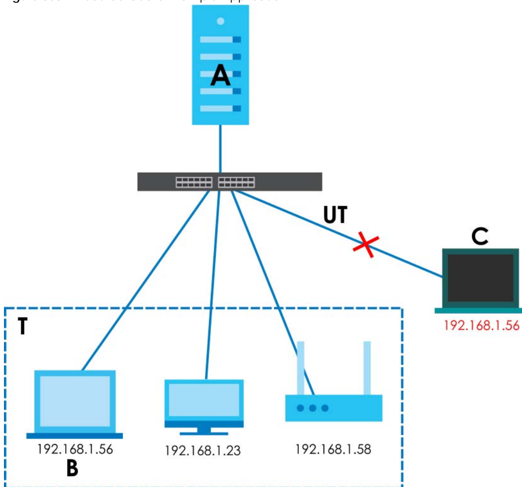
Figure 363 IP Source Guard Example Application
