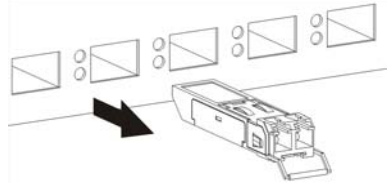
Figure 20 Transceiver Removal Example
